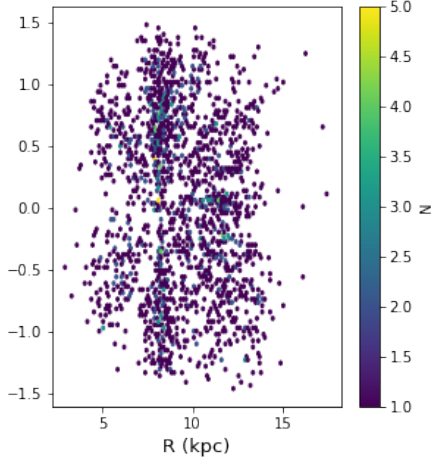
APOGEE DR17
