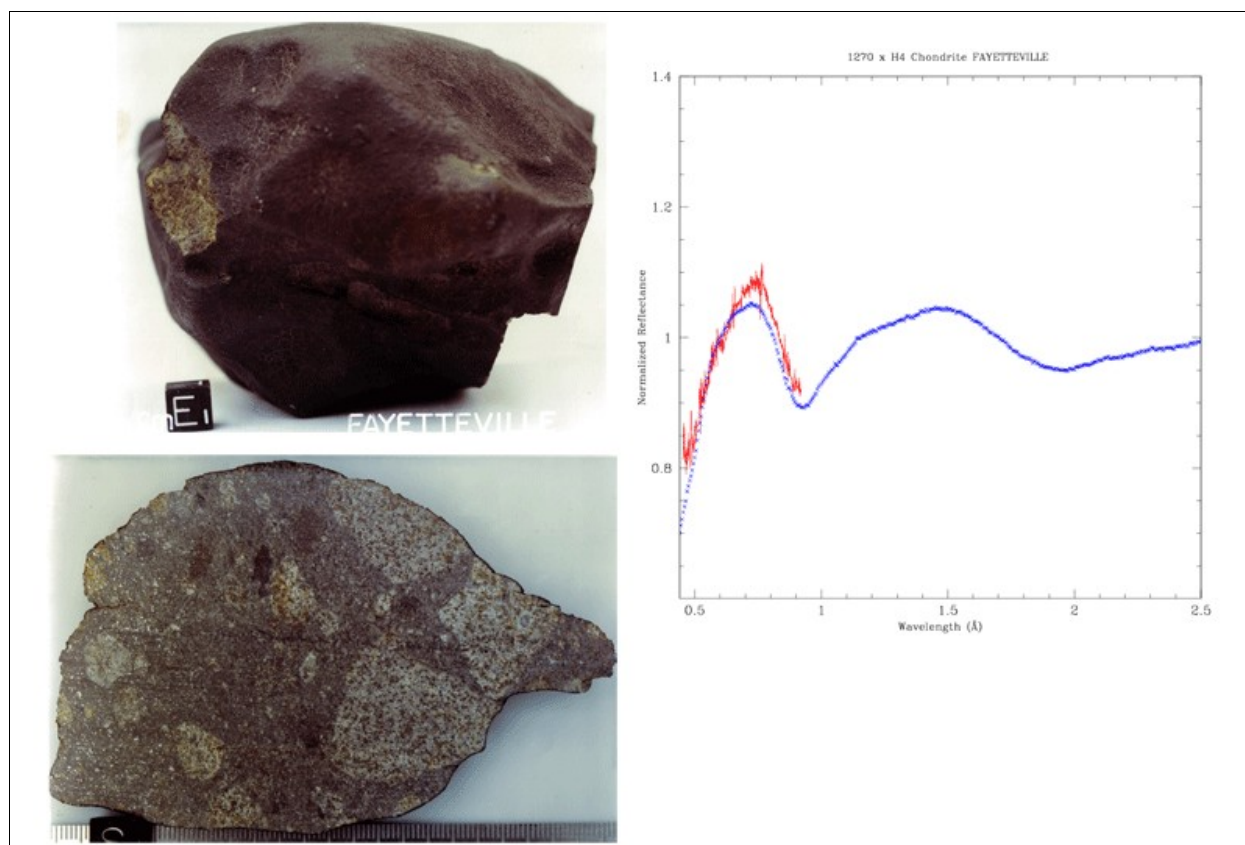
Figure 1. (Right) Comparison of the spectrum of asteroid (1270) Datura with the spectrum of the Fayetteville meteorite. (Left) Pictures of the Fayetteville meteorite (© Arkansas Center for Space and Planetary Sciences, University of Arkansas).
