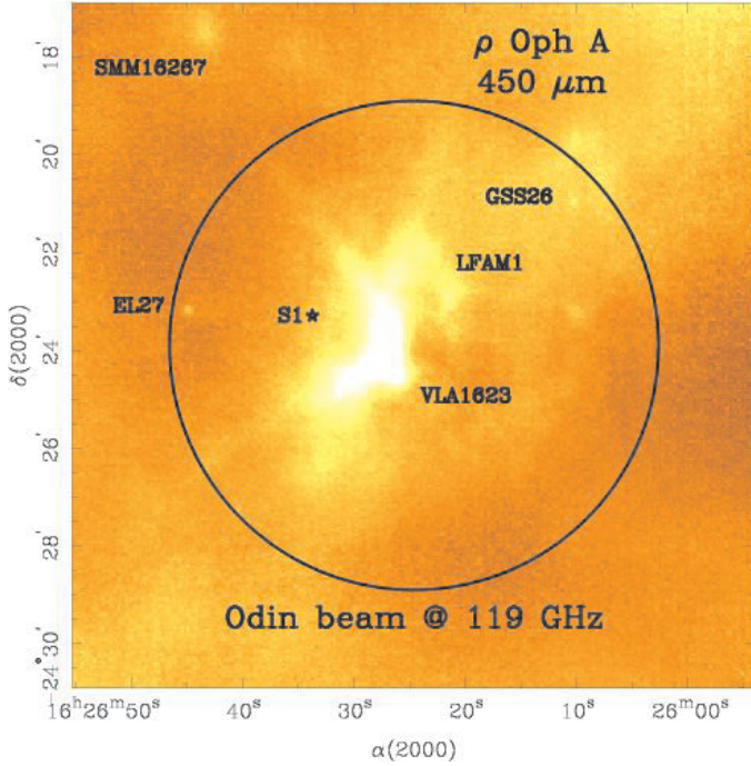
Fig. 1. The 10' Odin beam at 119 GHz, the frequency of O_2(N_J = 1_1-1_0) , is shown as the large circle superposed onto the 450 \mu m map by Hargreaves (2004, see also Wilson et al. 1999). At the distance of 145 pc (de Zeeuw et al. 1999), the beam size corresponds to 0.4 pc. A few discrete sources are labelled. The observations were centered on RA = 16 h 26 m 24 s .6, Dec = -24°23'54" (J2000).
