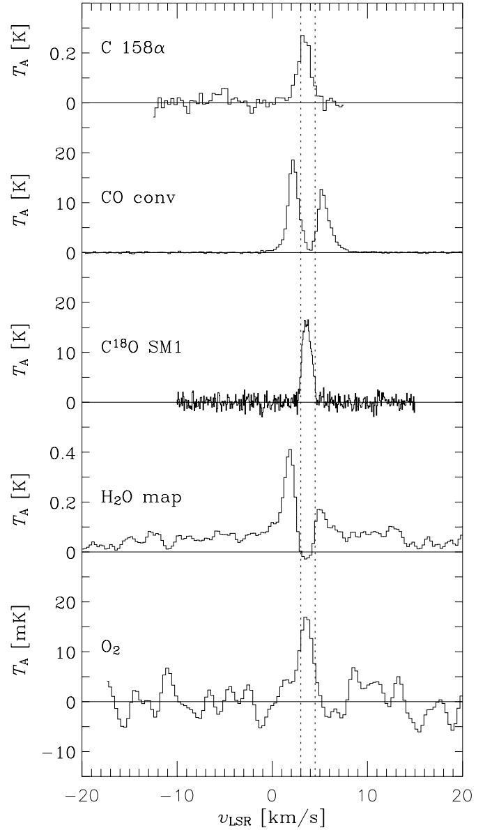
Fig. 2. The Hanning-smoothed O_2 line spectrum is shown in the bottom panel and compared to Odin H_2O(1_{1,0}-1_{0,1}) line data (Larsson et al. 2007), to C^{18}O(3-2) and CO(3-2) from the JCMT-archive, and the C\ 158\alpha recombination line from Pankonin & Walmsley (1978). The H_2O spectrum represents the average of the part of the \rho Oph A cloud mapped with Odin (slightly larger than 5' \times 4' ). The C^{18}O spectrum (15'' beam) refers to a pointed observation toward the Odin center coordinates, while the CO spectrum is that of the 3.5' \times 10' (at PA = 45°) CO(3-2) map convolved with the 10' Odin beam. The displayed spectrum of the C\ 158\alpha recombination line refers to the average of 4 map positions covering about 10' \times 10' . Vertical dotted lines are shown at v_{LSR} = +3.0 km s -1 and +4.5 km s -1 , respectively.
