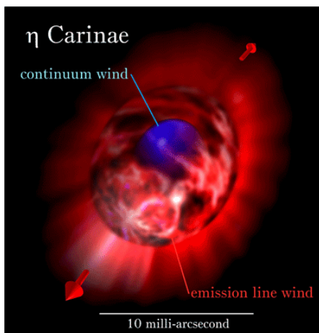
Fig. 2. The aspherical and latitude-dependent stellar wind of \eta Carinae. The artist's impression visualizes the inner regions of \eta Carinae probed with AMBER at different wavelengths. The dense stellar wind (blue) totally obscures the central star and the direction of the outflowing wind corresponds to the main axis of the Homunculus nebulae at larger scale.
