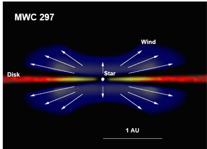
Fig. 1. A new picture of this system from AMBER observations of the young stellar object MWC 297. MWC 297 is surrounded by an equatorial optically-thick disc that is possibly still accreting, and an outflowing wind is located just above it.
