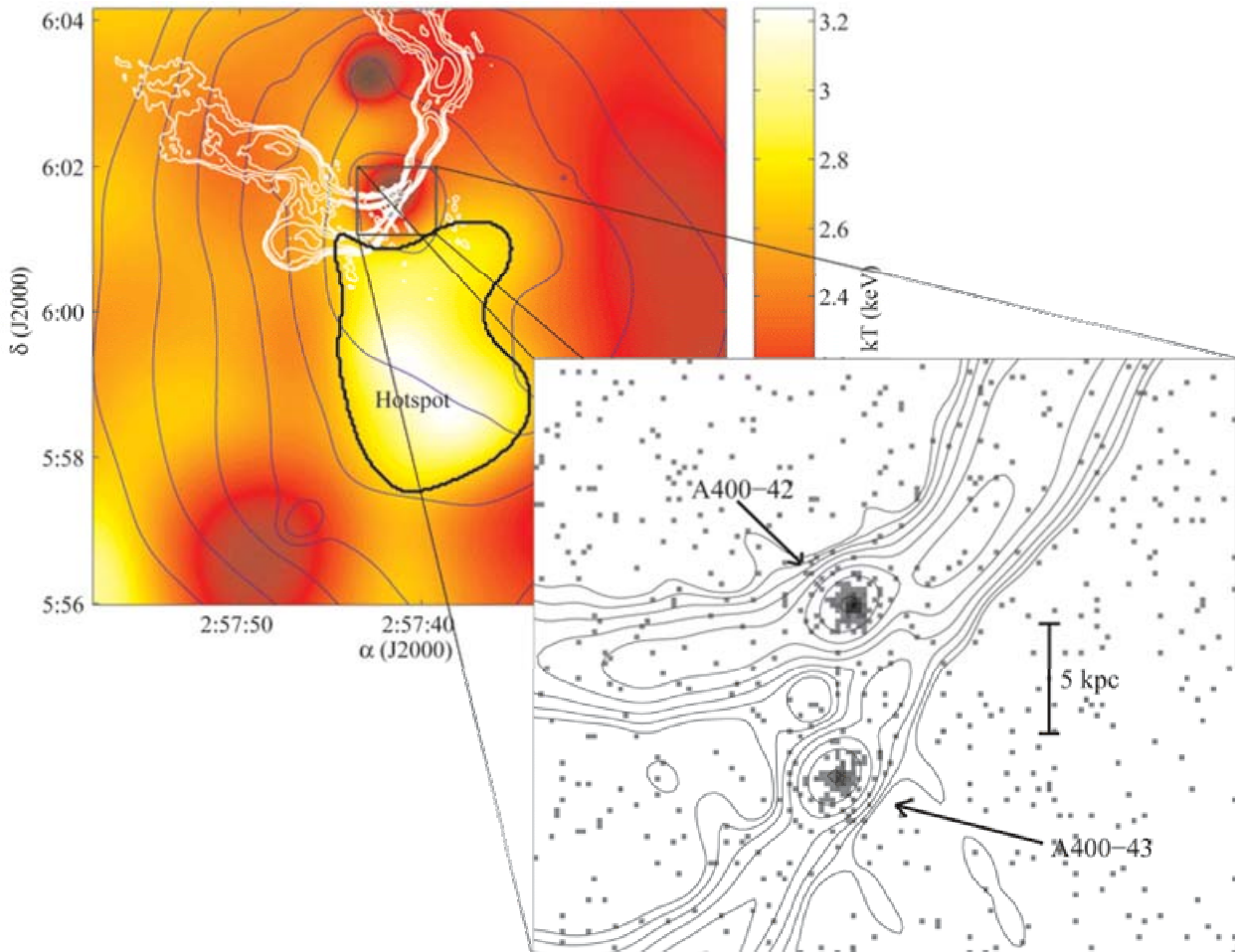
Fig. 1. This image shows the central region of the galaxy cluster Abell 400. The colour coding gives the temperature of the X-ray emitting gas trapped in the cluster: black-cold (18 million degrees Celsius) to white-hot (38 million degrees Celsius). The contours show the radio emission from the jets of plasma being expelled by the black holes. As the two black holes stream through the gas at supersonic velocities, the jets are bent toward the top of the image. The gas in front of the black holes is compressed and heated, as seen by the hotspot below them. The inset shows a blow up of the central regions. Each dot represents a position where an X-ray photon has struck Chandra's X-ray camera. The two black holes are seen as bright regions where as many as 250 X-ray photons struck the camera. The contours again show the radio emission from the black holes and the jets of plasma being ejected from them.
