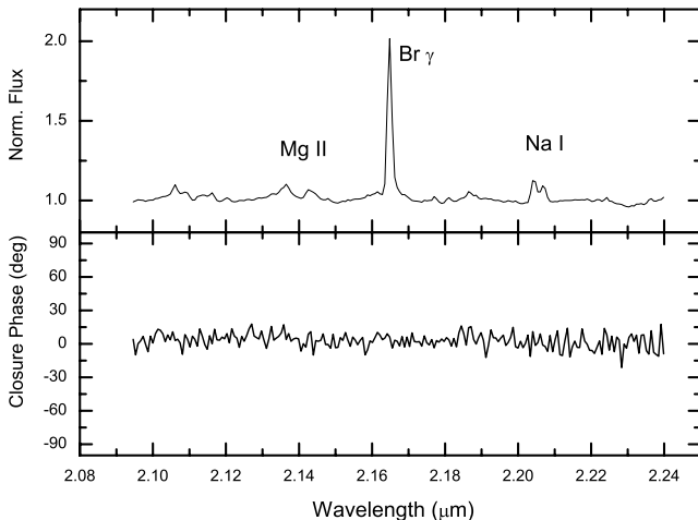
Fig. 4. VLTI/AMBER closure phase for CPD-57° 2874 obtained around Bry with spectral resolution R = 1500 . Within the noise level ( \approx \pm 10^\circ ) the closure phase is zero both in the continuum and in the Bry line. This strongly suggests that the CSE has an approximately centrally-symmetric projected intensity distribution in the near-IR.
