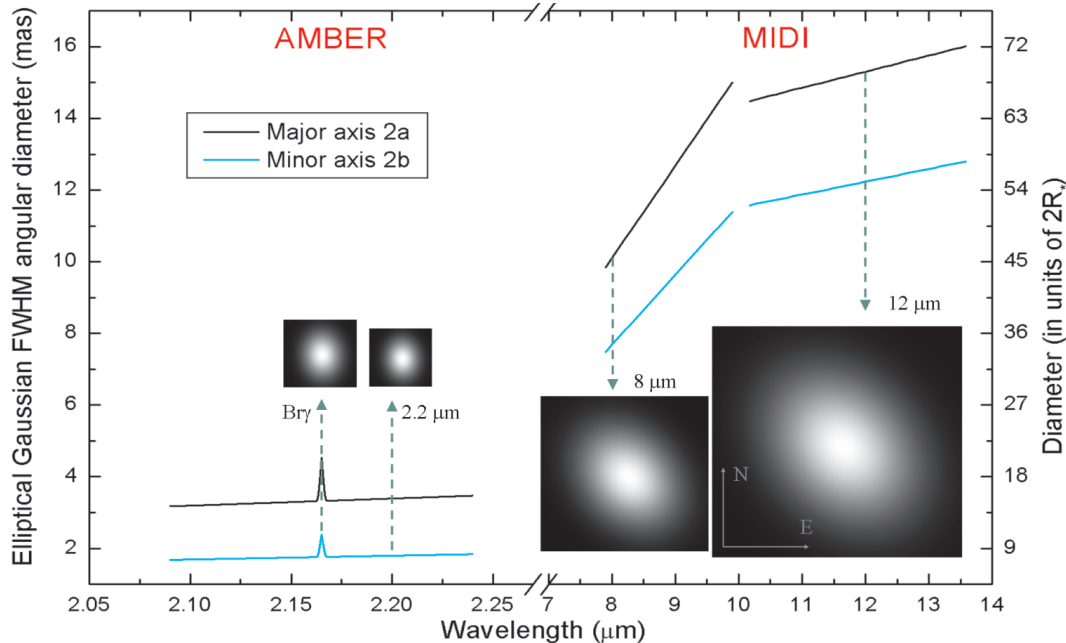
Fig. 5. Size and orientation of the CSE derived from the fit of an elliptical Gaussian model (Eqs. (1) and (2)) to the VLT/AMBER and VLT/MIDI visibilities (the corresponding fit parameters are listed in Table 4). The scale in the right is given in stellar diameters ( 2R_* ), where the radius R_* is estimated to be 60 \pm 15 R_\odot (Sect. 3).
