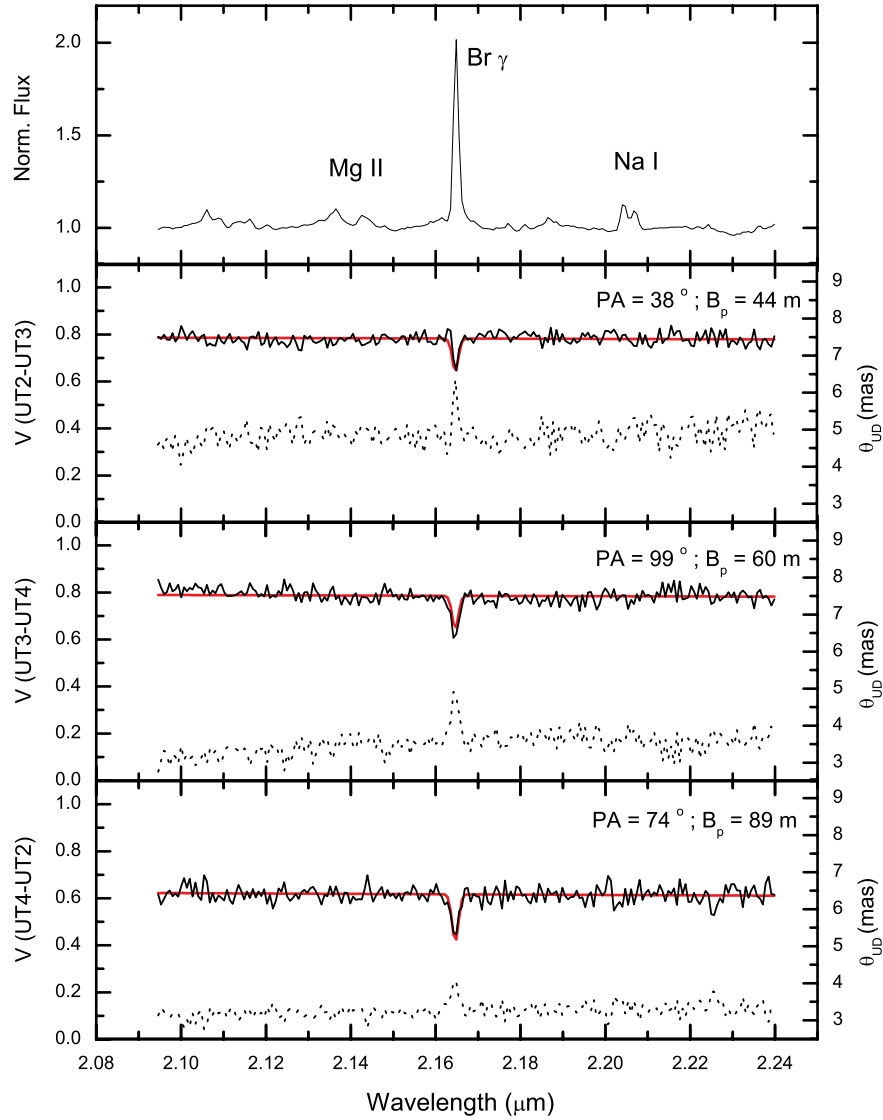
Fig. 2. VLT/AMBER observations of CPD–57° 2874 obtained around Br \gamma with spectral resolution R = 1500 . The normalized flux is shown in the top panel and the visibilities V for each baseline (30% best frames) are given in the other panels (the corresponding projected baselines B_p and position angles PA are indicated). The errors in V are \approx \pm 5\% . The dotted lines are the uniform disk angular diameters \theta_{UD} (to be read from the scales on the right axis), computed from V at each \lambda as a zero-order size estimate. The visibilities obtained from the elliptical Gaussian model fit the observations quite well (smooth solid lines; Eqs. (1) and (2), and Table 4). In contrast to the Br \gamma line, the Mg II and Na I lines do not show any clear signature in the visibilities.
