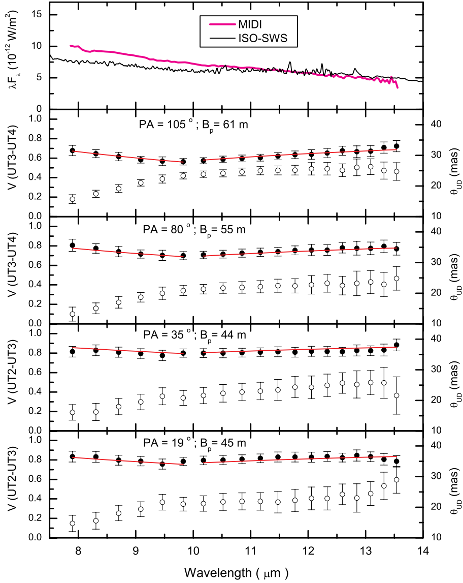
Fig. 3. VLT/MIDI observations of CPD-57° 2874 obtained in the mid-IR with spectral resolution R = 30 . This figure is organized as Fig. 2, but here V and \theta_{UD} are shown as filled and open circles, respectively. The MIDI and ISO-SWS (Sloan et al. 2003) spectra ( top panel ) do not show any clear evidence of a silicate feature around 10\mu\text{m} . The MIDI visibilities are well fitted with an elliptical Gaussian model (solid lines; Eqs. (1) and (2), and Table 4).
