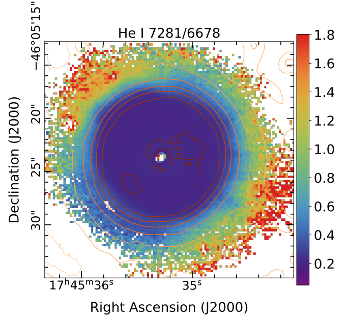
Fig. 9. Image of the Tc 1 core region for the ratio of the fluxes of the \text{He I} 7281 and 6678 \text{\AA} lines. Spaxel values above 0.31 are outside the feasible range of the \text{He I} ratio, indicating a possible contaminating line in the region outside of the bright core. The contours are for the H\beta flux.
