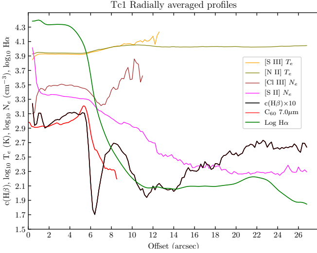
Fig. 7. Radial variation of the CEL diagnostics with the offset from the position of the CSt for T_e and N_e , which are both plotted as \log_{10} . For comparison the radial variation for c(H\beta) , scaled by a factor 10 to be similar in values to \log_{10} T_e and N_e , and the scaled \log_{10} H\alpha surface brightness, are also shown. The low c annulus occurs between radii 6–7". Also plotted (in red) is the \log_{10} surface brightness profile of the C_{60} 7.0 \mu\text{m} band ( \text{erg cm}^{-2} \text{s}^{-1} \times \text{an arbitrary constant} ) for comparison (c.f. Giese et al., in prep.). The C_{60} profile was however determined over a limited angular extent of 40".
