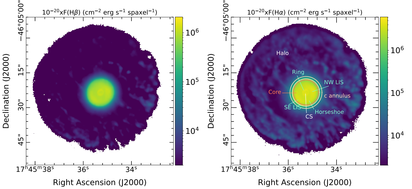
Fig. 1. Morphology of Tc 1 in H Balmer emission.
