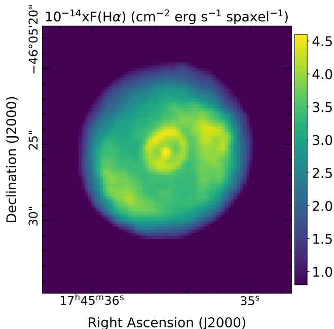
Fig. 10. Expanded image of the core region of Tc 1 in H \alpha surface brightness ( 10^{-14} erg cm ^{-2} s ^{-1} spaxel ^{-1} ).
