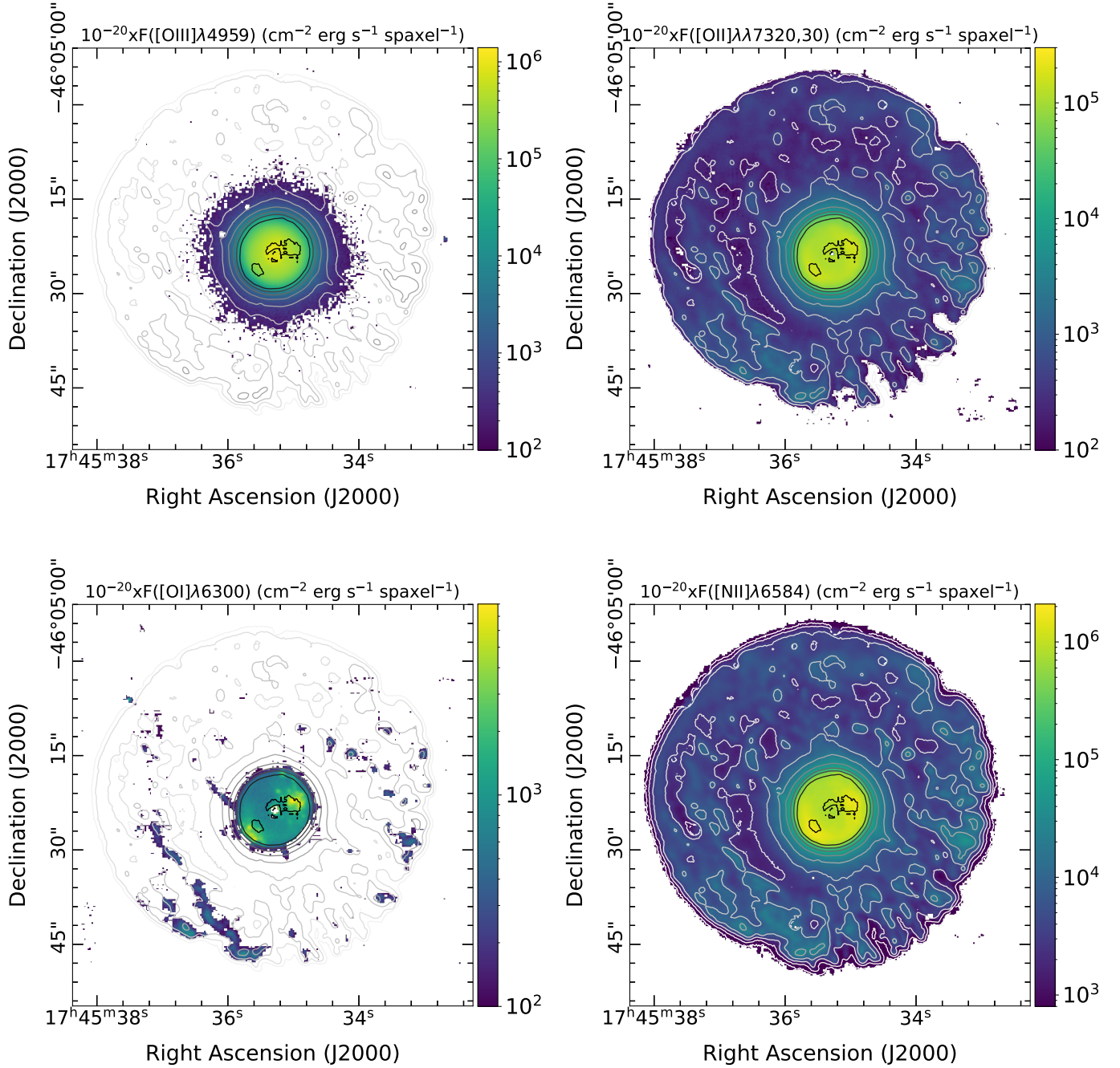
Fig. 2. Morphology of Tc 1 in some CELs.
