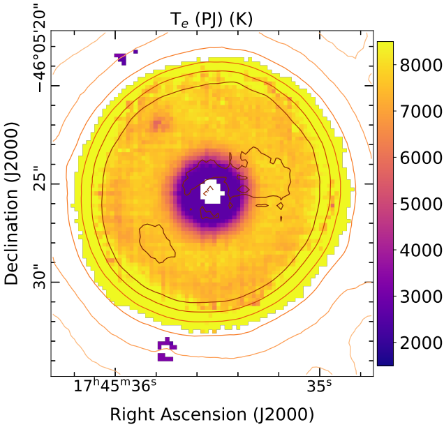
Fig. 8. Map of T_e for the core region only, derived from the Paschen continuum jump at 8250 \text{\AA} ratioed by the dereddened H\text{I} Paschen 11 (8862.8 \text{\AA} ) emission line strength. Initial estimates of T_e and N_e from the CEL diagnostic ratios (Sect. 4.2.1) for calculation of the dependence of PJ/P11 on T_e were employed. The contours are from the H\beta image (Figure 1) and the cut-off is at S/N of 3 per 0.2" spaxel.
