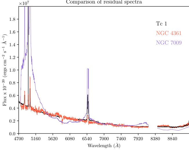
Fig. D.1. Comparison of the residual spectra (i.e. dereddened spectrum of the total nebular flux collected in the MUSE observations – the fitted nebular continuum, as calculated from the parameters in Table D.1), is shown between Tc 1, NGC 4361 (Walsh et al. (2024) and NGC 7009 (Walsh et al. 2018). All spectra have been cleaned of narrow emission lines and sky subtraction residuals and normalized to the same flux at 7000 Å. See text for further details.
