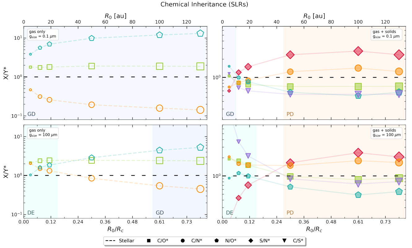
Fig. B.1: Same as Fig. 2 but showing planetary elemental ratios in the low-ionisation inheritance scenario.
