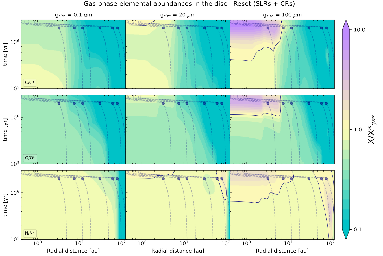
Fig. A.2: Same as Fig. A.1 but showing elemental abundances in the high-ionisation reset scenario.
