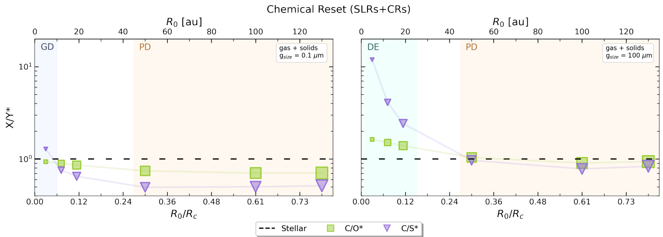
Fig. 4: Same as Fig. 2 but showing only the C/O* (green) and C/S* (purple) ratios in solid-enriched atmospheres, for a more direct comparison of elemental ratios when nitrogen-bearing species are not measurable. This subset highlights the characteristic chemical signatures that can still be identified when only C-, O-, and S-bearing species are available for atmospheric characterisation.
