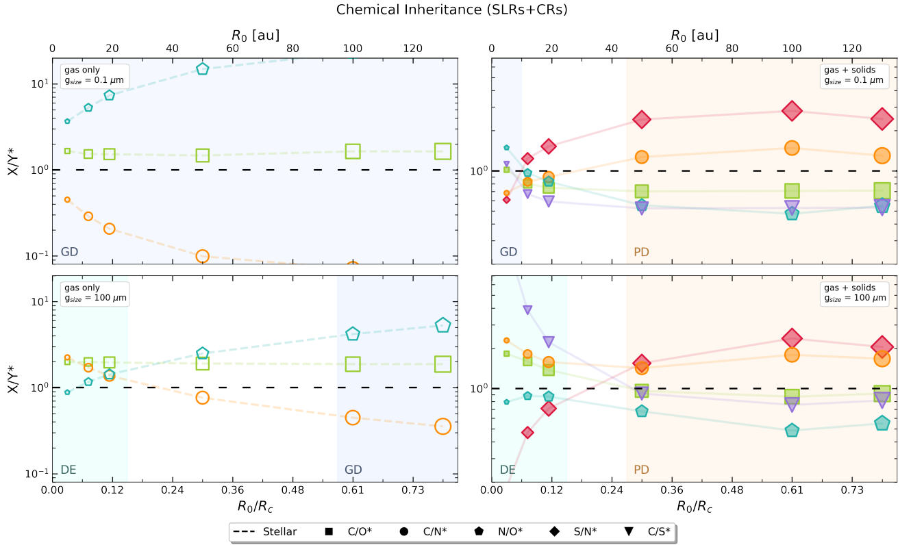
Fig. B.2: Same as Fig. 2 but showing planetary elemental ratios in the high-ionisation inheritance scenario.
