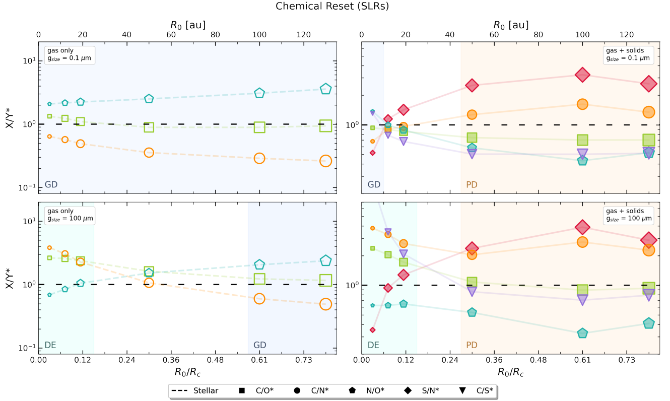
Fig. B.3: Same as Fig. 2 but showing planetary elemental ratios in the low-ionisation reset scenario.
