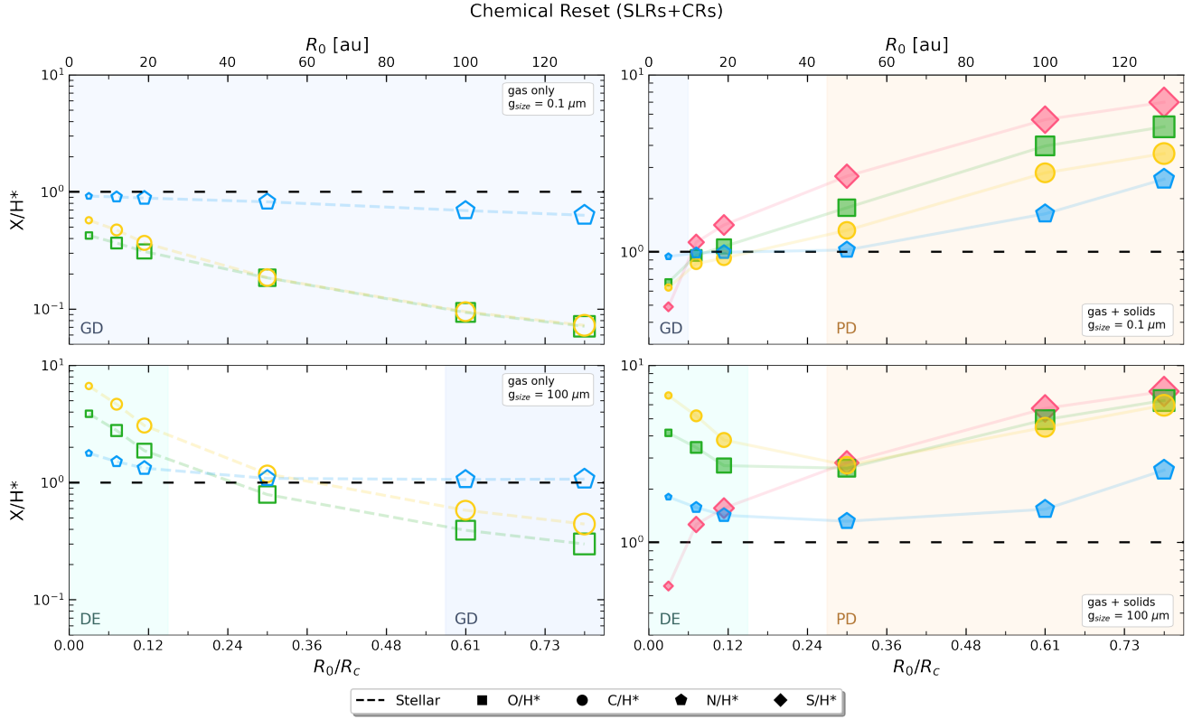
Fig. C.1: Same as Fig. 2 but showing elemental abundances in the primordial atmospheres of the six simulated giant planets as a function of their initial orbital positions. All abundances are normalised to their respective stellar value; the horizontal dashed line at 1 marks the stellar reference in all plots.
