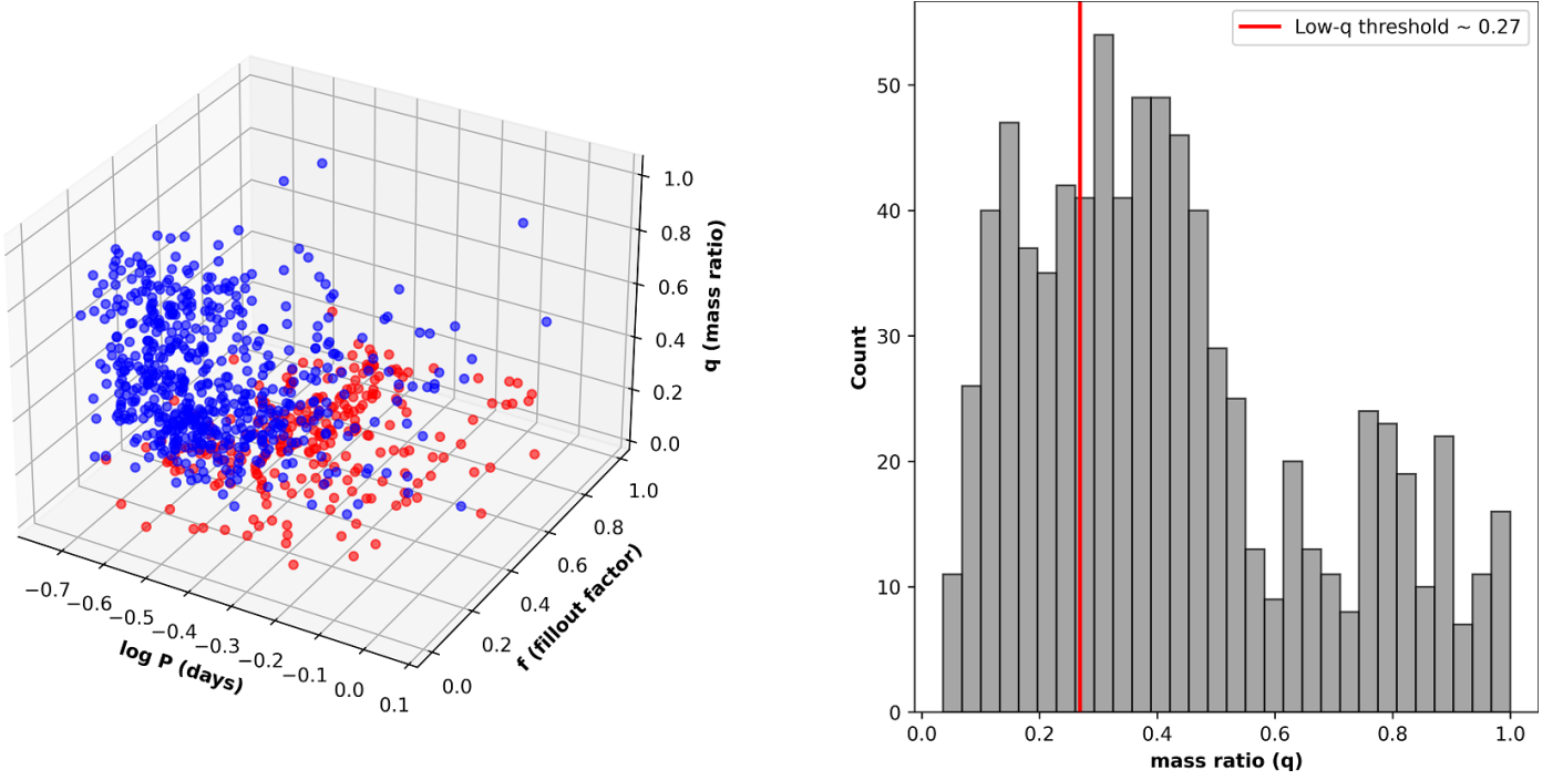
Fig. 3: Left: 3D scatter plot of \log P , f , and q for the contact binary sample. Systems with q \leq 0.27 are highlighted in red. Right: Histogram of q . The vertical red line marks the low mass-ratio threshold.
