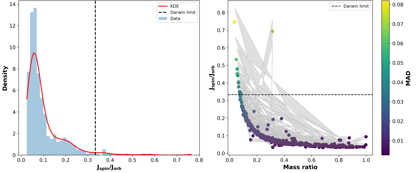
Fig. 4: a) Histogram of J_{\text{spin}}/J_{\text{orb}} with a KDE overlay. The vertical line indicates the classical Darwin limit (0.333). b) Two-dimensional scatter plot of the mass ratio vs. J_{\text{spin}}/J_{\text{orb}} , with uncertainty bands represented by the MAD of the MC realizations.
