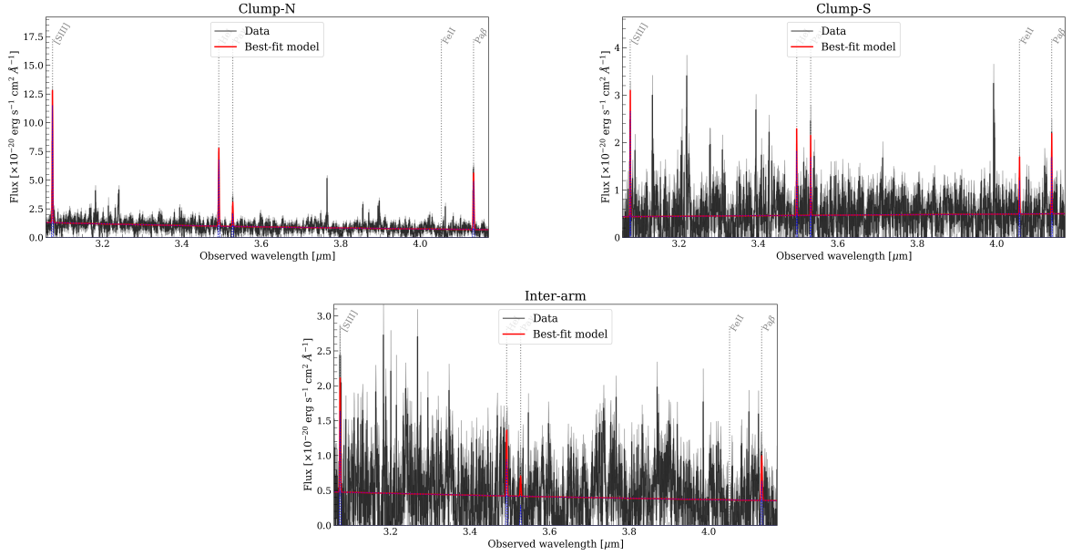
Fig. A.6. NIRSpec MSA high-resolution spectra ( R=2700 ) of K20-ID7, obtained with the G395H/F290LP, for the shutters where we detect emission lines at S/N>3 . Data are shown in black, with the best-fit model overplotted in red.
