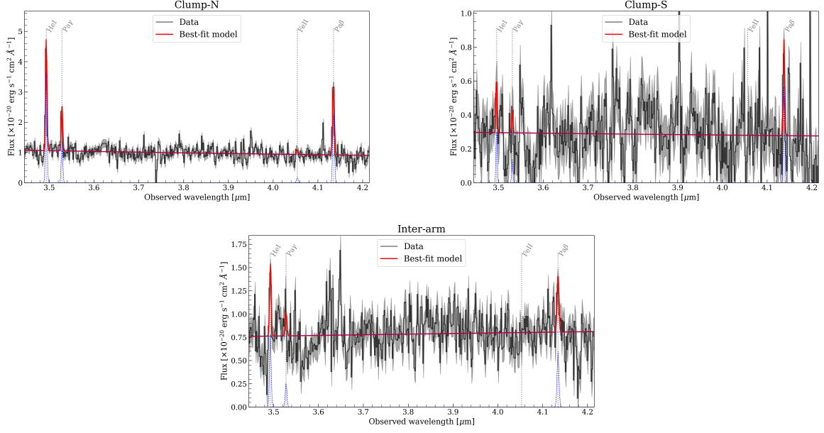
Fig. A.5. NIRSpec MSA high-resolution spectra ( R=1000 ) of K20-ID7, obtained with the G395M/F290LP, for the shutters where we detect emission lines at S/N>3 . Data are shown in black, with the best-fit model overplotted in red.
