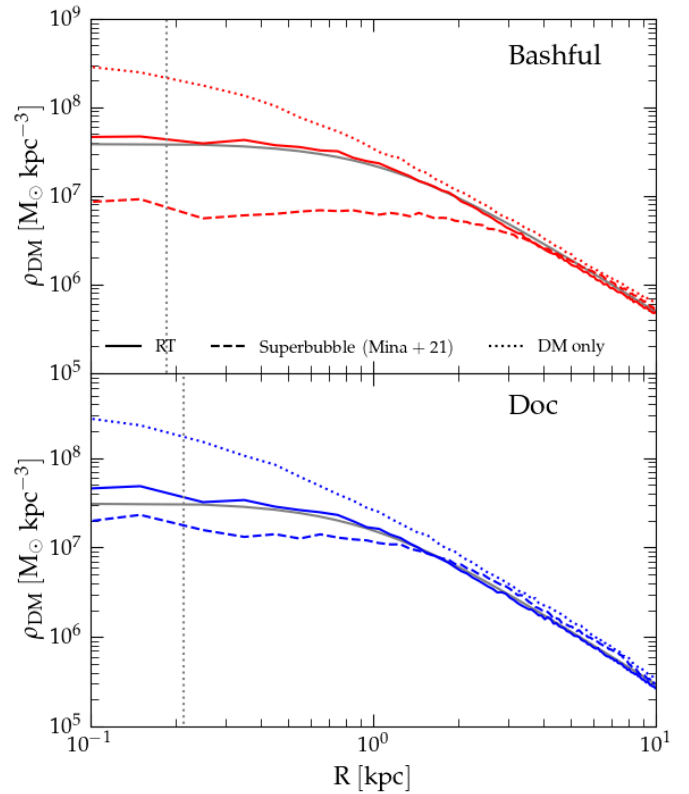
Fig. 9. Present-day DM density profile for the two most massive dwarf galaxies in the simulation, Bashful (top) and Doc (bottom). The solid lines represent the RT run, the dashed lines correspond to the Superbubble run (Mina et al. 2021), and the dotted line is the DM-only comparison run. The gray line shows the best-fitting pseudo-isothermal DM profile. The vertical dashed lines indicate the radii below which numerical convergence can not be reached to due two-body relaxation (Power et al. 2003).
