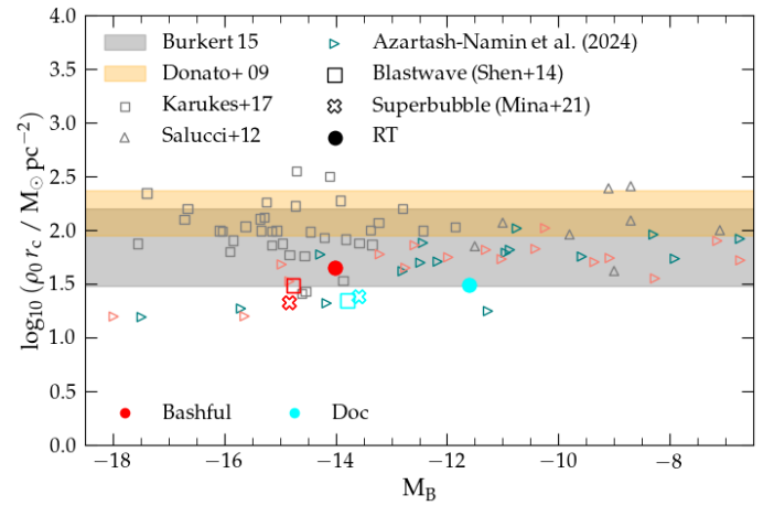
Fig. 12. Dark Matter core surface density ( \rho_0 r_c ) as a function of B-band magnitude of Bashful and Doc compared to disc dwarf galaxies (Karukes & Salucci 2017, gray squares), Milky Way dSphs (Salucci et al. 2012, gray triangles), the scaling relations from Donato et al. (2009, yellow shaded region), Burkert (2015, gray shaded region) and simulation data from Azartash-Namin et al. (2024) (teal and light red triangles for their blastwave and superbubble feedback simulations, respectively).
