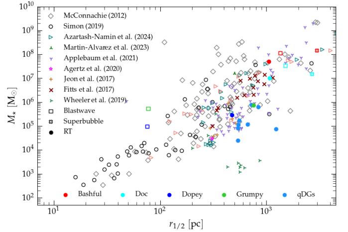
Fig. 5. Stellar mass versus half-light radius of the simulated dwarf galaxies, compared to observations from McConnachie (2012) and Simon (2019); simulations from Jeon et al. (2017); Fitts et al. (2017); Wheeler et al. (2019); Applebaum et al. (2021); Azartash-Namin et al. (2024); and RT simulations from Agertz et al. (2020) and Martin-Alvarez et al. (2023). For the Azartash-Namin et al. (2024) data points, the teal and light red colours correspond to their Blastwave and Superbubble run, respectively.
