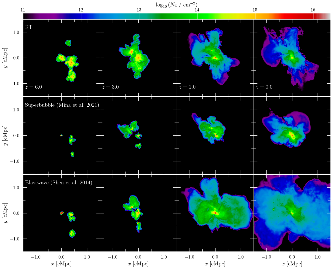
Fig. 13. Metal distribution through cosmic time from z=6 to z=0 for the RT (top), Superbubble (middle), and Blastwave (bottom) runs. Metals in the RT run are distributed over a greater area, as stars are formed in a greater number of small progenitor halos.
