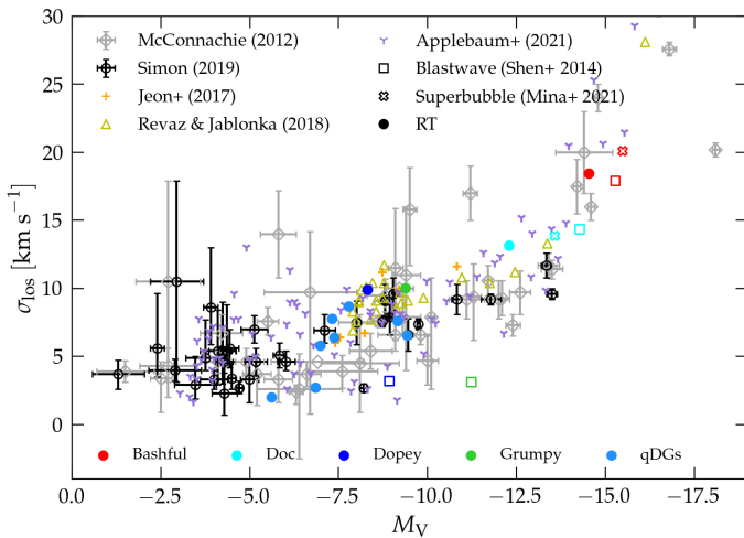
Fig. 6. Luminosity-velocity dispersion ( M_V - \sigma_{\text{los}} ) relation of the simulated dwarf galaxies compared to observations from McConnachie (2012) and Simon (2019) and simulations from Jeon et al. (2017) , Revaz & Jablonka (2018) and Applebaum et al. (2021) . Solid circles show the results of the new RT run, colour-coded as indicated; open squares and crosses correspond to the Blastwave and Superbubble runs.
