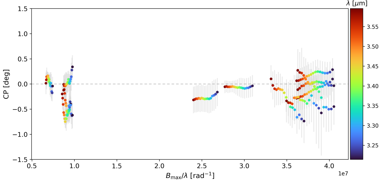
Fig. B.1. L -band interferometric CPs as a function of the spatial frequency of the longest baseline in the triangle.
