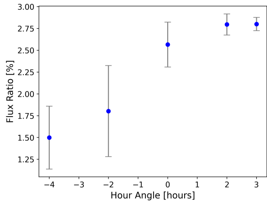
Fig. 6. Example of retrieved flux ratios from a synthetic 2D Gaussian model, assuming over-resolved emission. Variations due to different uv -plane samplings could mimic temporal variability.
