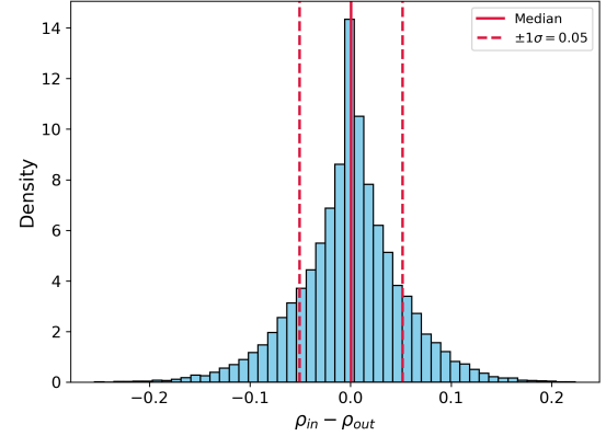
Fig. D.2. Distribution of the difference between the retrieved and true values for a correlation in visibility space across noise iterations and correlation values.
