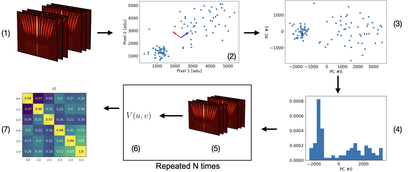
Fig. 2. Diagram of the process (Sect. 3.2) for generating visibilities used in the calculation of the correlation matrix: (1) intermediate observational frames; (2) pixel–pixel scatter plot of values with arrows showing the two PCs; (3) data of these two pixels transformed into the PC basis; (4) histogram of the values along one PC; (5) distribution used for generating synthetic frames; (6) visibilities extracted from these frames; (7) covariance matrix computed from the synthetic visibilities. Steps (5) and (6) were repeated to properly sample the visibility distribution.
