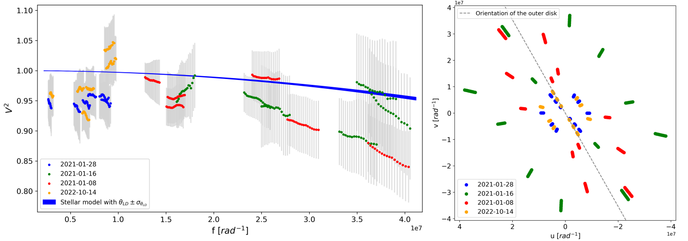
Fig. 1. Left panel: L -band interferometric squared fringe visibilities ( V^2 ) as a function of spatial frequency ( B/\lambda , where B is the projected baseline) for all the MATISSE observations in Table B.1. The blue-shaded area represents stellar squared visibility for the \beta Pictoris stellar model with a 1\sigma uncertainty on the angular diameter \theta_{LD} (see Table A.1). Right panel: uv plane coverage of all the observations. The dashed line represents the orientation of the major axis of the outer disk on the sky (PA=29.6°; see Table A.1).
