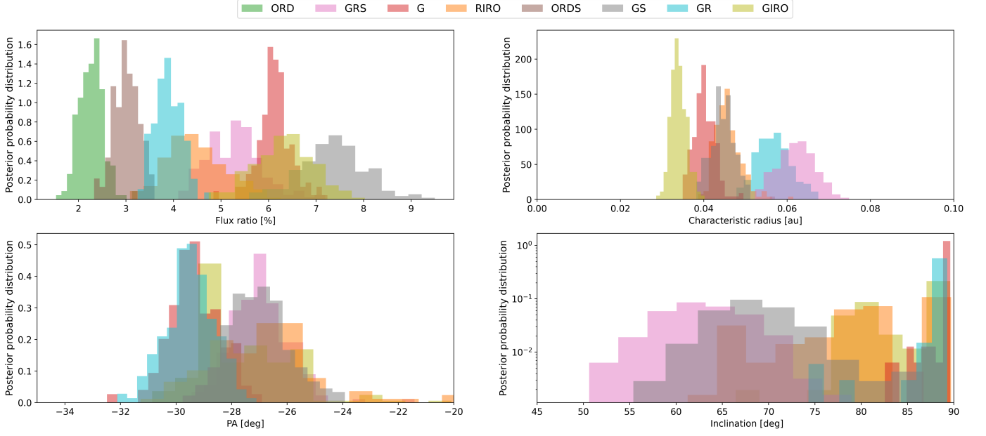
Fig. H.3. Posterior distributions for all single-component models and the inner component of two-component models, obtained when accounting for correlations. The distribution of inclinations (bottom right) is presented in log scale, because some (e.g., GRS and GS) are broader than others (e.g., G), while the other distributions are shown in linear scale.
