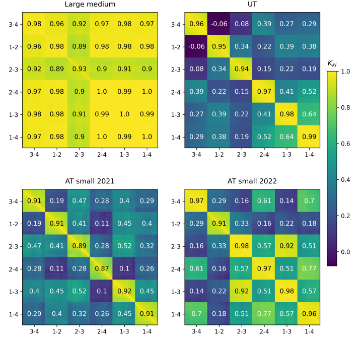
Fig. 3. Correlation matrices of the V^2 measurements for the four MATISSE L -band datasets (see Table B.1). Each pixel in the images represents a data point for the baseline and wavelength pairs. The values on the image represent the average correlation across all spectral channels for a given baseline pair.
