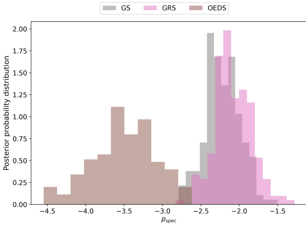
Fig. H.2. Spectral index of the flux ratio.
