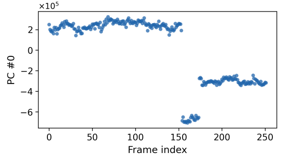
Fig. D.1. Example data distribution along the first PC (here for the BCD position IN-IN), showing a strong multimodal behavior.
