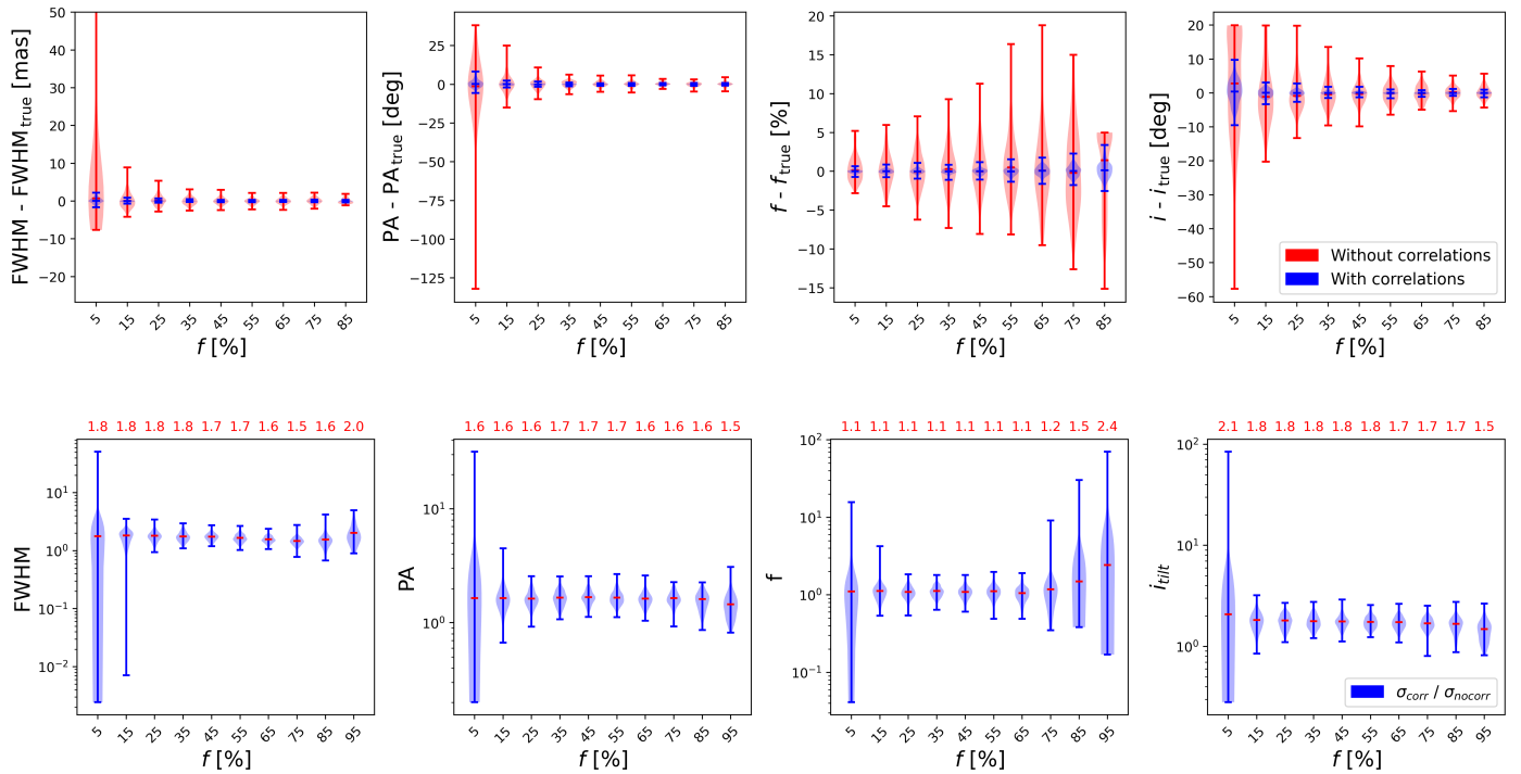
Fig. 7. Top: Distribution of the difference between the retrieved values and the input value for four parameters (FWHM, PA, flux ratio, and inclination). The red distributions were obtained under the assumption of independent errors, while the blue distributions account for correlations. These distributions are shown in the form of violin plots with increasing flux ratios on the horizontal axis. In each case, the vertical markers indicate the minimum, median, and maximum values. Bottom: Distribution of the ratios between the errors when accounting for correlations and errors when ignoring correlations. The median value is shown by the red text at the top of each violin plot.
