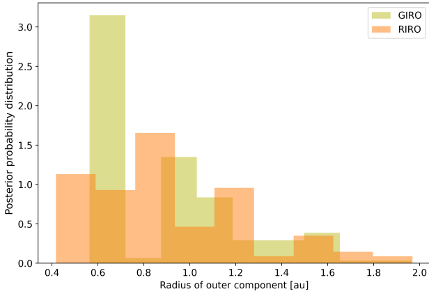
Fig. H.1. Half-light radius of the outer component of the two-component models.
