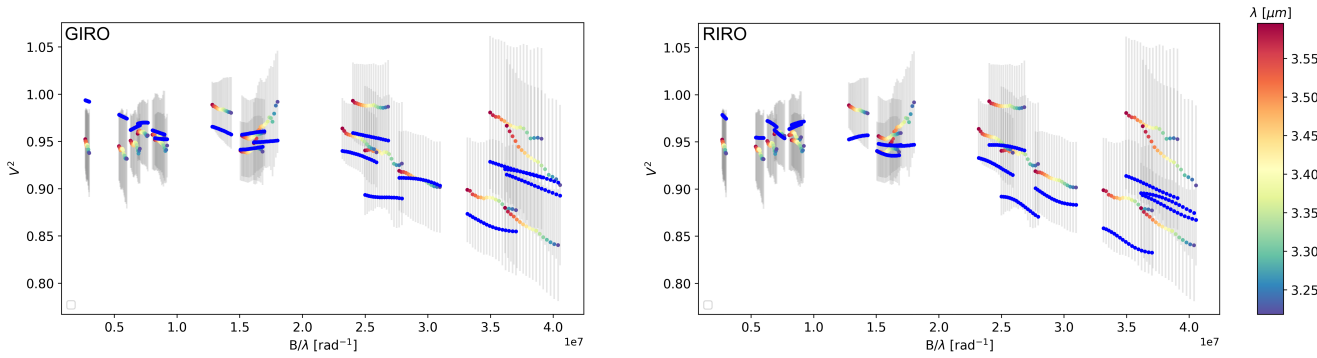
Fig. I.2. Best fits for the two-component models. The model keyword is indicated at the top left of the figure.
