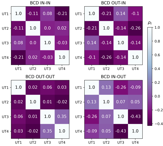
Fig. C.1. Correlation coefficients ( \rho_t ) between telescopes for the photometry of the UT dataset on the science target ( \beta Pictoris) at each BCD position.
