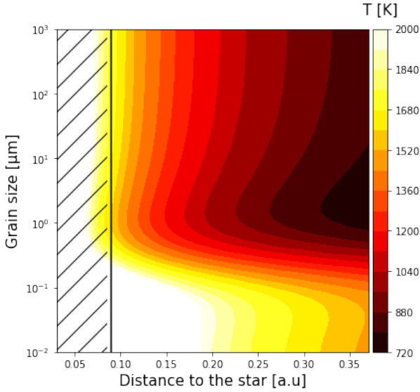
Fig. 4. Temperature of carbonaceous dust grains as a function of their size and distance to the star, assuming hard spheres. The white region marks the sublimation zone ( T > 2000 K), while the shaded area indicates the possible location of the half-flux radius of the emission detected with MATISSE.
