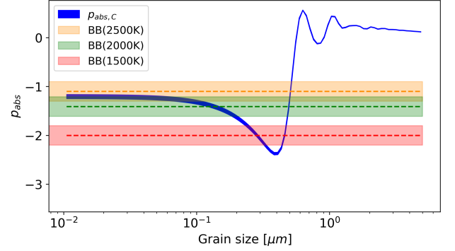
Fig. 5. Power-law exponent ( p_{\text{abs}} ) of the absorption efficiency, with corresponding 1\sigma error, for carbonaceous grains between \lambda = 3.2 and 3.6 \mu\text{m} as a function of grain size. Measured values (GS model; Sect. 4.4) assuming three BB temperatures are shown, with shaded areas indicating 1\sigma uncertainties.
