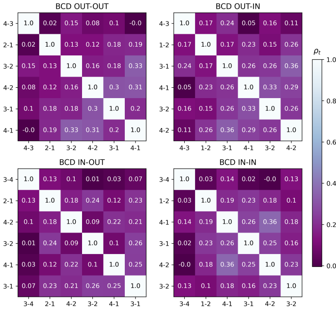
Fig. C.2. Correlation coefficients ( \rho_t ) between baselines for |I(u, \lambda, t)| of the AT Large Medium dataset on the science target, for each BCD position. The numbers represent the telescope indices (e.g., the baseline formed by AT3 and AT2 is labeled 3-2).
