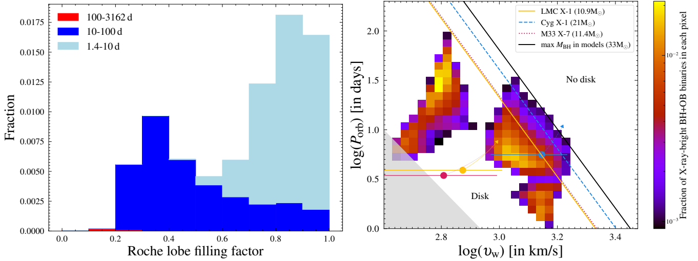
Fig. 3. Observable properties of X-ray-bright systems. Left panel: Distribution of the Roche lobe filling factor of BH+OB star binaries where an accretion disc can form (Sect. 3.2). Light blue, dark blue, and red colours denote the contributions from binary models with different initial orbital period ranges of 1.4–10 d, 10–100 d, and 100–3162 d, respectively. The coloured histograms are stacked on each other, and the sum of their ordinate values is equal to 0.0785 (the fraction of X-ray-bright systems predicted from our entire population of BH+OB star binaries). Right panel: Disc-formation thresholds (Eq. (10) of Sen et al. 2021) shown by slanted solid, dashed, and dotted lines for three BH masses corresponding to the three observed wind-fed BH HMXBs (Orosz et al. 2007, 2009; Miller-Jones et al. 2021; Ramachandran et al. 2022). The black slanted line shows the disc-formation threshold of the maximum BH mass from our binary model grid. An accretion disc can form below the slanted lines and vice versa. The three circles correspond to the observed orbital period and calculated OB star wind speed at the position of the BH (assuming a \beta -law for the wind velocity profile, with \beta = 1 , Eq. (1) of Sen et al. 2021) of the three BH-hosting wind-fed HMXBs. The horizontal solid lines correspond to the range of wind speed by varying \beta from 0.5 (upper-speed limit) to 2 (lower limit). The arrows indicate the new position of the square markers if the BH’s orbital period was twice as long. The grey region is where the wind-accretion approximation v_w > a\Omega is no longer valid. The heatmap shows the distribution of the orbital period of the binary models and wind speed of the OB star companions during the BH+OB star phase when an accretion disc can form. The colour bar gives the predicted fraction of BH HMXBs in each pixel. The sum of the pixels is equal to unity.
