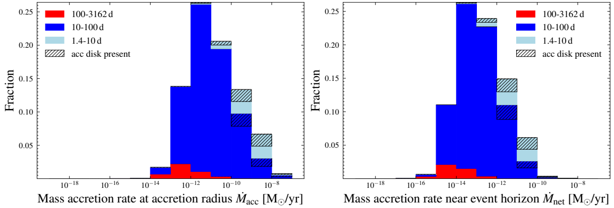
Fig. 1. Distribution of the mass-accretion rate at the accretion radius (Eq. (22), left panel ) and the mass-accretion rate at the event horizon of the BH (Eq. (32), right panel ), during the BH+OB star phase. The three colours denote the contributions from different initial orbital period ranges. The coloured histograms are stacked on each other, and the sum of the ordinate values equals unity. The black hatching shows the contribution from the BH+OB star binaries where a Keplerian accretion disc can form.
