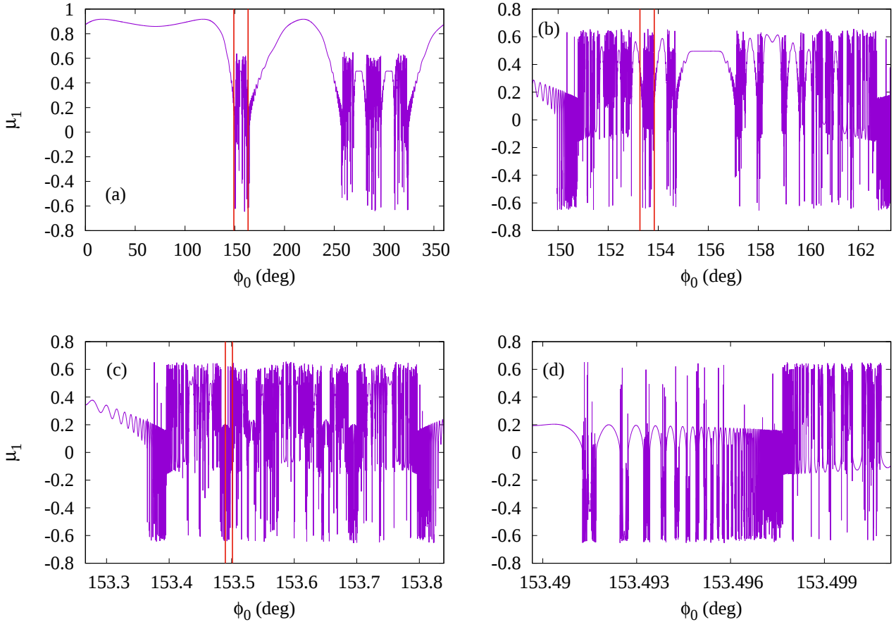
Fig. 7. Final pitch-angle cosine \mu_1 as a function of the initial gyrophase \phi_0 for \mu_0 = 0.5 in the case \beta = 90^\circ , \alpha = 60^\circ , and \mathcal{E} = 1 MeV (purple curves). Panel a refers to the whole range 0 \leq \phi_0 \leq 360^\circ , and panels b–d refer to increasingly small subintervals. Vertical red lines in panels a–c indicate the subinterval represented in the subsequent panel.
