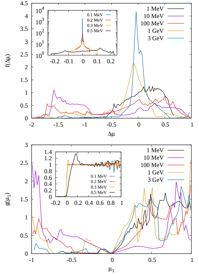
Fig. 5. Distributions f(\Delta\mu) of pitch-angle cosine variations (top panel) and g(\mu_1) of final pitch-angle cosine (bottom panel) calculated for various values of the particle energy \mathcal{E} in the range 0.1 \text{ MeV} \leq \mathcal{E} \leq 3 \times 10^3 \text{ MeV} . The cases \mathcal{E} = 0.1, 0.2, 0.3, 0.5 MeV are shown in the insets. Both panels refer to a magnetic structure where \beta = 90^\circ and \alpha = 60^\circ .
