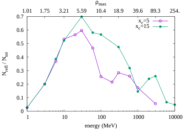
Fig. 6. Fraction N_{\text{refl}}/N_{\text{tot}} of reflected particles as a function of the particle energy \mathcal{E} for two values of SB width: 2x_c = 10 and 2x_c = 30 . Both curves correspond to \beta = 90^\circ , \alpha = 60^\circ , and \Delta x = 1 . The values of \rho_{\text{max}} are indicated in the top horizontal axis for reference.
