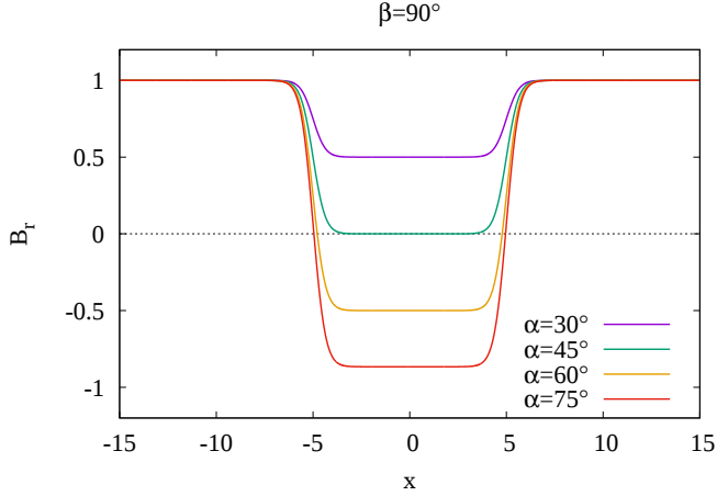
Fig. 1. Radial component B_r as a function of x , for \beta = 90^\circ and \alpha = 30^\circ, 45^\circ, 60^\circ , and 75^\circ . The radial component reverts its sign in the central region for \alpha > 45^\circ .
