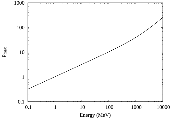
Fig. 3. Larmor radius \rho_{\max} , corresponding to \mu = 0 , as a function of the particle energy \mathcal{E} .
