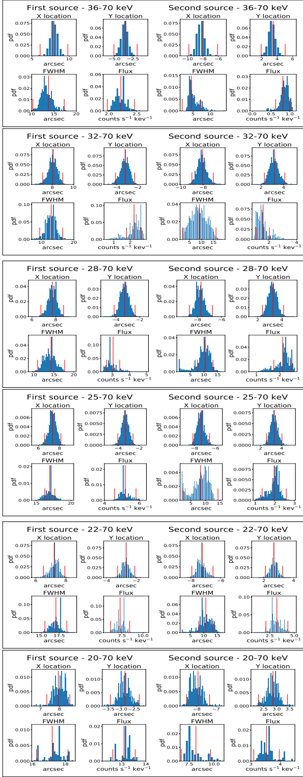
Fig. 6: Parameter histograms returned by the SMC reconstruction from the visibility amplitudes observed by STIX at 05:45:30 UT – 05:46:15 UT on November 18, 2020. From top to bottom, each box contains the histograms corresponding to the energy channels E_1 , E_2 , E_3 , E_4 , E_5 , and E_6 , respectively. Each of the six boxes contains the probability distributions of the sources locations and associated FWHM and fluxes. In red, we show the estimated means (used to provide the reconstructed maps) and standard deviations.
