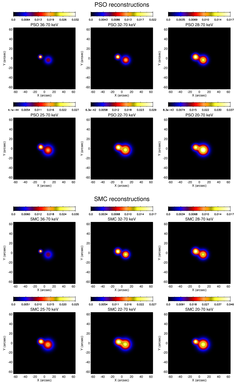
Fig. 3: Reconstructions computed via PSO (first box) and SMC (second box) from the visibility amplitudes observed by STIX at 05:45:30 UT – 05:46:15 UT on November 18, 2020. For each box, from top to bottom, left to right: reconstructions corresponding to the energy channels E_1 , E_2 , E_3 , E_4 , E_5 , and E_6 , respectively. The SMC reconstructions use the conditional mean.
