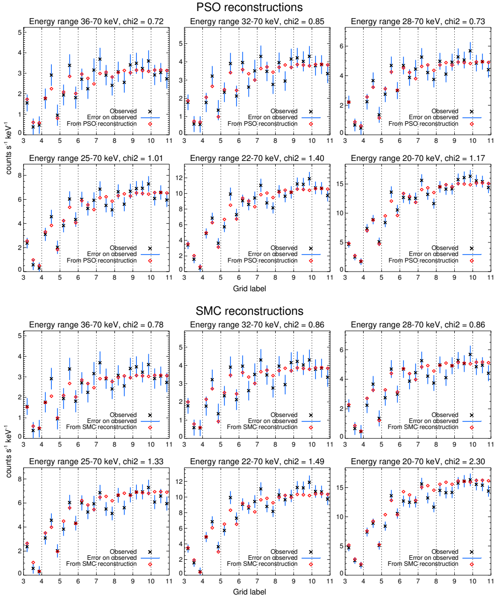
Fig. 4: Amplitude fits computed via PSO (first box) and SMC (second box) from the visibility amplitudes observed by STIX at 05:45:30 UT – 05:46:15 UT on November 18, 2020. For each box, from top to bottom, left to right: Amplitude fits corresponding to the energy channels E_1 , E_2 , E_3 , E_4 , E_5 , and E_6 , respectively.
