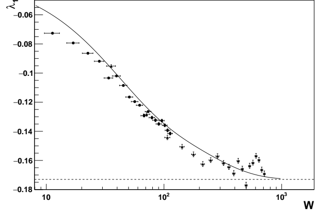
Fig. B.2. Slope of \log_{10} P(H_{20w} > x) over the interval corresponding to -7 < \log_{10} P(H_{20w} > x) < -4 as a function of W . Circles and triangles correspond to \mu_w = 2.5 and 3, respectively.
