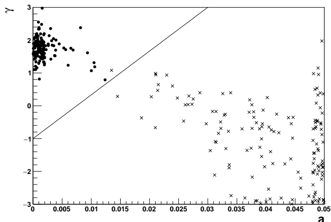
Fig. 5. Position of the lowest (dots) and highest (crosses) a points of \mathcal{E}_{90} (the region of the (a, \gamma) plane with P_w larger than 90% of the maximum) for the 144 pulsar sample. The solid line corresponds to the line L_m along which a scan is performed to obtain the model weight pulsation significance, as described in Section 4.4.
