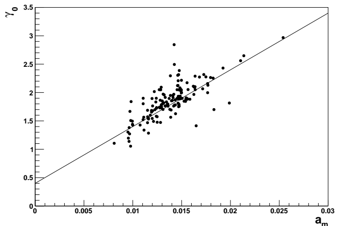
Fig. 7. Correlation between \gamma_0 , the intercept of the \mathcal{E}_{90} major axis with the a = 0 axis, and a_m , the position of the maximum P_w along L_m for the 144 pulsar sample. The solid line shows the \gamma_0 = 0.4 + 100a_m parameterization.
