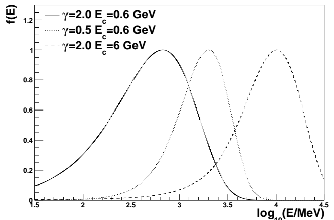
Fig. 1. Weight position independent part f(E) for three test pulsar spectra.
