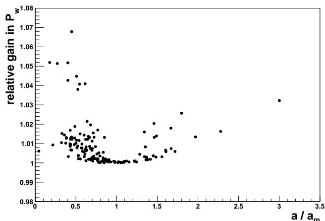
Fig. 8. Maximum P_w gain along L_M as a function of its relative position with respect to a_m for the 144 pulsar sample.
