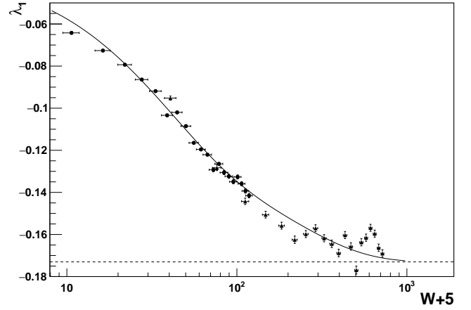
Fig. B.3. Slope of \log_{10} P(H_{20w} > x) over the interval corresponding to -7 < \log_{10} P(H_{20w} > x) < -4 as a function of W + 5 . Circles and triangles correspond to \mu_w = 2.5 and 3, respectively.
