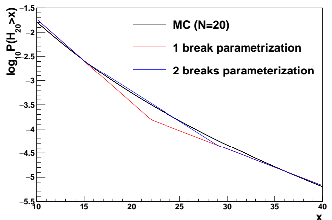
Fig. A.3. Logarithm of the H_{20} cumulative distribution for N = 20 in the x range where a single broken linear polynomial does not provide a good approximation. The black line corresponds to the MC result while the red and blue curves correspond to the single and double broken linear polynomial approximations, respectively.
