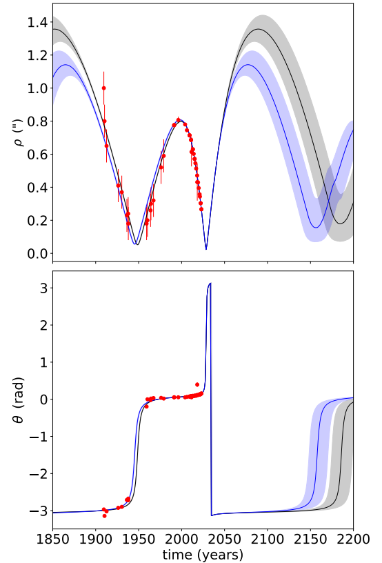
Fig. C.4. Best orbital solution for AB orbit. In all panels the solid line corresponds to the best-fit model and the shaded area to the 1 \sigma region. The solid blue lines correspond to Solution I and the black ones to Solution II. The red dots correspond to the astrometric measurements. The error bars shown in the astrometry before 1991 correspond to the large uncertainty case.
