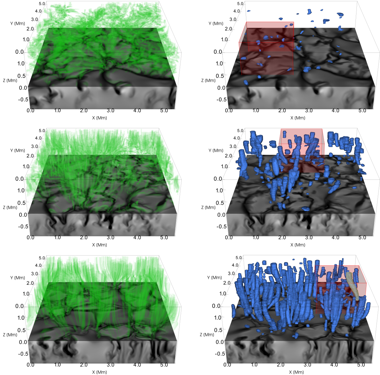
Fig. 4. 3D renderings of vortex detections computed with swirling strength (left column) and SWIRL (right column). The top, middle, and bottom rows contain data from the SSD, Bz50, and Bz200 simulations, respectively, at the 20 km spatial resolution. The red cubes indicate the location of the zoomed-in regions in Fig. 3. The vertical velocity field is plotted from the bottom of the domain up to Z = 0 Mm. The color scale is the same as in Fig. 3.
