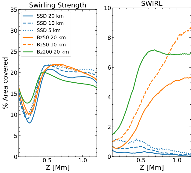
Fig. 5. Percentage of area covered by vortices detected with swirling strength (left) and SWIRL (right) as a function of height. The meaning of the curves is indicated in the figure. We note the difference in scale of the vertical axes.
