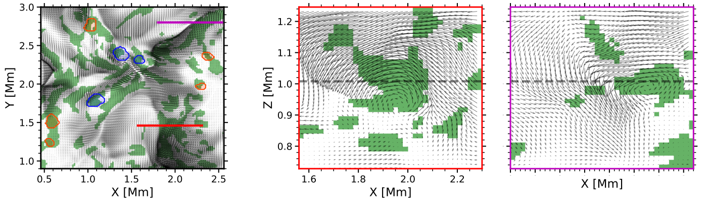
Fig. C.2. Same as Fig. C.1 but at Z = 1 Mm.
