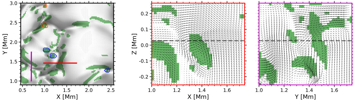
Fig. C.1. Horizontal vortices in the SSD model. Left: Same close-up view as in Fig. 3 for the SSD model at Z = 0 Mm, with two overplotted lines (red and magenta) crossing different regions of swirling strength values (green patches). Middle and right: Vertical slices taken along the positions of the lines in the left panel. The black arrows show the velocity field projected onto each slice, i.e., (v_x, v_z) for the middle panel (red line) and (v_y, v_z) for the right panel (magenta line). The horizontal dashed black line indicates the reference height ( Z = 0 Mm) of the horizontal slice shown in the left panel.
