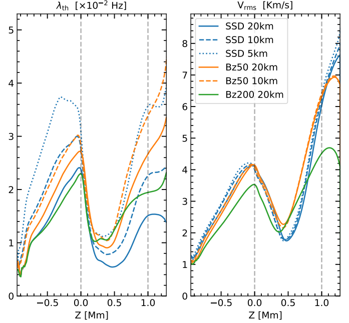
Fig. 1. Horizontal and temporal average of the height-dependent swirling strength threshold \lambda_{th} (left) and the rms velocity (right). The meaning of the curves is indicated in the figure. Vertical dashed gray lines are references at Z = 0 Mm and Z = 1 Mm.
