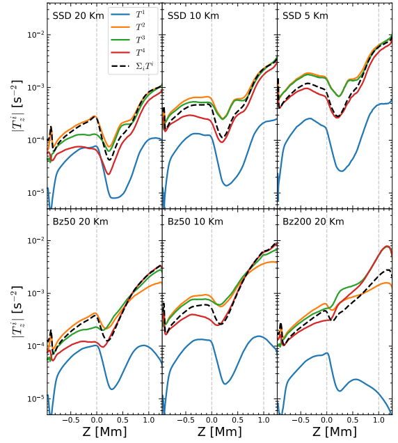
Fig. 2. Horizontal and temporal averages of the absolute values of the vertical component of the swirling strength generation terms given by Eq. (3) as a function of height, corresponding to the hydrodynamic stretching ( T^1 , blue lines) and baroclinic ( T^2 , orange lines) terms, and the magnetic baroclinic ( T^3 , green lines) and tension ( T^4 , red lines) terms. The dashed black line represents the total production of swirling strength given by \Sigma_i T^i . Each panel corresponds to the model indicated in the top left corner. The vertical dashed gray lines are visual references at Z = 0 Mm and Z = 1 Mm.
