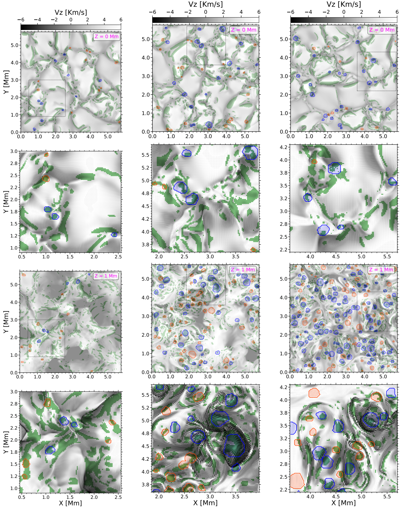
Fig. 3. Spatial distribution of vortex detections in the photosphere (first and second rows) and in the chromosphere (third and fourth rows) obtained with swirling strength (green patches) and the SWIRL code (orange and blue contours). From left to right, the columns show the results of SSD, Bz50, and Bz200 simulations at 20 km resolution. The first and third row shows the global domain at the photosphere and chromosphere, respectively. The second and fourth row shows a close-up view given by the dotted black square in the first and third rows, respectively. The black arrows in the zoom plots represent the horizontal velocity field ( v_x, v_y ). The arrow scale is the same in all the panels.
