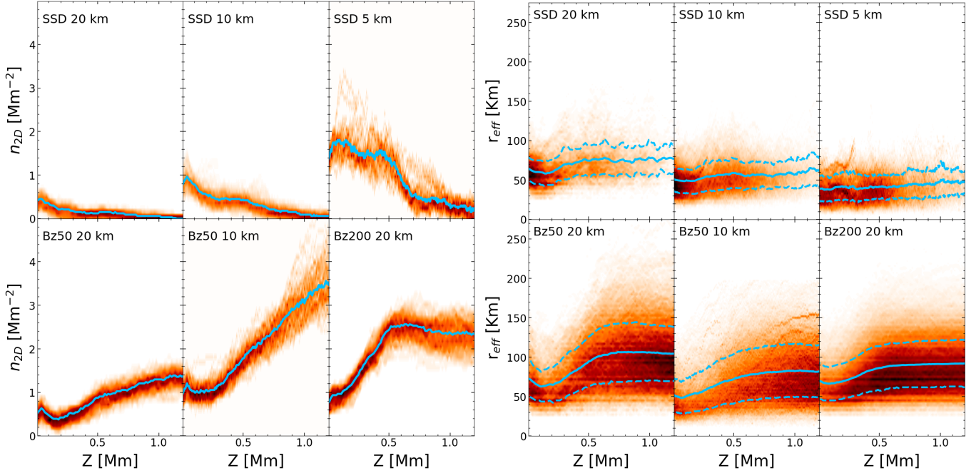
Fig. 6. 2D histograms showing the number density (left) and estimated radius (right) of vortex detections at a given height made with SWIRL. Each data point represents the density number of vortices at a single time instant. The color scale indicates the density of data points around a given value. Darker regions indicate larger concentrations of data points. The solid blue line represents the median of the distributions and the dashed blue lines in the right panel indicate the 1\sigma deviation of the distributions.
