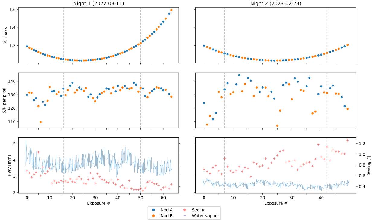
Fig. 1. Observing conditions as a function of time for Night 1 (left) and Night 2 (right). The vertical grey lines indicate the extent of the transit event. Top: airmass. The blue and orange coloured points represent nodding positions A and B. Middle: as above but for median S/N per pixel. Bottom: weather conditions. Red crosses correspond to the seeing in arcseconds for each exposure, and the blue line to the precipitable water vapour (PWV), i.e. water vapour along our line of sight, throughout the night in millimetres.
