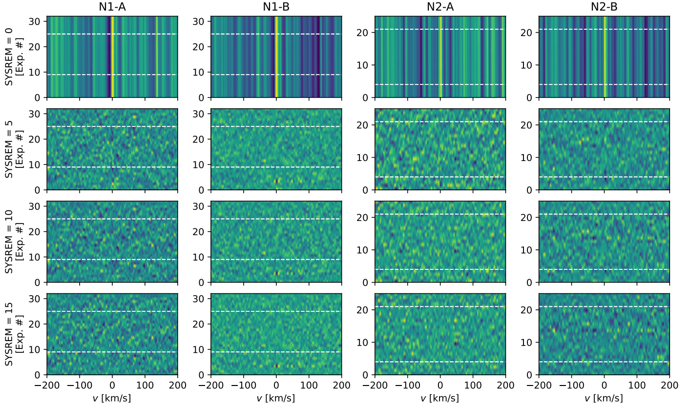
Fig. 8. Cross-correlation function maps of the A and B frames for Night 1 (N1) and Night 2 (N2) from our VLT/CRIRES + data. For each plot, the dotted white lines denote the start and end of the transit. The data are shown for SYSREM iterations 0, 5, 10, and 15 in order to demonstrate that all non-zero iterations are clear of any obvious contamination or artefacts. The maps show cross-correlation with the ‘global’ template from the CHI-model (see Table 3) that includes a cloud deck at P = 10^{-5} bar.
