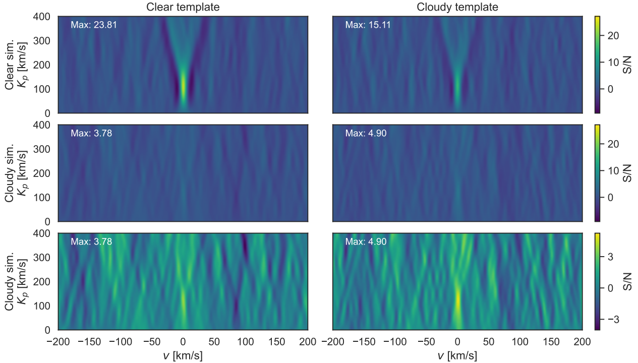
Fig. 5. Simulated K_p - v plots used to test the impact of including or excluding cloud decks in four different test cases. Top: simulations of a ‘clear’ WASP-107 b that has no cloud deck present cross-correlated with a ‘clear’ template that excludes clouds (left) and with a ‘cloudy’ template that includes clouds (right). Middle: same as the top row but now simulating a ‘cloudy’ WASP-107 b with a cloud deck present at P = 10^{-5} bar, shown with the same colour scale as the test above for comparison. Bottom: same as the middle row but now shown with its own colour scale for reference.
