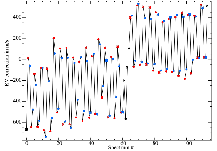
Fig. 2. Wavelength correction illustrated as RV shifts to the wavelength in the middle of a spectral order (vertical axis) determined for each spectrum. Red and blue asterisks show AA or BB nodding pairs of consecutive exposures where no interruption in AO operation occurred and thus we expected no change in the across-the-slit position. The differences in these pairs provide an alternative estimate of the precision. The mean differences are 80 m/s for N1 and 36 m/s for N2, which are to be compared to the estimates based on telluric line centres giving 91 and 53 m/s, correspondingly. The large shift between the nights was measured by cross-correlating the two templates and converting it to an extra RV for each night to provide a sense of scale for the reader. In reality, most of this shift is translation (not RV) due to the reproducibility of the CRIRES + wavelength settings.
