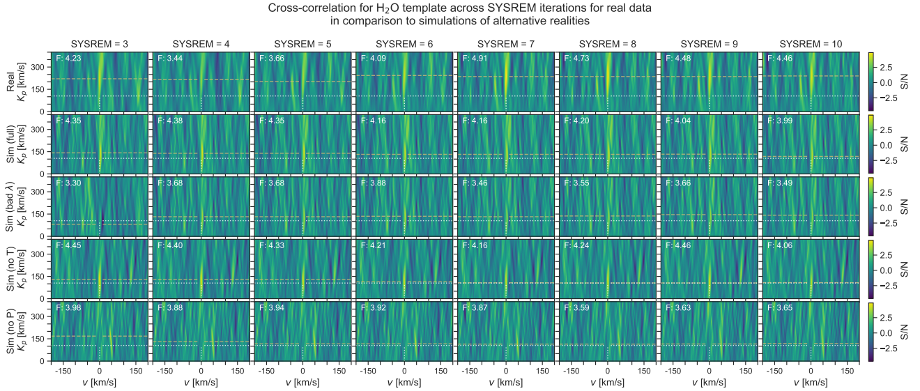
Fig. 11. Real and simulated K_p - v plots for SYSREM iterations 3–10 cross-correlating with the H 2 O template including clouds. In each plot, the dotted white line denotes the expected location of the peak, and the dashed yellow line denotes the actual location of the peak. First row: real data K_p - v map as shown in Fig. 10. Second row: simulated observation including all expected components (a ‘full’ simulation). Third row: simulated observation with an intentionally perturbed wavelength solution (‘bad \lambda ’). Fourth row: simulated observation excluding telluric contamination (‘no T’). Fifth row: simulated observation excluding a planetary atmosphere (‘no P’).
