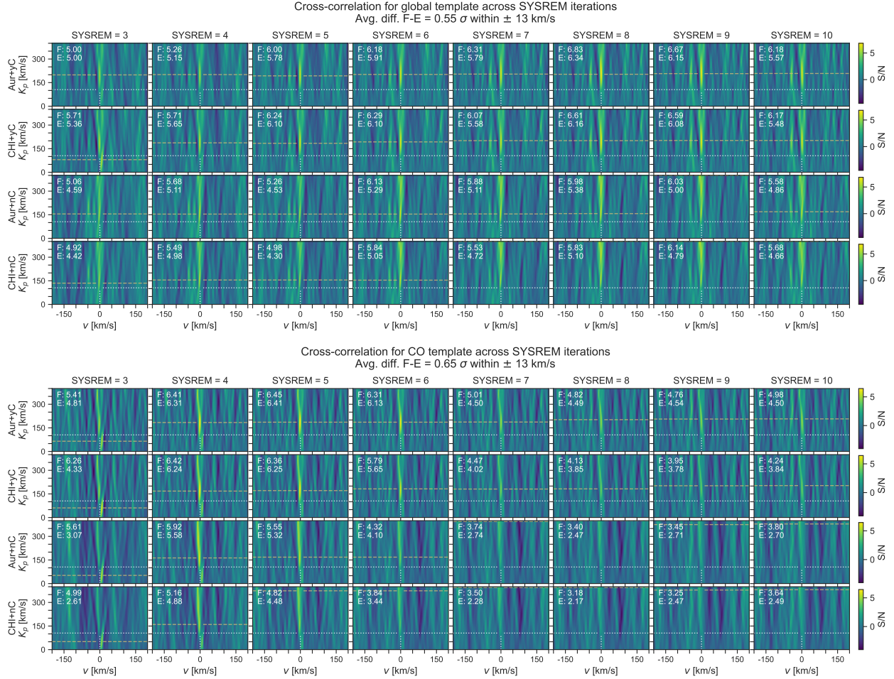
Fig. 9. K_p - v plots for SYSREM iterations 3-10 cross-correlating with the global template top and with the CO template bottom . In each plot, the dotted white line denotes the expected location of the peak, and the dashed yellow line denotes the actual location of the peak. In the top left, the F-value denotes the maximum value found across the ‘full’ map, and the E-value denotes the maximum value found within the ‘expected’ location, i.e. within 13 km/s of K_p = 105 km/s and v = 0 km/s.
