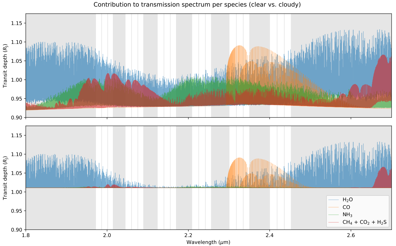
Fig. 4. Simulated global (i.e. including all species) transmission spectrum of WASP-107 b, coloured by species contribution, based on parameters from the results of the Welbanks et al. (2024) CHIMERA forward model and as generated by petitRADTRANS at a resolving power of R = 10^6 . The plot demonstrates the notable change of the spectrum’s shape when either excluding ( top , showing a ‘clear’ atmosphere) or including ( bottom , a ‘cloudy’ atmosphere) the presence of a grey cloud deck at P = 10^{-5} bar. The grey areas denote wavelength ranges that fall outside of the spectral orders of the VLT/CRIRES + K band of \sim 2.0\text{--}2.5\ \mu\text{m} (1972–2452 nm).
