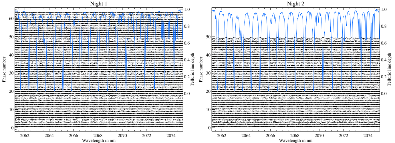
Fig. 3. Per-phase differences (black lines) between observed WASP-107 b spectra and an inverse model of the mean nightly telluric absorption with a mean PSF profile scaled to the appropriate airmass. This spectral segment is totally dominated by telluric features and contains no significant stellar lines. Vertical offsets between each subsequent phase were added for visibility. A blue overplotted spectrum shows the mean telluric spectrum for each night at the lowest airmass. Note that substantial structure in the residuals is only visible for two phases on Night 2 (third from bottom, and topmost), which is indicative of not only the PSF changes in those phases but also the general stability of the PSF otherwise.
