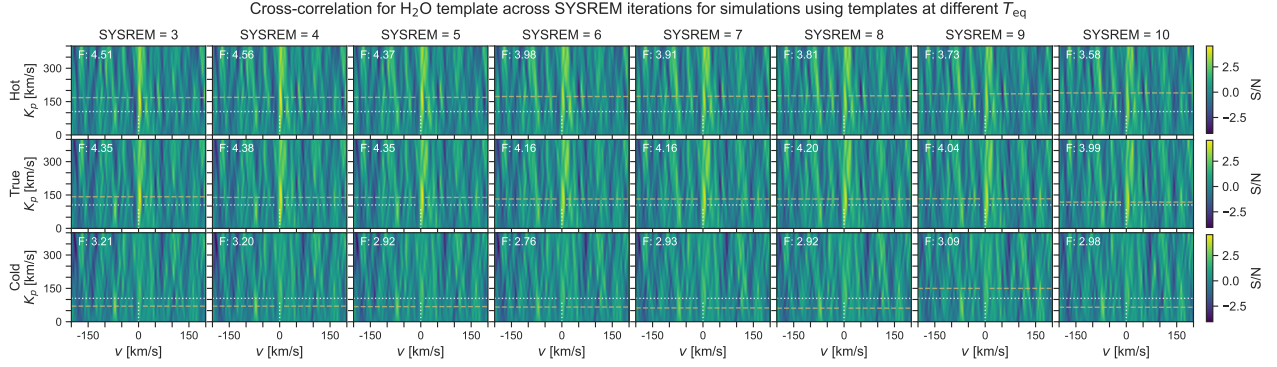
Fig. 12. Simulated K_p - v plots for SYSREM iterations 3–10 cross-correlating with the \text{H}_2\text{O} template including clouds. In each plot, the dotted white line denotes the expected location of the peak, and the dashed yellow line denotes the actual location of the peak. All simulated observations include tellurics. Top row: cross-correlation with a template with equilibrium temperature T_{\text{eq}} = 1200 K (‘hot’). Middle row: cross-correlation with a template with equilibrium temperature T_{\text{eq}} = 738 K (‘true’). Bottom row: cross-correlation with a template with equilibrium temperature T_{\text{eq}} = 300 K (‘cold’).
