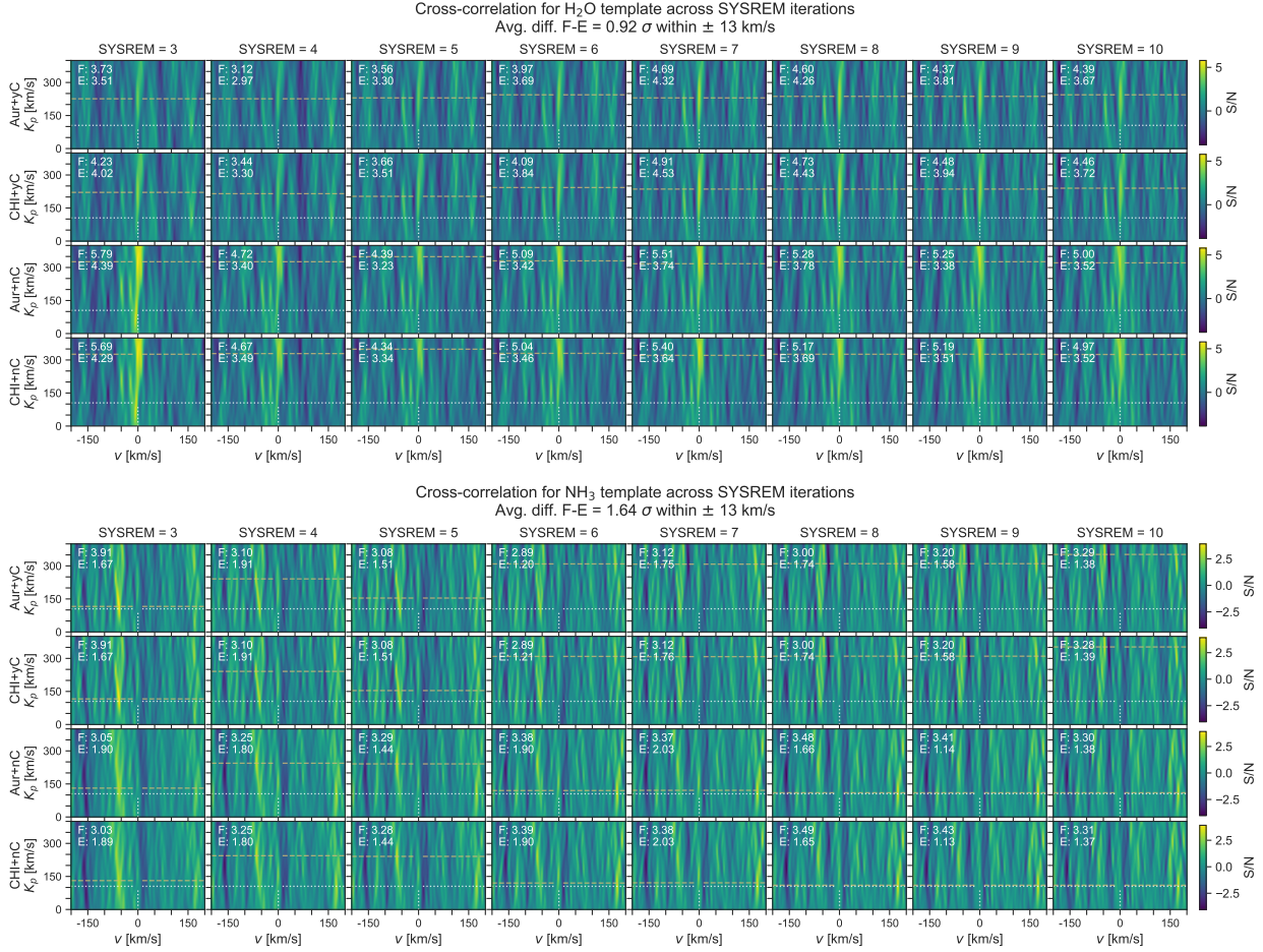
Fig. 10. K_p - v plots for SYSREM iterations 3-10 cross-correlating with the H 2 O template top and with the NH 3 template bottom . In each plot, the dotted white line denotes the expected location of the peak, and the dashed yellow line denotes the actual location of the peak. In the top left, the F-value denotes the maximum value found across the ‘full’ map, and the E-value denotes the maximum value found within the ‘expected’ location, i.e. within 13 km/s of K_p = 105 km/s and v = 0 km/s.
