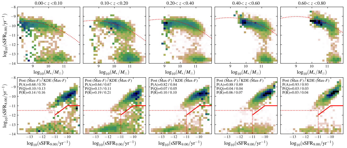
Fig. 8. Top: Distribution of Euclid galaxies across the stellar mass versus \text{sSFR}_8 plane. The dotted line denotes the definition of the SFMS by Popesso et al. (2023). Bottom: Distribution of Euclid galaxies across the \text{sSFR}_9 versus \text{sSFR}_8 plane. The dotted and solid lines denote the retired and quenched domain demarcation lines, respectively.
