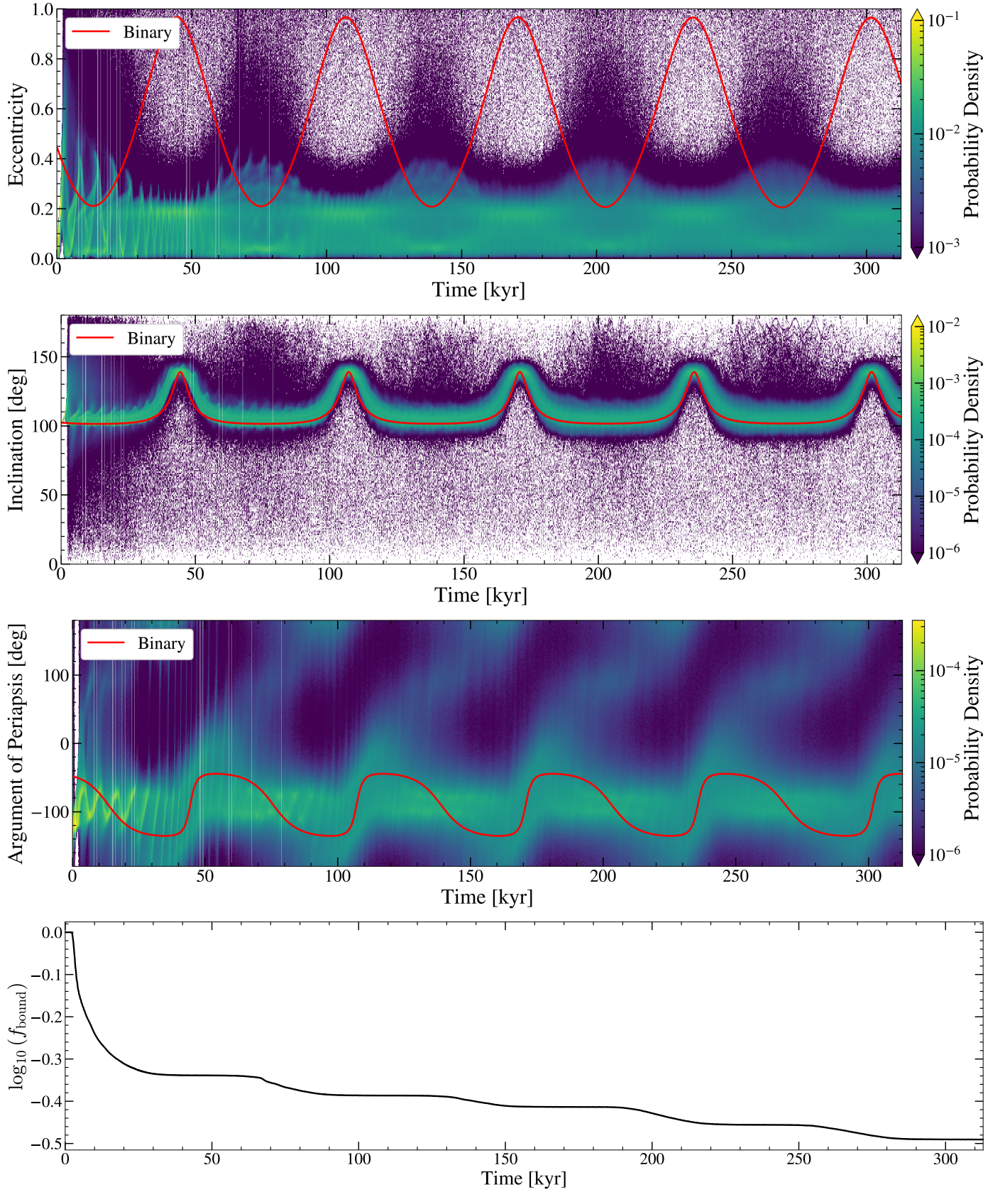
Fig. 3. Top three panels: evolution of the distribution of the eccentricity, inclination, and the argument of periapsis of the bound ( e < 1 ) disk particles. The evolution of the binary orbital elements is also plotted (solid red lines). The orbital elements of the binary oscillate on a timescale of T_{\text{VZLK}} = 62.5 kyr. Bottom: fraction of bound disk particles over time. After an initial period of rapid mass loss, the disk loses mass in periodic bursts on the vZLK timescale.
