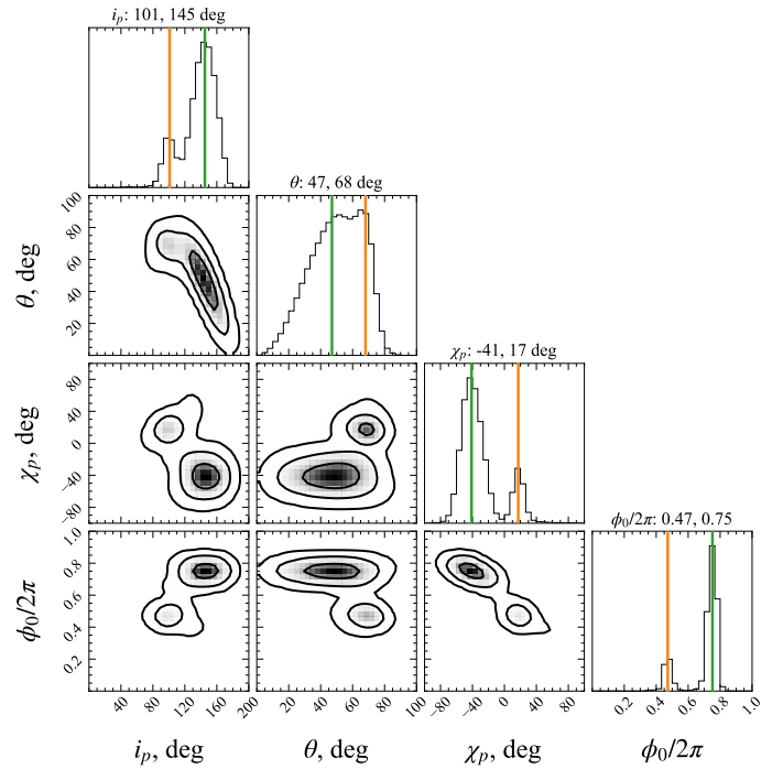
Fig. 6. Posterior distributions of the RVM parameters derived from the phase-resolved PAs (spectro-polarimetric analysis). Contours correspond to 1\sigma , 2\sigma , and 3\sigma CLs. The histograms show the normalized one-dimensional distributions for a given parameter derived from the posterior samples. Vertical lines in the diagonal panels mark the median values of the two posterior clusters.
