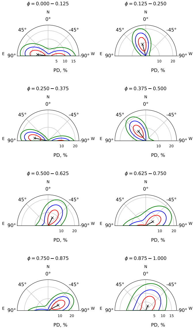
Fig. 5. Protractor plots showing phase-resolved PD (radius) and PA (azimuth) in the 2–8 keV range. Contours indicate 1, 2, and 3\sigma CLs for two parameters, shown in red, blue, and green, respectively. The cross marks the best-fit point, and the line indicates the polarization direction.
