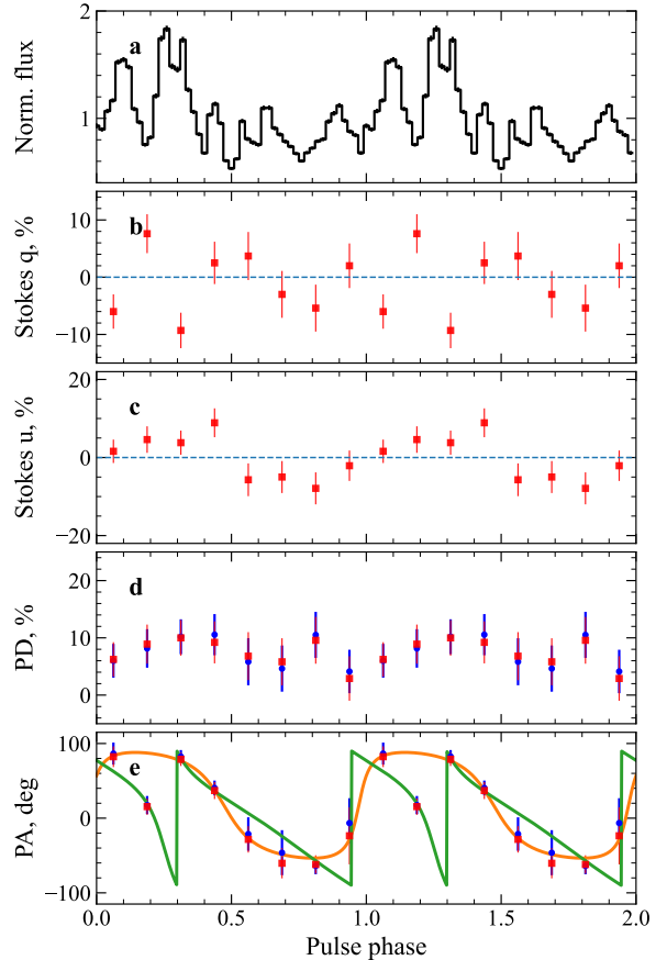
Fig. 3. Phase-resolved properties of 4U 1954+319 over two pulse cycles. The PD and PA measurements derive from two methods: blue points show spectro-polarimetric analysis results, and square red symbols show model-independent measurements obtained with ixpepolarization . Panels display (a) the normalized pulse profile in the 2–8 keV band derived from the IXPE data, (b)–(c) the Stokes parameters q and u , (d) the PD, and (e) the PA. The PA panel shows two RVM solutions from Table 3, corresponding to two distinct posterior clusters in Fig. 6: Solution 1 (orange) and Solution 2 (green).
