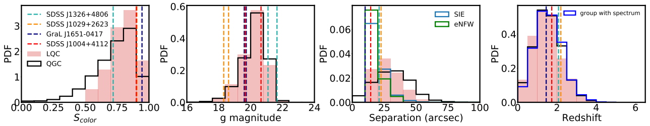
Fig. 7. Statistical properties of LQC, QGC, and discoverable known lenses. First panel: distribution of the colour similarity, S_{\text{colour}} (we note that the vertical marker line for SDSS J1004+4112 falls on top of the line for SDSS J1029+2623, which makes the line for SDSS J1029+2623 difficult to see). Second panel: distribution of the Pan-STARRS1 g band magnitudes for all quasar images contained in each quasar candidate group or known lensed quasar system. Third panel: distribution of the maximum image separation. The blue and green curves are the simulation results derived from the model in Appendix B, corresponding to different lens mass profile models. Fourth panel: distribution of the photometric redshift z_{\text{ph}} for all quasar images in each group or known system; the blue curve shows the z_{\text{ph}} distribution for those quasar candidate groups in the QGC that have sufficient spectroscopic matches. Dashed lines indicate the positions of the corresponding values for the four discoverable known lenses in CatNorth. Stepped black histograms trace the distributions for the QGC.
