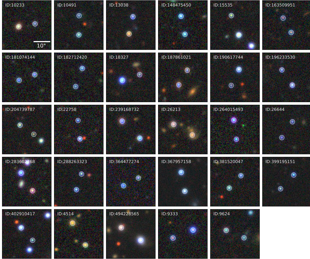
Fig. 11. DESI Legacy Imaging Surveys DR9 grz composite images of the 29 dual quasar candidate systems. Each cut-out spans 30 arcsec \times 30 arcsec. White circles mark the positions of the quasar candidate images.
