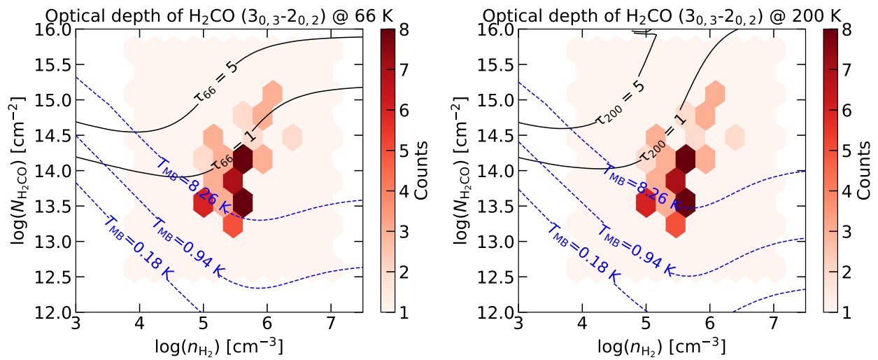
Fig. D.1: Optical depth of p\text{-H}_2\text{CO} (3_{0,3}-2_{0,2}) as a function of n(\text{H}_2) - N(p\text{-H}_2\text{CO}) for a fix value of T_{\text{kin}} . The color hexagonally binned distributions display the PyRADEX+MCMC constrained n(\text{H}_2) and N(p\text{-H}_2\text{CO}) of our sources. The black solid curves show the optical depth of \tau = 1 and \tau = 5 for p\text{-H}_2\text{CO} (3_{0,3}-2_{0,2}) transition on top of n(\text{H}_2) and N(p\text{-H}_2\text{CO}) space, assuming fixed kinetic temperature of 66 K (the median temperature of our sample; left panel) and 200 K (higher temperature; right panel). The blue dashed curves indicate the contour corresponding to the brightest, average, and faintest observed intensities for p\text{-H}_2\text{CO} (3_{0,3}-2_{0,2}) transition (see the text).
