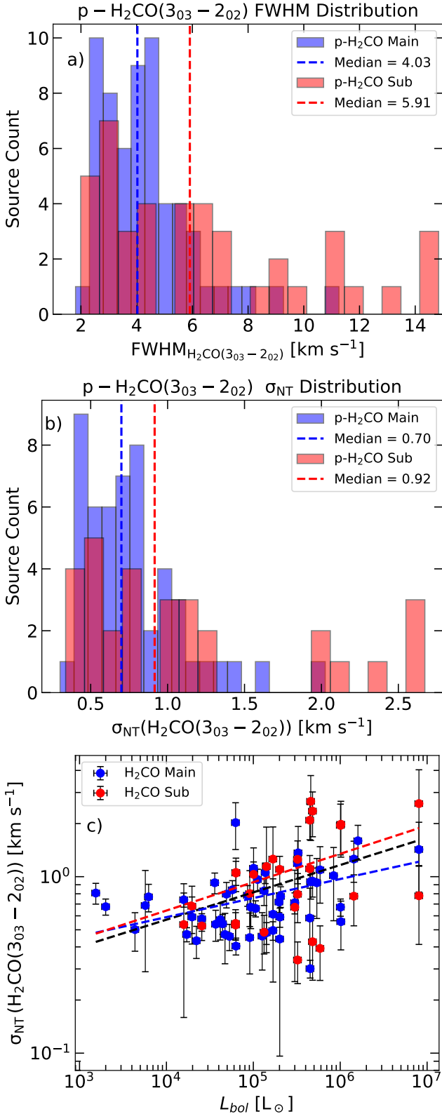
Fig. 10. Distributions of (a) FWHM and (b) \sigma_{NT} of the p -H 2 CO ( 3_{0,3}-2_{0,2} ) transition. The blue and red histograms represent the H 2 CO Main and H 2 CO Sub components, respectively, with the corresponding dashed lines marking their median values. Panel c: relation between \sigma_{NT} and L_{bol} . The black, blue, and red dashed lines indicate the power-law fits for all components combined, the Main components, and the Sub components, respectively.
