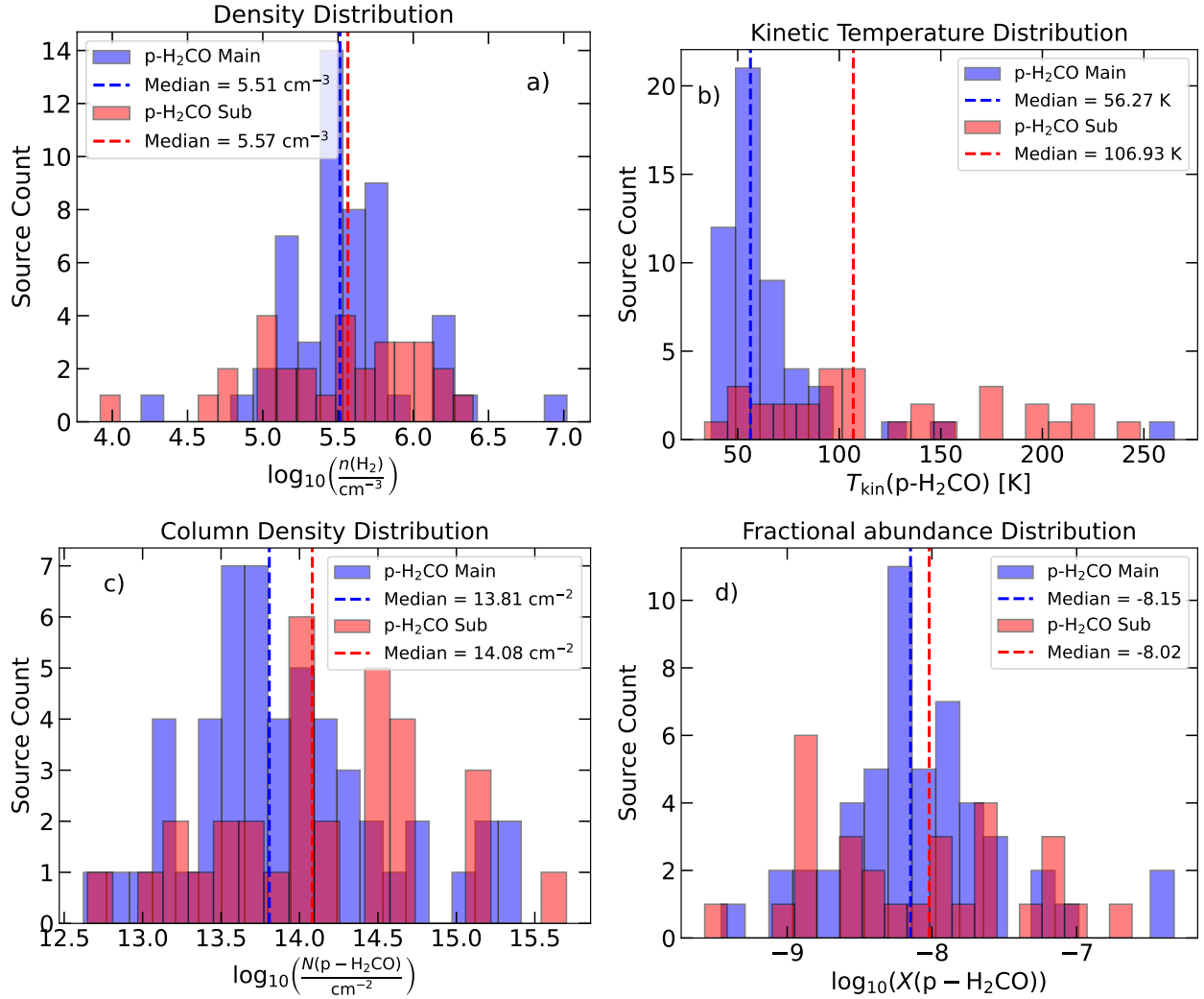
Fig. 4. Distributions of the pyRADEX+MCMC derived (a) n(\text{H}_2) , (b) T_{\text{kin}} , (c) N(p\text{-H}_2\text{CO}) , and (d) p\text{-H}_2\text{CO} fractional abundance, X(p\text{-H}_2\text{CO}) toward the different velocity components identified in our sample, as traced by the p\text{-H}_2\text{CO} . The blue and red histograms represent the distributions for the “H 2 CO Main” and “H 2 CO Sub” components, respectively, while the corresponding dashed lines indicate the median values of each distribution.
