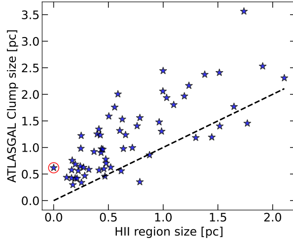
Fig. A.2: Comparison of physical size of H II regions and associated ATLASGAL clump size taken from Csengeri et al. (2014). The dashed black line shows the line of equality. The red circle represents only unresolved H II region, G030.720–0.082, in our sample.
