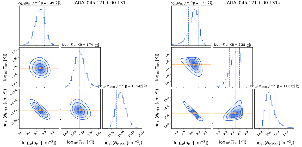
Fig. A.4: Example corner plot for AGAL045.121+00.131. To constrain physical properties of the molecular clouds we used the non-LTE RADEX modelling with MCMC algorithm, here we show the corresponding corner plot for each Gaussian component displaying the 1D histogram of the posterior distribution for each parameter (kinetic temperature, T_{\text{kin}} , \text{H}_2 density, n(\text{H}_2) , and p\text{-H}_2\text{CO} column density, N(p\text{-H}_2\text{CO}) ). The histograms represent the PDFs of the Monte Carlo fit parameters, while the blue curves represent the scatter plot of the joint distribution between the two parameters. The orange solid lines indicate the median of the PDFs, representing the most likely fit parameters, and the dotted blue lines correspond to the 1\sigma confidence intervals. The subtitle of each corner plot shows most likely value of the parameters with upper and lower 1\sigma error.
