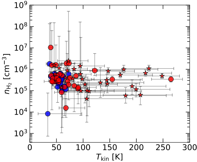
Fig. 3. Distribution of the sources in the n(\text{H}_2) – T_{\text{kin}} plane. The blue and red colors respectively represent sources with single and multiple component Gaussian profiles. Filled circles denote components classified as “H 2 CO Main,” while stars indicate those identified as “H 2 CO Sub.”
