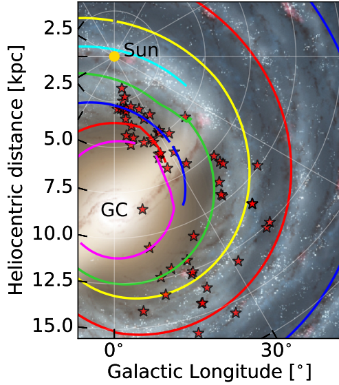
Fig. 1. Galactic distribution of the source sample. The locations of the targets are denoted by red stars on an artistic rendering of the Milky Way. The distances to the observed H II regions and their associated clumps are taken from Paper I (and references therein). The spiral arms are marked following the description presented in Reid et al. (2019), and the individual spiral arms are colored as follows: the 3 kpc in magenta, the Norma-Outer Arm in red, the Scutum-Centaurus Arm in blue, the Sagittarius-Carina Arm in green, the Local Arm in cyan, and the Perseus Arm in yellow.
