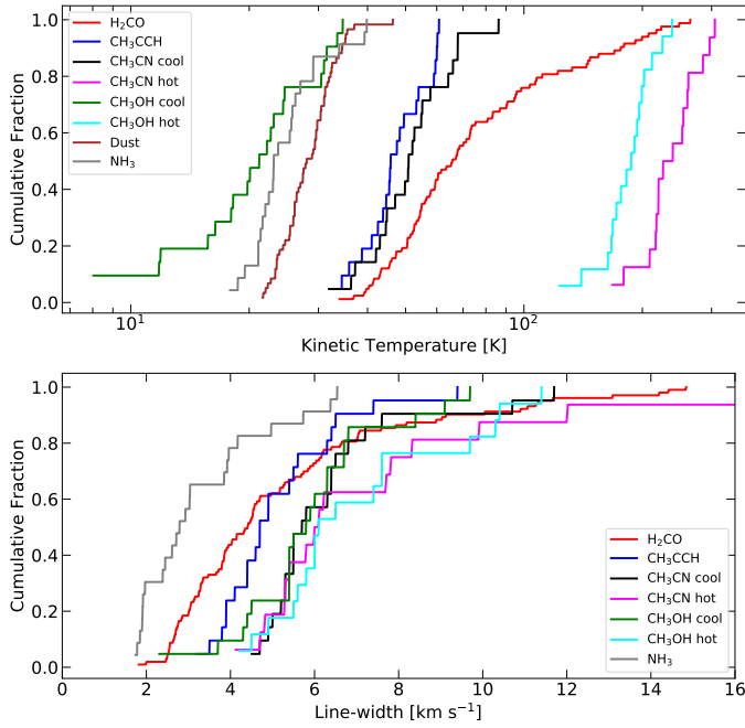
Fig. 8. Cumulative distribution functions for temperatures ( top panel ) and line width ( bottom panel ) for different H II regions. Different colors represent various tracers and components, as indicated in the legend. The \text{NH}_3 properties are from Wienen et al. (2012) . The \text{CH}_3\text{CCH} , \text{CH}_3\text{OH} (hot and cold), and \text{CH}_3\text{CN} (hot and cold) properties are from Giannetti et al. (2017) , whereas dust properties are from Urquhart et al. (2018) .
