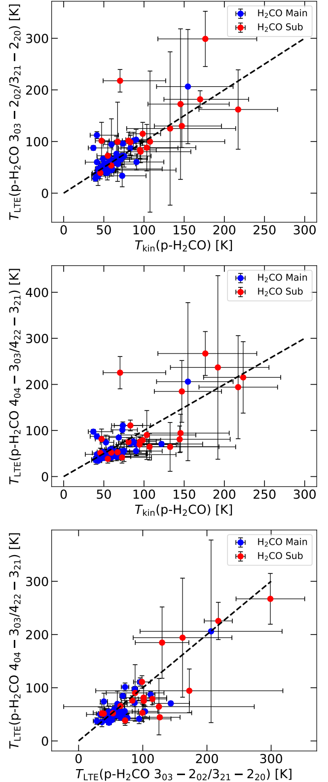
Fig. 6. Comparison between the kinetic temperatures derived from pyRADEX+MCMC modeling and using the p\text{-H}_2\text{CO} integrated line intensities ratios R_1 (top panel) and R_2 (middle panel). Bottom panel: comparison of the kinetic temperatures derived from R_1 and R_2 . The LTE temperature uncertainties are from uncertainties in the integrated intensities of the observed p\text{-H}_2\text{CO} lines. The dashed black lines indicate a slope of unity.
