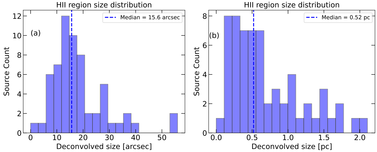
Fig. A.3: Distribution of (a) angular and (b) physical deconvolved FWHM size of H II region. The vertical dashed line shows the median value of the distribution.
