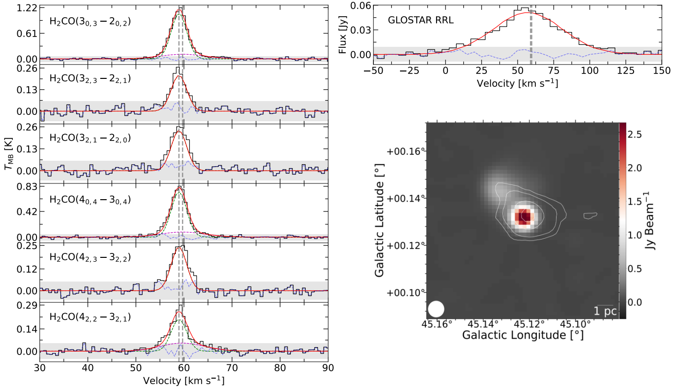
Fig. 2. Spectra of the different p -H 2 CO and RRL transitions studied in this work toward AGAL045.121+00.131. Left panels: spectra of all six of the observed p -H 2 CO transitions (black) along with the multicomponent Gaussian fitting (green and magenta) and residual of the fitting (dashed blue). The total fit is displayed in red and the gray shaded region demarcates the 3\sigma level of the rms noise. The vertical dashed gray lines mark the centroid velocities of each fit Gaussian component. Right panel: spectra of the stacked GLOSTAR \langle Hn \rangle RRL in black alongside the Gaussian fit in red. Also displayed is the 5.3 GHz radio continuum emission map obtained with the GLOSTAR VLA D configuration toward this source and overlaid with white contours is the ATLASGAL 870 \mu m. The white filled circle shows the 25'' GLOSTAR beam.
