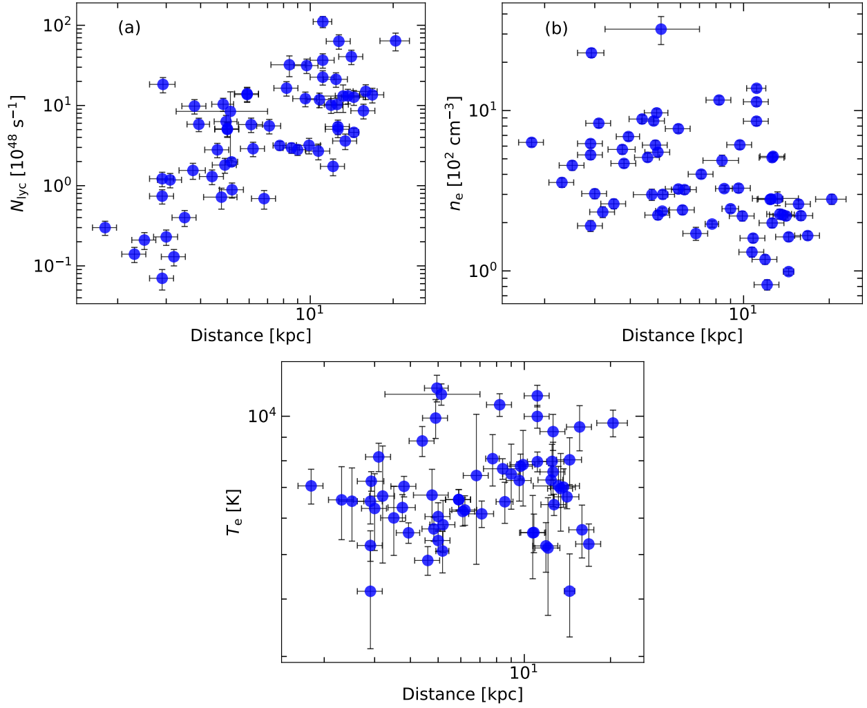
Fig. B.1: Relation between the distances and (a) N_{\text{Lyc}} , (b) n_e , and (c) T_e for our sample.
