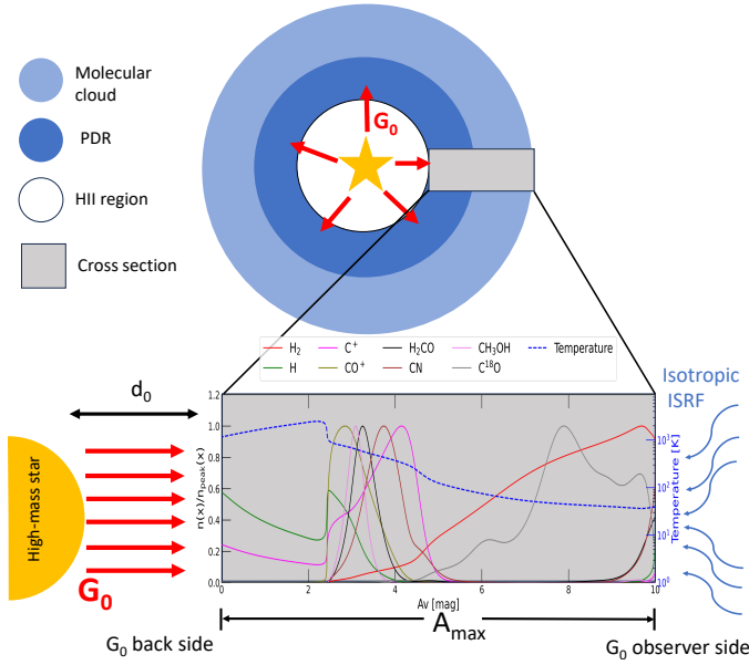
Fig. 9. Schematic depicting a fully evolved H II region in which accretion onto the central star has ceased but the region remains embedded in its surrounding environment. Additionally, it outlines the various input parameters used in the Meudon PDR code and output molecular abundance as presented in Fig. A.5.
