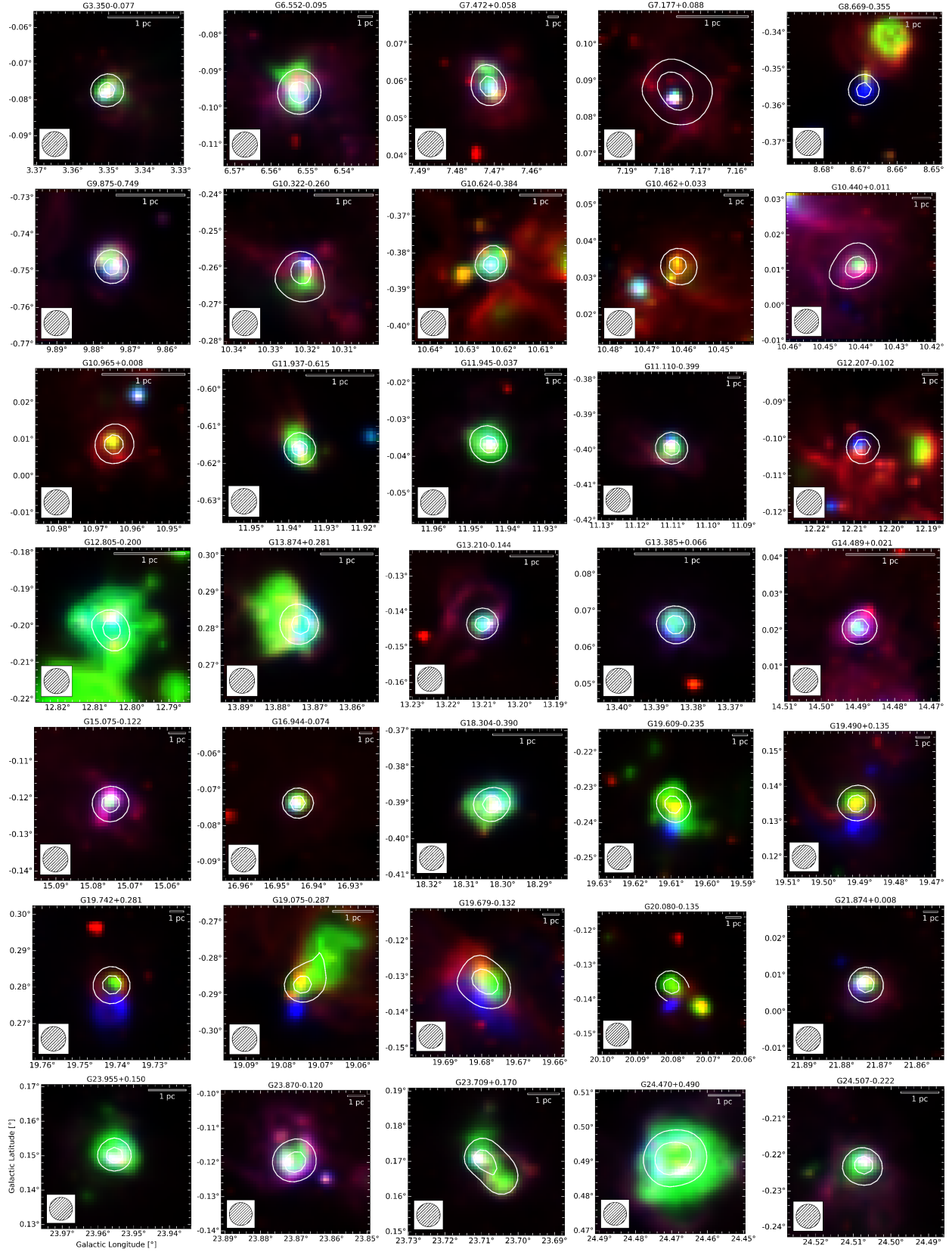
Fig. A.1: Three-color composite images of the targets of this study. The images combine mid-infrared data from Herschel 70 \mu\text{m} (red), MIPS GAL 24 \mu\text{m} (green), and GLIMPSE 8.0 \mu\text{m} (blue), overlaid with the GLOSTAR 5 GHz radio continuum contours in white. The filled white circle in corner represents the 25'' beam of the radio continuum data from Paper I.
