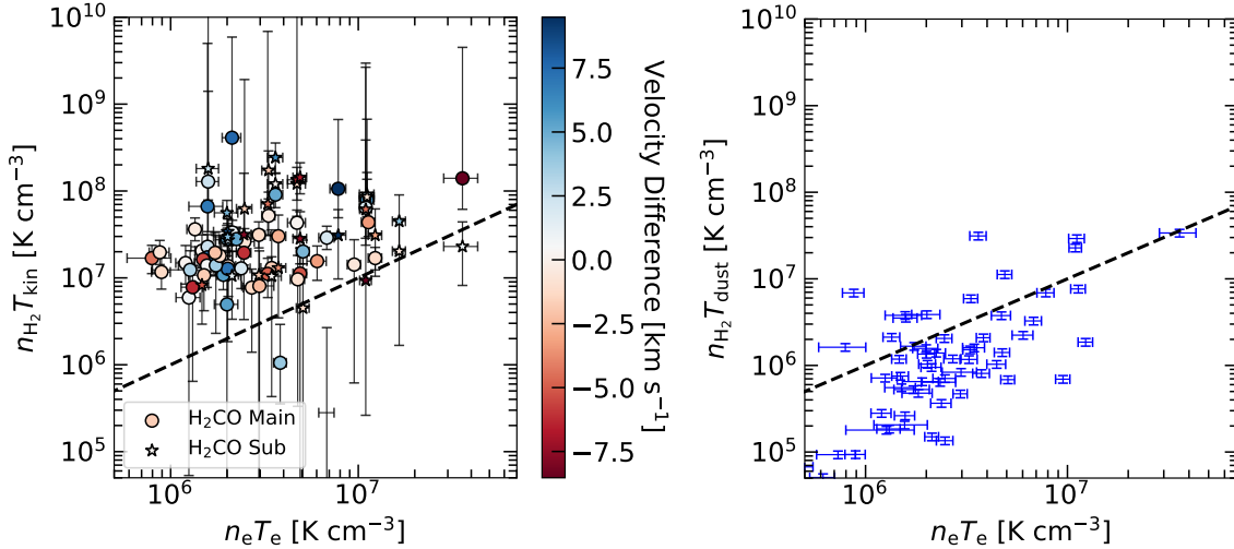
Fig. 11. Comparison between the thermal pressure of ionized and molecular gas. The color bar indicates the velocity difference between the RRL and p -H 2 CO transitions. Left panel: n(\text{H}_2) and T_{\text{kin}} derived from p -H 2 CO in this work. Right panel: n(\text{H}_2) and T_{\text{dust}} estimated from the 870 \mu\text{m} emission (Urquhart et al. 2018, 2022), representing the average clump pressure. The dashed black lines mark the slope of equal pressure. The plots are set to the same scale for visual comparison.
