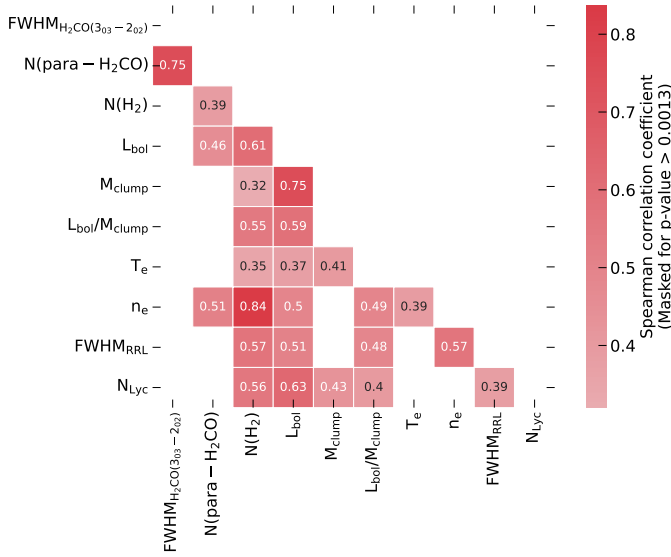
Fig. 7. Correlation matrix showing the relationships between various physical properties of molecular gas, ionized gas, and dust clumps. The color bar and annotations indicate the Spearman’s correlation coefficients. We flagged and excluded correlations with p -values > 0.0013 ( 3\sigma ), thereby removing statistically insignificant relationships.
