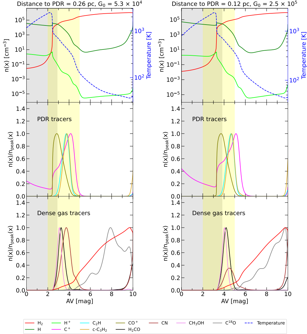
Fig. A.5: Meudon PDR model results for a constant thermal pressure of P_{\text{th}} \sim 4.6 \times 10^7 \text{ K cm}^{-3} . Left panel: Meudon PDR model run with input spectral type of O5V, distance to PDR of d_0 = 0.26 \text{ pc} , and far-UV flux, G_0 \sim 5.3 \times 10^4 in units of Habing field. Right panel: Meudon PDR model run with input spectral type of O5V, distance to PDR of d_0 = 0.12 \text{ pc} , and far-UV flux, G_0 \sim 2.5 \times 10^5 in units of Habing field. The top plots show the evolution of hydrogen species – \text{H}_2 , \text{H} , and \text{H}^+ , as well as the gas temperature as a function of visual extinction A_V . The middle and bottom plots present the spatial density profiles of key PDR and dense gas tracer molecules (see main text), where each density has been normalized to its maximum value within the cloud.
