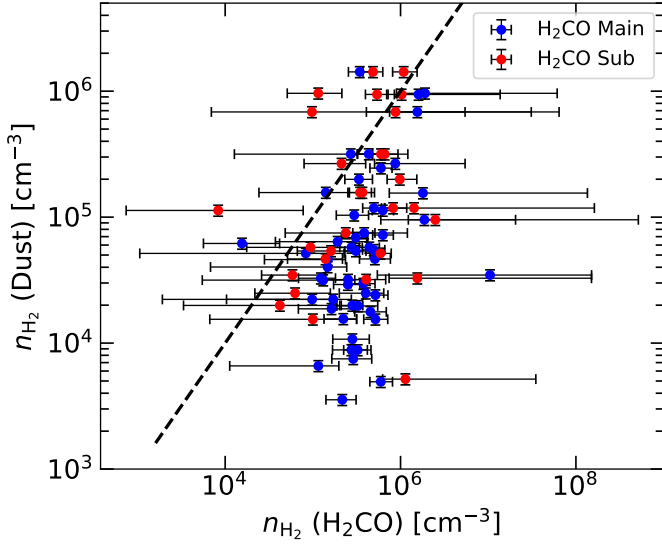
Fig. 5. Comparison between n(\text{H}_2) probed by 870\ \mu\text{m} emission from dust and p\text{-H}_2\text{CO} as derived from our pyRADEX+MCMC models. The dashed black line displays a slope of unit value.
