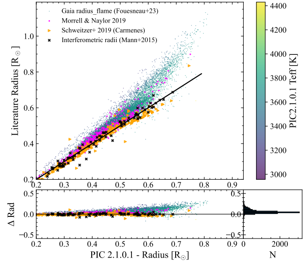
Fig. 11. Comparison of stellar radii from different sources. Top: comparison between P4 radii estimated in this work (x-axis) and the radius_flame values from Gaia DR3 (y-axis), shown with a colour map representing the effective temperature. The radii from other literature works are also shown. The solid line is the 1:1 relation. Bottom: distribution of the differences between the P4 radii and Gaia DR3 radius_flame values and other external literature estimates.
