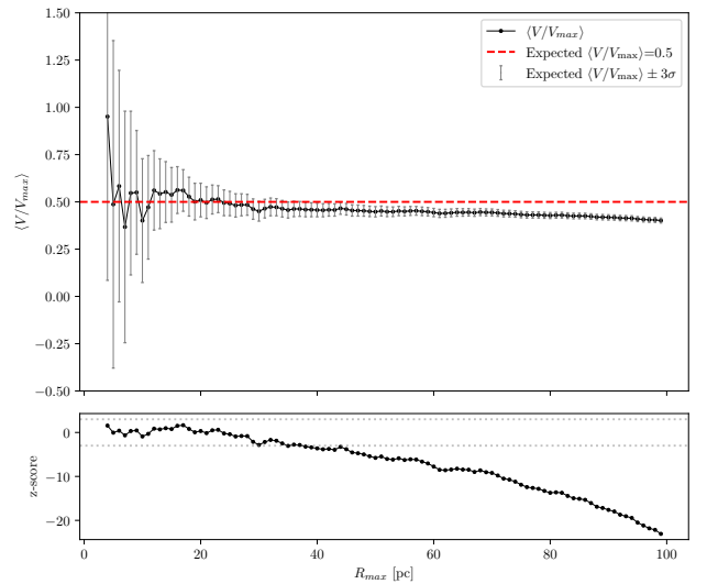
Fig. 8. Top: \langle V/V_{\max} \rangle as a function of R_{\max} for the P4 targets with 7 \leq M_{G,0} \leq 14 , where V_{\max} is the corresponding maximum volume. The red dashed line indicates the expected value of 0.5, and the grey error bars show the 3\sigma statistical uncertainty. Bottom: z-score of the deviation from the expected 0.5 value, defined as z = (\langle V/V_{\max} \rangle - 0.5)/\sigma , as a function of R_{\max} . The horizontal dotted grey lines indicate the \pm 3\sigma limits used to assess the completeness of the sample.
