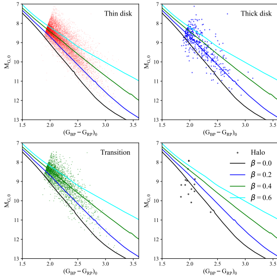
Fig. 15. CAMD of the different P4 galactic populations, compared with a 200 Myr solar metallicity isochrone with different \beta_{\text{spot}} values (Franciosini et al. 2022).
