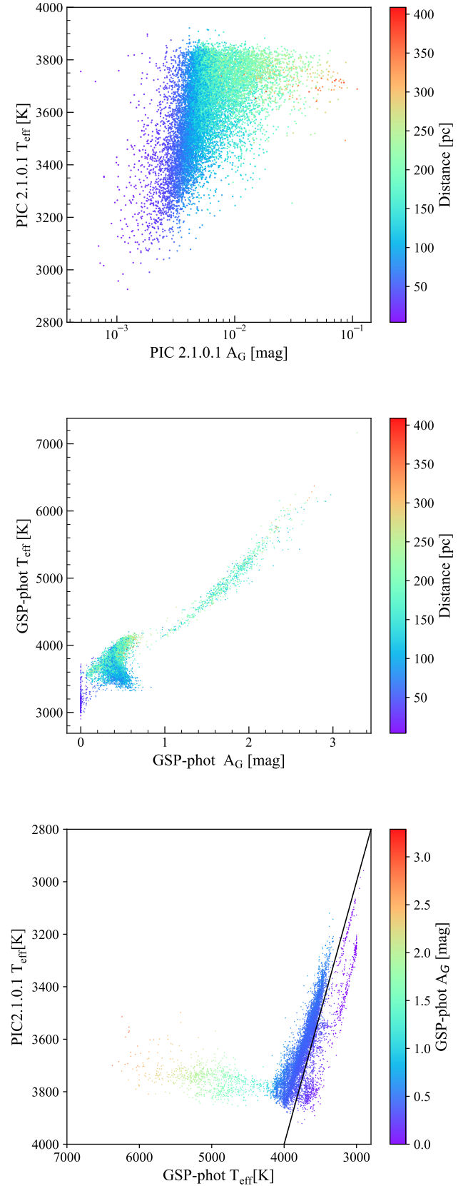
Fig. 12. Effective temperatures and extinction derived in PIC2.1.0.1 (top) and Gaia DR3 (middle). The colour indicates the Gaia DR3 distance. The bottom panel compares GSP-phot (x-axis) and PIC2.1.0.1 (y-axis) effective temperatures, colour-coded by GSP-phot extinction. The solid line marks the one-to-one relation.
