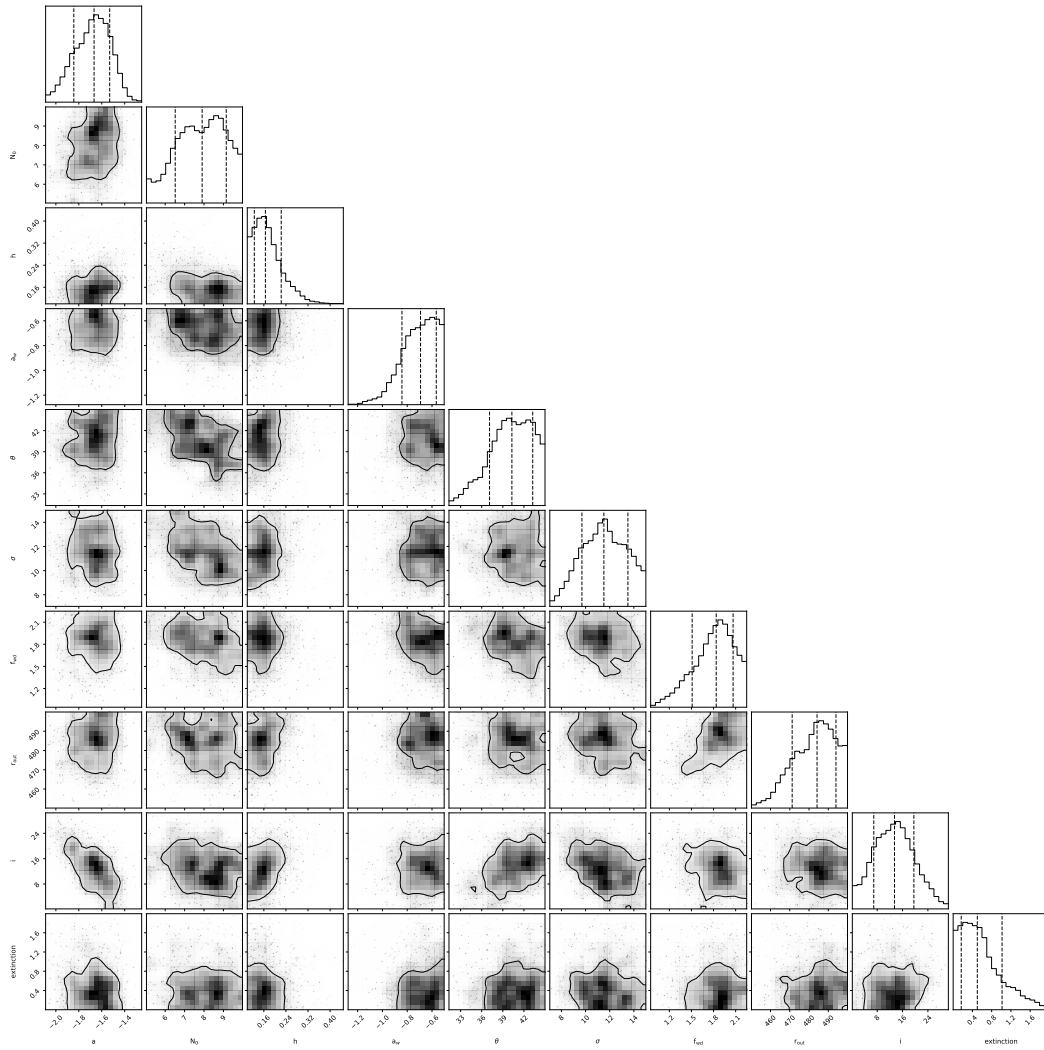
Fig. A.2. 1D and 2D posterior distributions of the model parameters resulting from the fit of J1010 with the disk+wind model of Hönl & Kishimoto (2017). The vertical dashed lines correspond to the percentiles at 16, 50, and 84, whose values are reported in Table 3.
