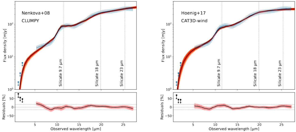
Fig. 2. Smoothed and interpolated nuclear spectrum of J1010, with the emission lines and the PAH features removed (solid blue line), and the best fits with torus models (shaded orange area, which corresponds to model SEDs between the 16 and 84 percentiles of the posterior and solid black line corresponding to the 50 percentile of the posterior). The left panels correspond to the fit with the clumpy torus models of Nenkova et al. (2008a) , and the right panel to the disk + wind models of Hönig & Kishimoto (2017) . Vertical dotted lines are the peak wavelengths measured for the silicate features in the nuclear spectrum (see Table 4). The bottom panels show the residuals as a percentage of the continuum flux, with the horizontal dotted lines indicating 0 and 15% error for guidance. The blue and black upper limits are the J, H, and Ks fluxes from the 2MASS Point Source Catalog (1.69, 3.18, and 6.55 mJy, respectively) and corresponding residuals. These upper limits are shown for comparison only and were not included in the fit.
