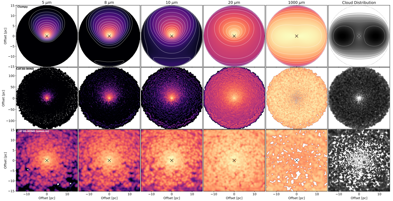
Fig. 3. Model images of the clumpy (top row) and disk + wind (bottom rows) models fit to the nuclear continuum spectrum of J1010 as they would look projected on the sky. The models correspond to the ones described by the parameters of the 50 percentile given in Tables 2 and 3. In the case of the clumpy model, \tau_V = 160 and Y = 20 were used instead of the values shown in Table 2 because the latter are outside the parameter range from which images are computed in HyperCat, but this has negligible impact on torus emission and cloud distribution. The last row is a zoom-in of the disk + wind model showing the same physical region as the clumpy model shown in the top row ( 30 \times 30 \text{ pc}^2 ), since the middle row covers a FOV of 300 \times 300 \text{ pc}^2 . The physical sizes were computed by assuming a bolometric luminosity of 10^{45} \text{ erg s}^{-1} , and in the case of the disk + wind model, a pixel scale = 0.19 \times r_{\text{sub}} , with r_{\text{sub}} = 0.288 \text{ pc} for the largest graphite grains. From left to right, the panels correspond to torus model emission at 5, 8, 10, 20, and 1000 \mu\text{m} , and to the cloud distribution considering all the mass. All the panels are shown in logarithmic color scale and they are normalized to the peak of emission. The black cross in the top and bottom panels indicates the position of the AGN.
