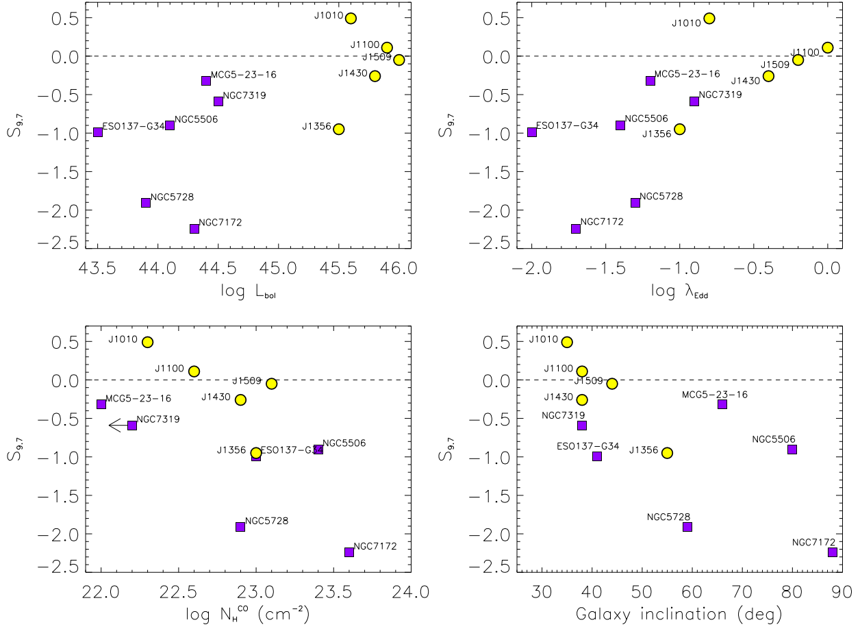
Fig. 4. Strength of the 9.7 \mu\text{m} silicate feature versus the bolometric luminosity, Eddington ratio, gas column density, and galaxy inclination. Yellow circles are the five QSOFEED QSO2s studied in Ramos Almeida et al. (2025) and purple squares the six GATOS Seyfert 2 galaxies from Garca-Bernete et al. (2024a). The horizontal dashed line in all panels indicates the separation between silicate features in absorption (negative values) and in emission (positive values).
