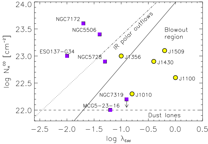
Fig. 5. Column density measured from CO versus the Eddington ratio. The blowout region is where radiation pressure pushes away the obscuring material ( \lambda_{\text{Edd}} > \lambda_{\text{Edd}}^{\text{eff}}(N_{\text{H}}) ), from Ricci et al. (2017). The dot-dashed line from Venanzi et al. (2020) indicates the limit where the AGN radiation acceleration balances gravity and IR radiation pressure dominates, giving rise to polar dusty outflows. The dotted line is an extrapolation of this limit to lower column densities, and the horizontal dashed line is the approximate upper limit for absorption due to dust lanes (Ricci et al. 2017). Yellow circles are the five QSO2s from Ramos Almeida et al. (2025) and purple squares are the Seyfert galaxies from García-Bernete et al. (2024a).
