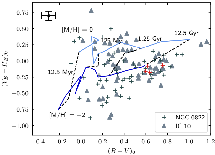
Fig. 10. Reddening-corrected (B - V)_0 vs. (Y_E - H_E)_0 colour-colour diagram of our cluster sample. PARSEC simple stellar populations with [M/H] = -2 and 0 are overplotted (blue lines) with connecting lines of constant age (dashed lines). A subset of the GCs within NGC 6822 for which we have data coverage are indicated in red. Median errors are displayed in the top left-hand corner.
