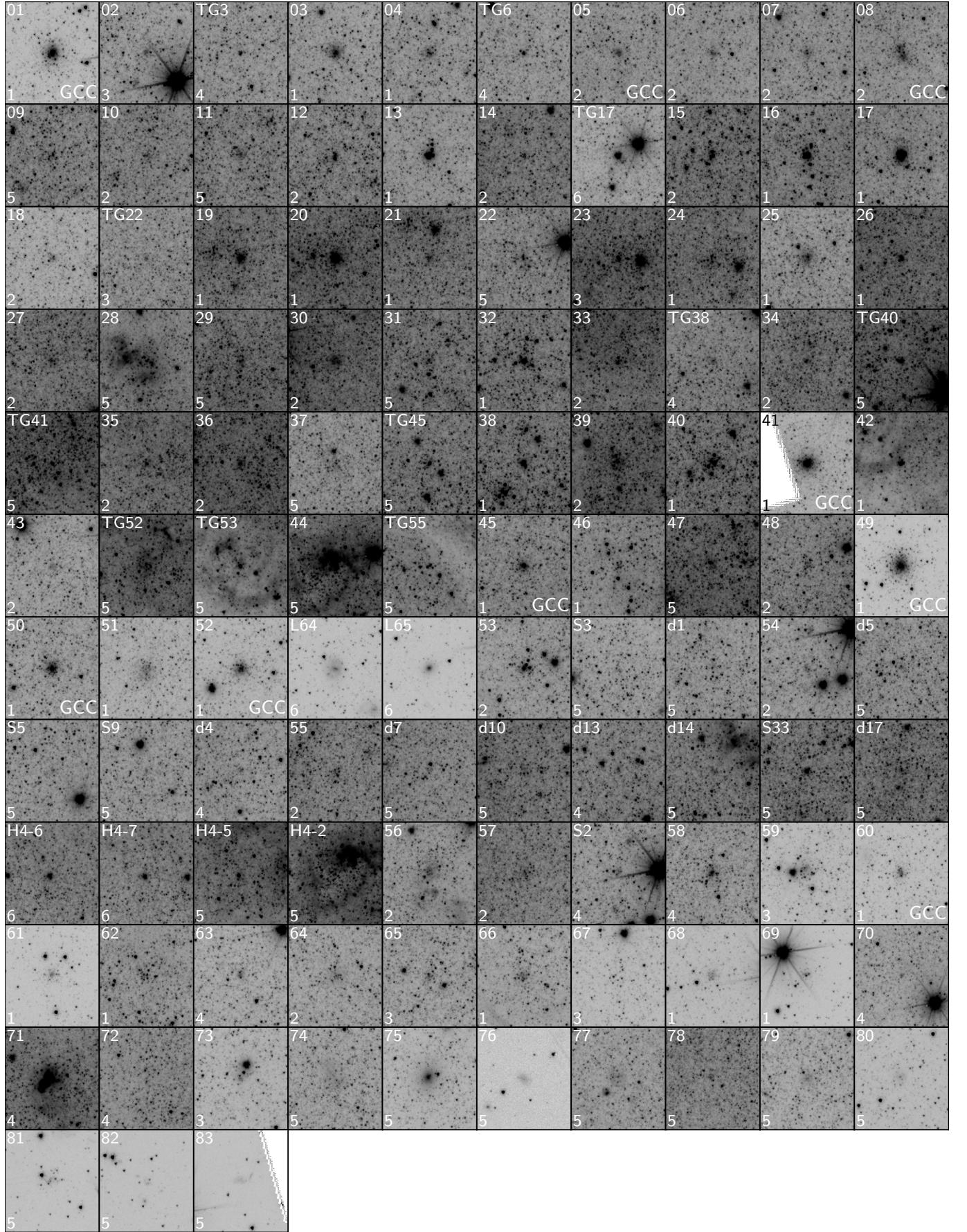
Fig. C.2. Same as Fig. C.1 but for IC 10. New clusters from this study start from Euclid ID 58 onwards. Thumbnails are 18'0 on the side (corresponding to approximately the same physical size as the NGC 6822 thumbnails).
