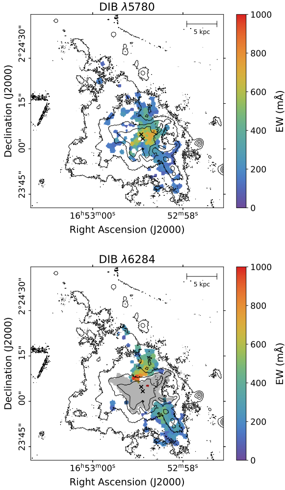
Fig. 5. Maps of detections of DIB \lambda 5780 (top) and DIB \lambda 6284 (bottom). In the bottom panel, the gray area is the region where \text{EW}([\text{O I}]\lambda 6300) \geq 10 \text{ \AA} . The lack of DIB \lambda 6284 detections in these tiles is likely an observational artefact, as the line is blended with the broader [\text{O I}]\lambda 6300 feature. The black contours trace the \text{H}\alpha emission and the black crosses show the locations of the AGNs (Komossa et al. 2003).
