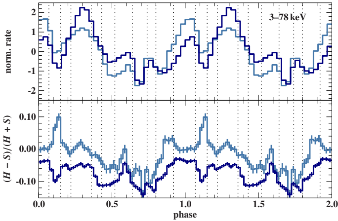
Fig. 5. Comparison of pulse profile and hardness ratio between Obs. I and II. Top: NuSTAR broadband pulse profile for Obs. I (dark blue) and Obs. II (light blue). The pulse profiles are normalized to average zero and units of standard deviation. Dotted lines mark the phase intervals selected for pulse-phase-resolved spectroscopy. Bottom: Hardness ratio of the 3–7 keV and 7–14 keV band, defined as (H - S)/(H + S) . The phase definition is the same as in Paper I.
