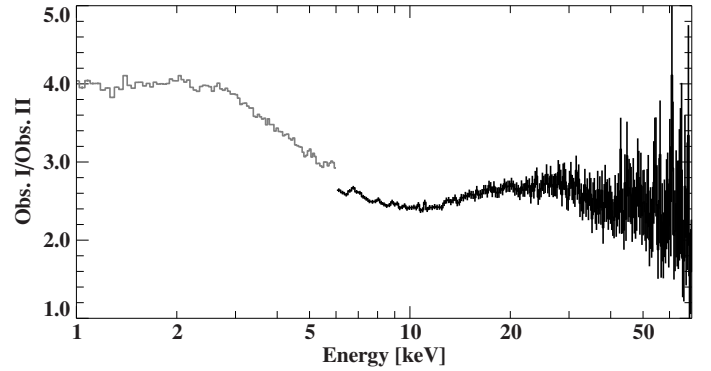
Fig. 2. Energy-resolved count-rate ratio of Obs. I over Obs. II. The gray curve is NICER/XTI; the black one is NuSTAR /FPMA. The offset between NICER and NuSTAR points at flux cross-calibration uncertainties between the instruments.
