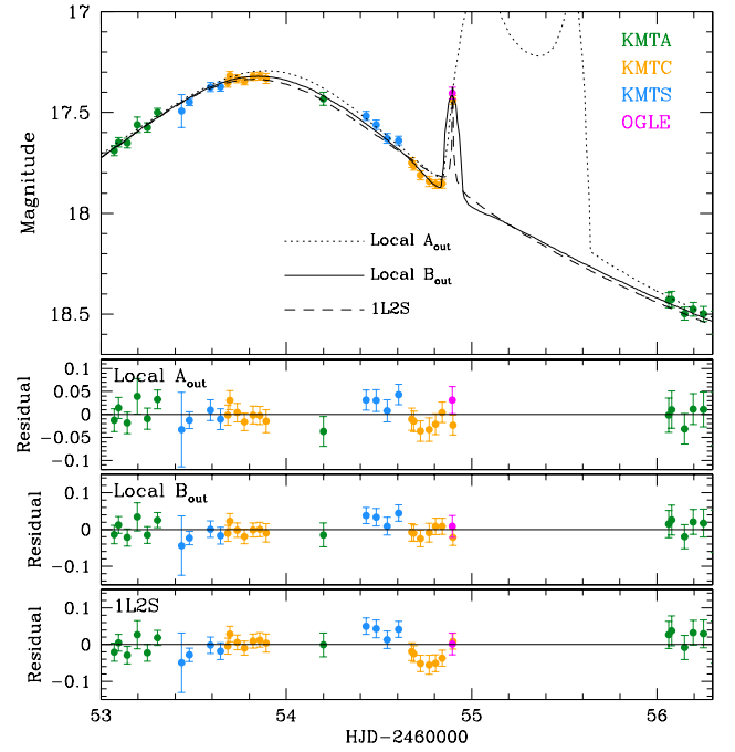
Fig. 4. Model curves of the local solutions A_{\text{out}} and B_{\text{out}} for KMT-2023-BLG-0416. The lower panels show the residuals from the two local planetary solutions and the single-lens binary-source (1L2S) solution.
