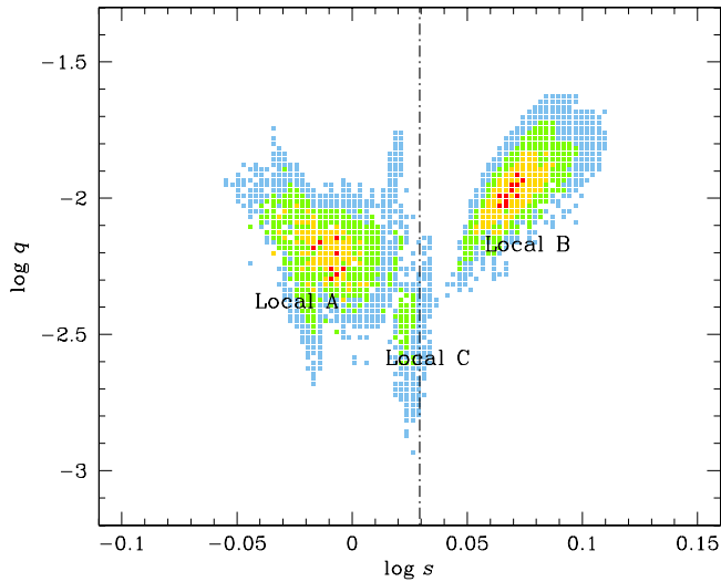
Fig. 11. \Delta\chi^2 map in the (\log s, \log q) parameter plane of KMT-2023-BLG-1642. The color coding is set to represent points with \leq 1\sigma (red), \leq 2\sigma (yellow), \leq 3\sigma (green), and \leq 4\sigma (cyan), where n = 3 .
