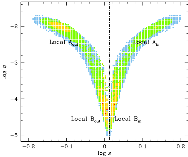
Fig. 3. \Delta\chi^2 map on the plane of the planet parameters ( \log s, \log q ) of the lensing event KMT-2023-BLG-0416. The color scheme represents points with \Delta\chi^2 < 1^2 n (red), < 2^2 n (yellow), < 3^2 n (green), and < 4^2 n (cyan), where n = 2 . The labels marked by A_{\text{in}} , A_{\text{out}} , B_{\text{in}} , and B_{\text{out}} represent positions of the four local solutions. The vertical dot-dashed line indicates the geometric mean between the binary separations of the B_{\text{in}} and B_{\text{out}} solutions.
