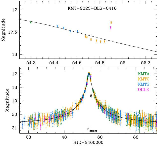
Fig. 2. Lensing light curve of KMT-2023-BLG-0416. The lower panel presents the overall perspective, while the upper panel provides a close-up view of the anomaly region. The arrow in the lower panel indicates the time of the anomaly. The curve drawn over the data points is a 1L1S model obtained by fitting the light curve with the exclusion of the data around the anomaly.
