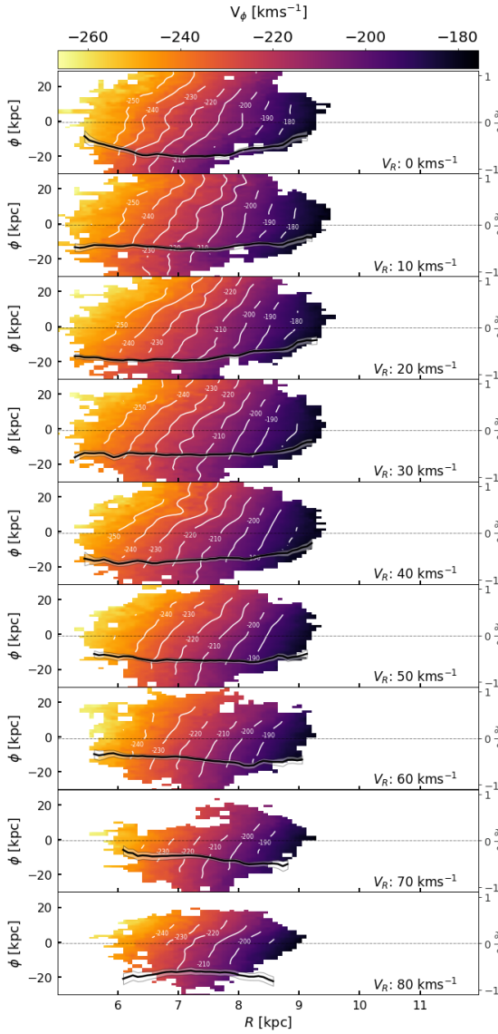
Fig. C.1. Mean azimuthal velocity of the groups in Hercules in the R - \phi projection, for |Z| < 0.2 kpc. The contours of regions with the same velocity are shown for clarity (in white). The slope of the linear fitting ( \phi, V_\phi ) is shown (in black) for every R column, in units of [\text{km s}^{-1} \text{ deg}^{-1}] . The 3\sigma error of the slope is shown in a translucent region around the line. The group has the same slope at all V_R . This corresponds to a vertical displacement of the moving group in the V_R - V_\phi diagram.
