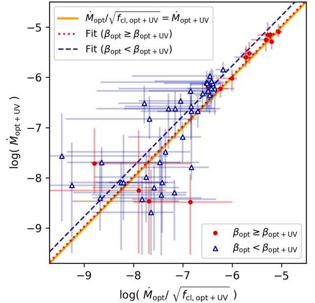
Fig. D.3. Comparison of the mass-loss rates derived from the optical + UV data, versus those of the optical-only data (fitted assuming a smooth wind) corrected for clumping using the individual f_{\text{cl}} values obtained from our optical + UV fits. The difference between the two seems to be related to different values of \beta (see text).
