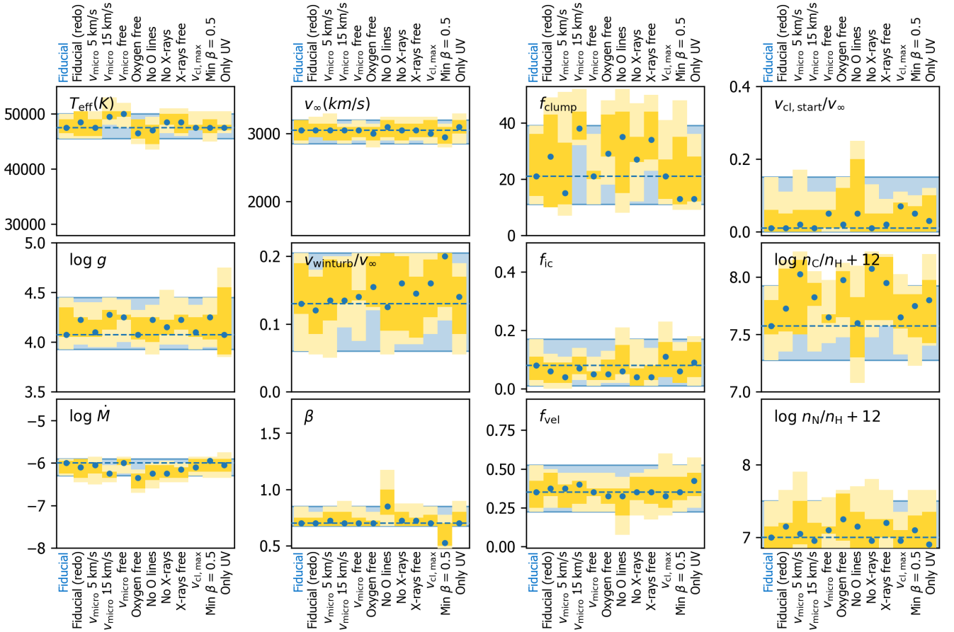
Fig. 11. Comparison of parameters from the different test runs, fitting in each instance the spectrum of H35. For each run and each parameter we indicate the best fit value (blue dots) and 1 and 2\sigma error bars (dark and light yellow). In the first column we show the parameters of our ‘fiducial run’: this is the setup as used throughout the paper. The other columns show parameters of runs where we changed the setup, one aspect at the time: ‘Fiducial (redo)’ – different initial random population of models, ‘ v_{\text{micro}} 5 \text{ km s}^{-1} ’ and ‘ v_{\text{micro}} 15 \text{ km s}^{-1} ’ – assumed value for v_{\text{micro}} to 5 and 15 \text{ km s}^{-1} , respectively, instead of 10 \text{ km s}^{-1} , ‘ v_{\text{micro}} \text{ free} ’ – v_{\text{micro}} a free parameter, ‘Oxygen free’ – oxygen abundance a free parameter, ‘No O lines’ – exclude both O IV \lambda 1340 and O V \lambda 1371 from the fitting, ‘No X-rays’ – do not include any X-rays, ‘X-rays free’ – f_X a free parameter, ‘ v_{\text{cl,max}} ’ – assume v_{\text{cl,max}} = 2v_{\text{cl,start}} instead of v_{\text{cl,max}}/v_{\infty} = \max(0.3, v_{\text{cl,start}}/v_{\infty}) , ‘Min \beta = 0.5 ’ – set lower limit of \beta to 0.5 instead of 0.7 and ‘Only UV’ – only fit the UV spectra. For reference, the best fit value and 2\sigma error region of the fiducial run are shown in blue throughout all columns.
