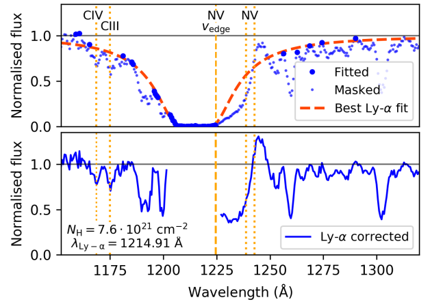
Fig. 3. Ly- \alpha fitting procedure for H35. Upper panel: original data (blue: flux points indicated with a large dot are considered in the fit, small ones are not) and the best fit Ly- \alpha profile (orange dashed line). Lower panel: Ly- \alpha corrected flux and the values of N_{\text{H}} and \lambda_{\text{Ly-}\alpha} used for the correction. Indicated with vertical lines are the rest wavelengths of transitions of diagnostic lines (yellow dotted) and the position of the edge of the N V \lambda 1240 line (yellow dashed).
