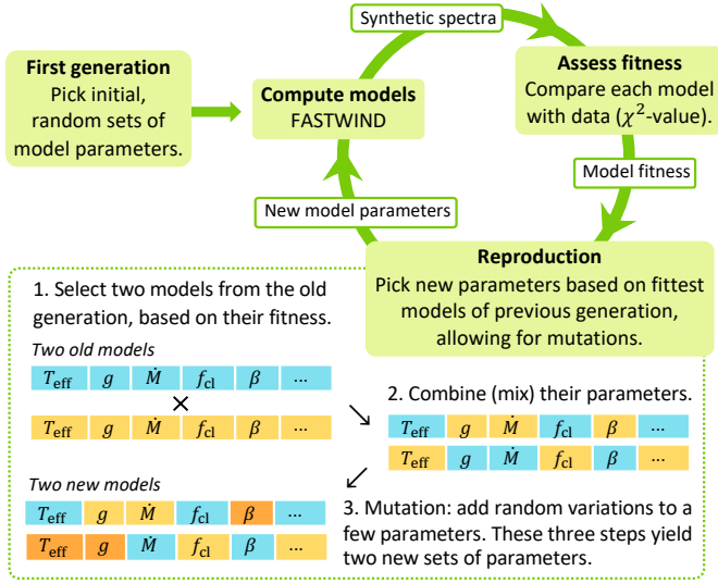
Fig. 6. Flowchart portraying the workings of KIWI-GA. In each generation, depicted by the green circle with arrows, a large amount of models is computed (typically 50–250). The reproduction step is a means of natural selection towards fitter models, which eventually leads to convergence of the algorithm towards the best fitting solution (typically after 30–100 generations).
