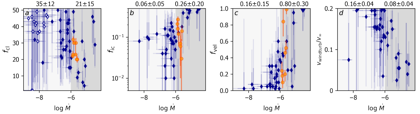
Fig. 16. Wind structure parameters plotted against mass-loss rate of stars in R136 (blue diamonds, dark and light shaded error bars denote 1\sigma and 2\sigma uncertainties) and eight Galactic stars of the sample of Hawcroft et al. (2021) , orange circles, 2\sigma uncertainties). The limits of the y -axis of each plot coincide with the range of values that was allowed during the fit. The panels a – d show, from left to right, the clumping factor, the interclump density contrast, the vorosity and the wind turbulence. At the top of each panel the average value of the parameter ( \pm 1\sigma uncertainty) is quoted for two \dot{M} regimes: low ( \log \dot{M} < -6 , light grey shaded) and high ( \log \dot{M} > -6 , dark grey shaded). In the leftmost panel, the diamonds with a white interior denote sources that are not present in the other three panels, as the f_{ic} , f_{vel} and v_{windturb} values were not fitted in their optical + UV runs. No values of Hawcroft et al. (2021) are shown in the rightmost panel, as they do not fit v_{windturb} .
