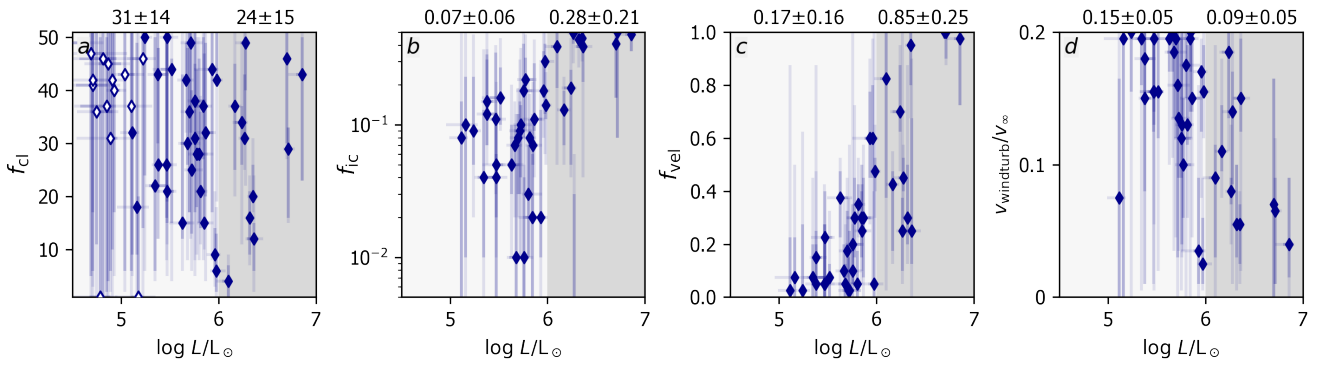
Fig. H.2. As Fig. 16 but as a function of L/L_{\odot} . The cutoff value for the ‘low’ and ‘high’ regime is at \log L/L_{\odot} = 6 .
