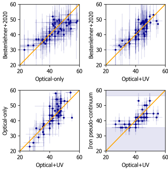
Fig. D.2. Comparison of different temperature analyses in units of 1000 K. Top: the optical-only analysis of Bestenlehner et al. (2020) against our optical-only (left) and our optical + UV analysis (right). Bottom: our optical-only (left) and our iron pseudo-continuum analysis (right) against our optical + UV analysis. The shaded area in the bottom right plot indicates the region that is not covered by the CMFGEN grid that we used (Bestenlehner et al. 2014).
