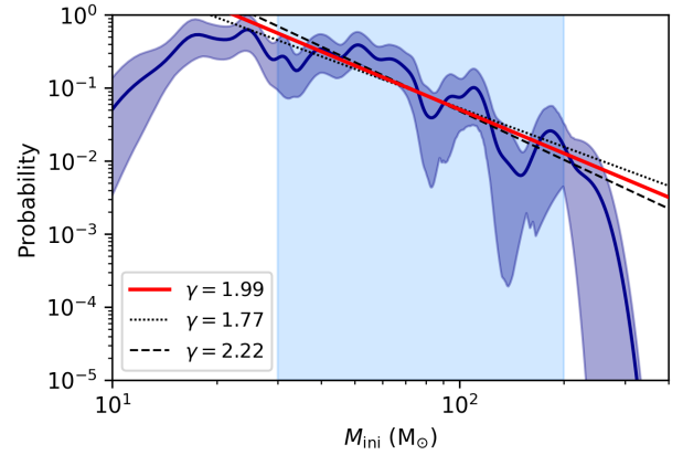
Fig. E.3. Distribution of initial masses of stars in the core of R136, as found using BONNSAI. The dark blue solid line and the shaded area around it are the observed distribution and bootstrapped 2\sigma uncertainties. Red solid line is the best power law fit over the region 30-200 M_{\odot} (light blue background), black dashed and dotted line represent 2\sigma uncertainty on the slope.
