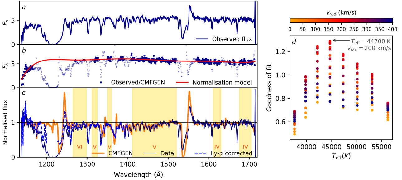
Fig. 2. UV normalisation and T_{\text{eff}} fitting procedure for H35. Left panels: (a) the observed flux in units of 10^{-14} \text{ ergs cm}^{-2} \text{ s}^{-1} \text{ \AA}^{-1} , (b) the observed flux divided by the normalised CMFGEN model (dark blue points, masked points are shown semi-transparent) and a fit through the non-masked points (red solid line), and (c) the normalised spectrum (dark blue solid line), the normalised, Ly- \alpha corrected spectrum (blue dashed line) and the CMFGEN model used for obtaining the normalisation model (solid orange line). The yellow shaded areas indicate the regions used for determining the goodness of fit of the iron pseudo-continuum of the model; roman numerals indicate the dominant iron ion in each region. Right panel: for each model T_{\text{eff}} and v_{\text{rad}} the dimensionless goodness of fit to the normalised iron pseudo-continuum of the data (defined as the inverse of the squared sum of the difference between the normalised fluxes of the model and the data in the iron continuum). At the peak lie the T_{\text{eff}} and v_{\text{rad}} that give the best fit: these are the values that are used for the final normalisation shown on the left.
