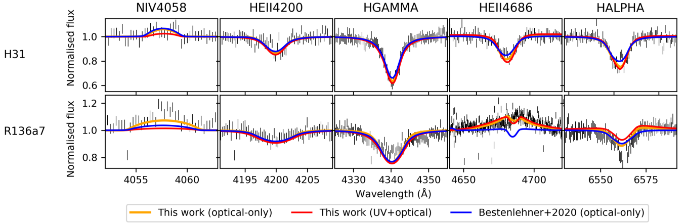
Fig. D.1. Comparison of optical lines of fits obtained with different methods. The top row shows lines of H31, for which the parameters of Bestenlehner et al. (2020) and this work agree well: this level of agreement is representative for most stars in the sample. The bottom row shows lines of R136a7, where there is some discrepancy between the parameters of Bestenlehner et al. (2020) and our results. The difference is especially clear in He II \lambda 4686 , and seems related to differences in T_{\text{eff}} and \dot{M} .
