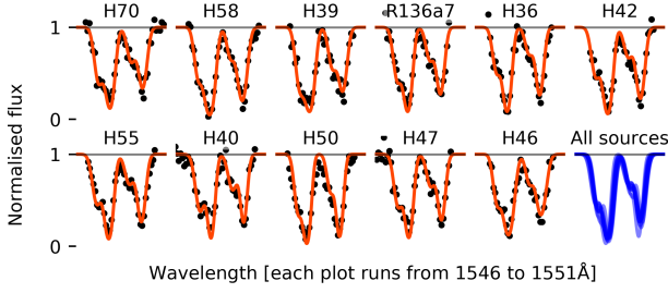
Fig. 4. Best fits of the interstellar C IV \lambda\lambda 1548 – 1551 lines for all sources of de Koter et al. (1998) . For each source we show the normalised flux of the interstellar lines (black dots) and the best fit (orange lines). The last panel contains the best fit of all sources (blue lines).
