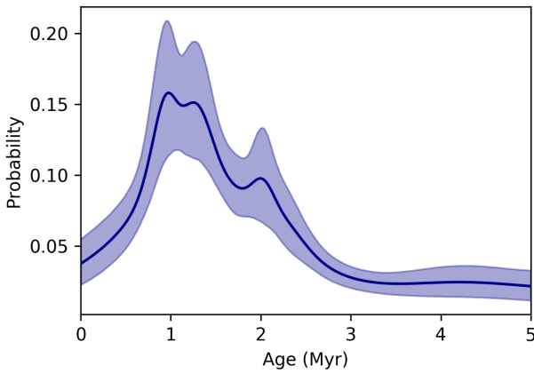
Fig. E.2. Age distribution of stars in the core of R136, as found using BONNSAI. The dark blue solid line and the shaded area around it are the observed distribution and bootstrapped 2\sigma uncertainties.
