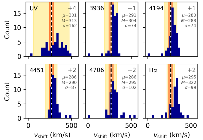
Fig. B.2. Distribution of measured wavelength corrections v_{\text{shift}} in \text{km s}^{-1} , for each grating (dark blue). We indicate the mean R136 velocity of 267.7 \text{ km s}^{-1} as measured by Hénault-Brunet et al. (2012, black dashed lines), together with the non-binary-corrected velocity dispersion of \sigma = \pm 25 \text{ km s}^{-1} (orange-red shaded), as well as a velocity range corresponding \pm 2 pixels around the R136 mean (yellow shaded). The numbers in the upper right corner of each plot denote the amount of stars that fall out of the plotted velocity range. Below that, we show the inferred mean \mu , median M and standard deviation \sigma of each grating (all in \text{km s}^{-1} ).
