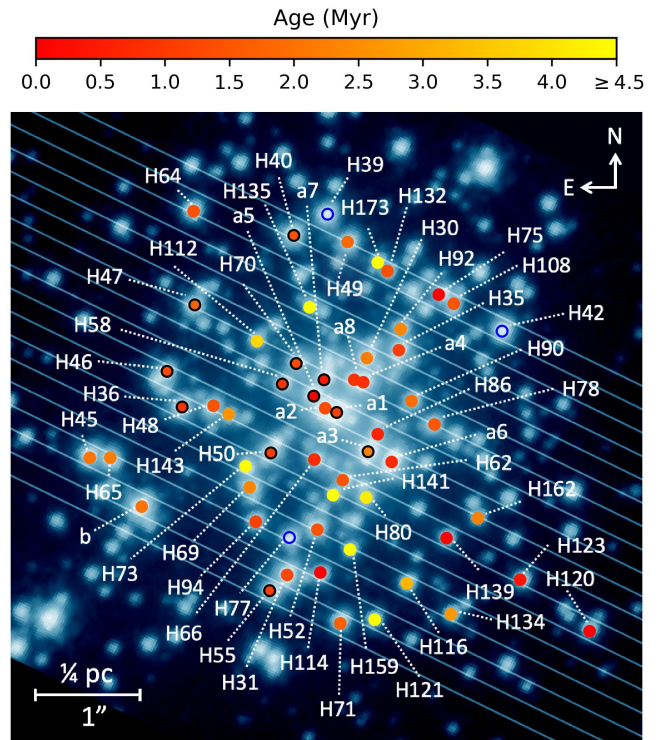
Fig. E.4. As Fig. 1, but colour coding by stellar age instead of mass.
