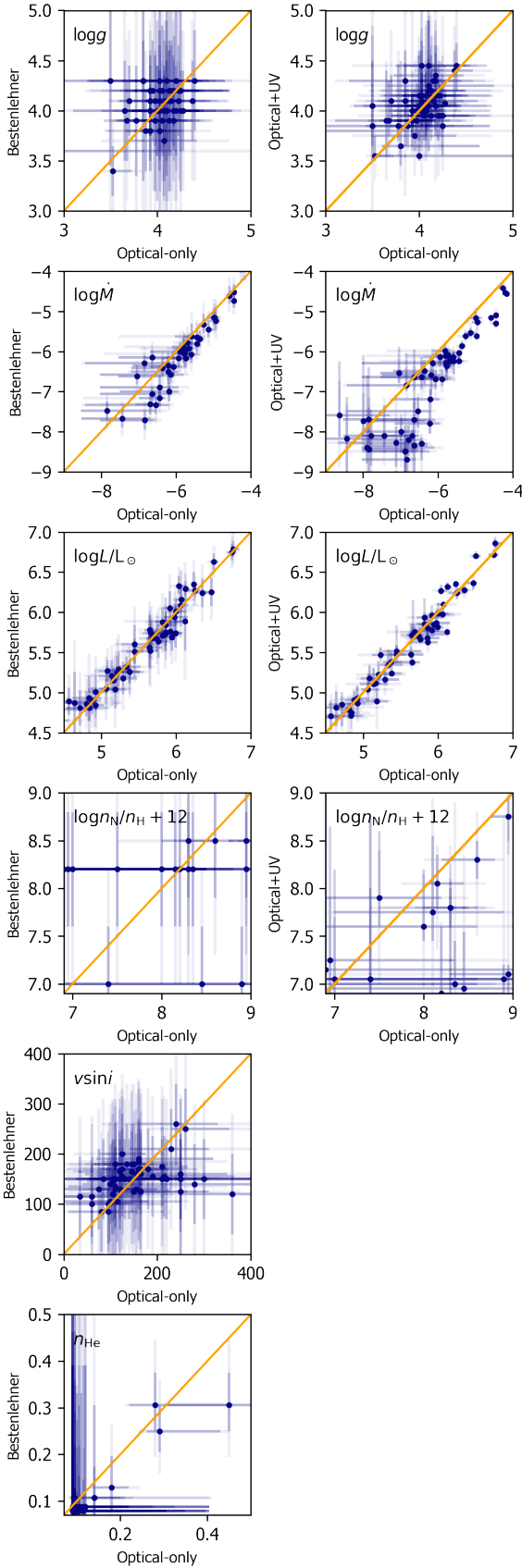
Fig. D.4. Comparison of different analyses. Left column: optical-only analysis with KIWI-GA (this work) against the optical-only analysis with IACOB-GBAT (Bestenlehner et al. 2020), right column: optical-only analysis with KIWI-GA vs. optical + UV analysis with KIWI-GA (both this work).
