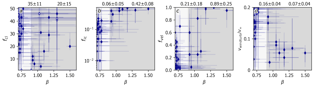
Fig. H.3. As Fig. 16 but as a function of \beta . The cutoff value for the ‘low’ and ‘high’ regime is at \beta = 0.9 .
