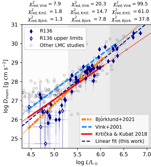
Fig. 13. As Fig. 12 but now for the modified wind momentum. In grey circles we show the values or upper limits of Mokiemi et al. (2007); Bestenlehner et al. (2014); Ramírez-Agudelo et al. (2017); Sabín-Sanjulián et al. (2017), which we all lowered by 0.7 dex, assuming f_{\text{cl}} = 25 .
