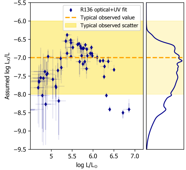
Fig. G.1. Left: L_X/L against L of our best fitting models (dark blue diamonds with 2\sigma error bars). Right: Distribution of the L_X/L values from our best fitting models. We indicate the typical observed value of L_X/L (orange dashed line) and the typical scatter around this value (yellow band). We stress that the X-ray luminosity L_X/L is not a free parameter in our fitting and the L_X/L values shown here do not represent the actual X-ray flux of the given stars: this plot serves solely as a check on our assumptions (see text).
