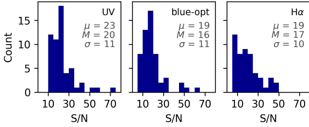
Fig. B.1. S/N distribution for each wavelength range: UV (left), blue-optical (middle) and H \alpha (right). Mean \mu , median M and standard deviation \sigma are given for each range.
