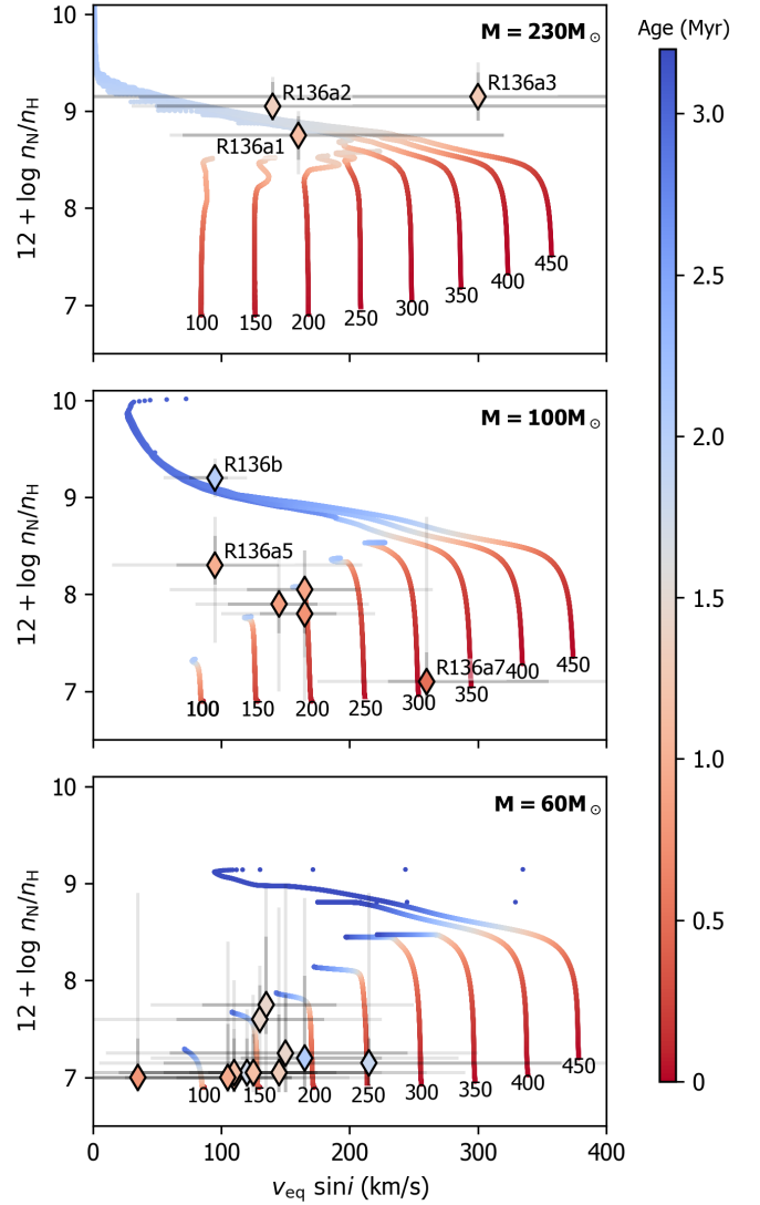
Fig. 20. Hunter diagrams, showing stellar age (red to blue colour bar) as a function of rotation and nitrogen surface abundance. Evolutionary tracks are taken from Köhler et al. (2015) and depict the evolution of stars with an initial mass of 230 M_\odot (top), 100 M_\odot (centre), and 60 M_\odot (bottom) with a range of initial rotation rates. We note that the theoretical rotation rates are scaled by \pi/4 to correct for the average projection angle, and that the tracks are cut off at T_{\text{eff}} < 29\,000 \text{ K} . The diamond markers indicate the observed positions of sources in the respective mass-regimes, where their colour maps to age via the same coding as the tracks. For a discussion on the error bars on the observed rotation rates of the WNh stars, see text.
