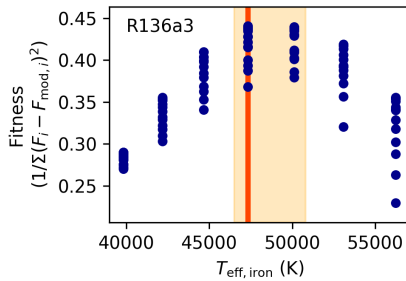
Fig. F.2. Fitness distribution of the iron pseudo-continuum fit of R136a3. The best fitting temperature (47315 K) is indicated. A temperature of 50000 K results in about the same fitness. The fitness is comparable to the inverse of a \chi^2 : it is the inverse of the sum of the square of the residuals. The residuals are the difference between the normalised observed flux F_i and model flux F_{\text{mod},i} , for all flux points of the iron pseudo-continuum.
