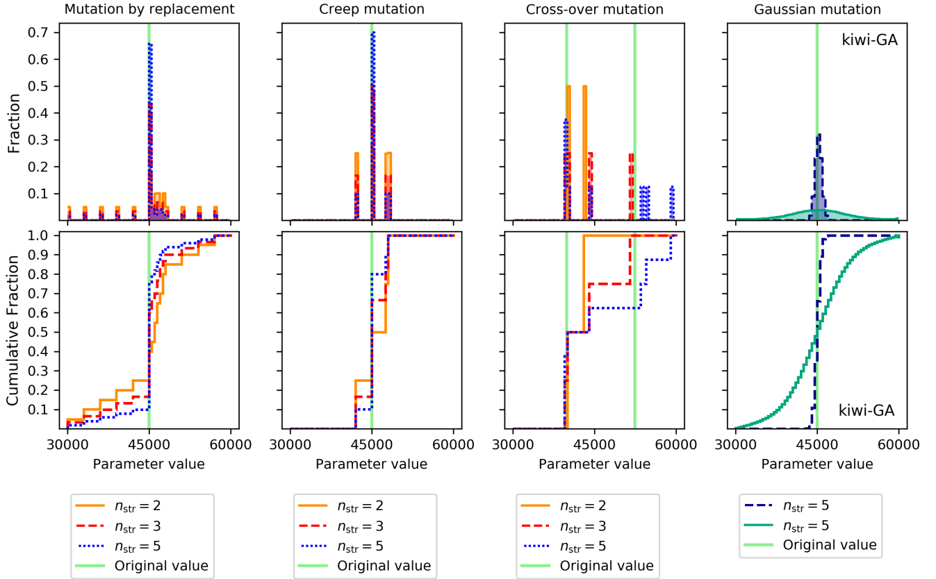
Fig. B.3. Distribution (top panels) and cumulative distribution (bottom panels) of mutation sizes of different schemes. The panels in the first three columns on the left show the behaviour of different types of mutation that result from modifying strings that represent the parameters in three different ways: by replacing one string digit by a random other digit (mutation by replacement), by increasing or decreasing the value of one string digit with 1 (creep mutation), and by changing one or more digits of a string by slicing it during the recombination process (cross-over mutation). The green vertical line indicates the original value of the parameter (in the third panels from the left this are two lines: one for each parent), in orange, red and blue the distribution of parameter values after the mutation has taken place. The different colours refer to the amount of digits that decode one parameter. The rightmost panels show the behaviour when the mutation size is described by a Gaussian distribution, as is the case in KIWI-GA.
