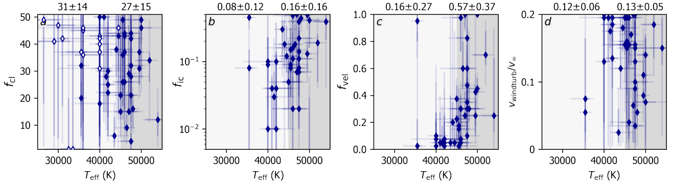
Fig. H.1. As Fig. 16 but as a function of T_{\text{eff}} . The cutoff value for the ‘low’ and ‘high’ regime is at T_{\text{eff}} = 45000 K.
