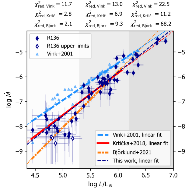
Fig. 12. Mass-loss rates from the optical + UV fits (dark blue solid diamonds) compared to the mass-loss predictions of Vink et al. (2001, light blue triangles), Krtićka & Kubát (2018, red solid line) and Björklund et al. (2021, orange dot-dashed line). The prescription of Vink et al. (2001) depends on more parameters than luminosity; a linear fit through the individual points (light blue dashed line) is plotted to guide the eye. Thin dotted lines in corresponding colours show the extrapolation of each prescription beyond the coverage of their respective model grids. For reference, a linear fit through the data points is shown (thin dashed dark blue line). For all mass-loss prescriptions we assess the goodness of fit ( \chi^2 -values, top) for three ranges of luminosity.
