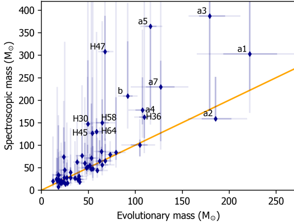
Fig. E.1. For more massive stars spectroscopic masses are systematically larger than evolutionary masses.
