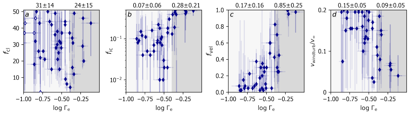
Fig. H.4. As Fig. 16 but as a function of \log \Gamma_{\text{Edd},e} . The cutoff value for the ‘low’ and ‘high’ regime is at \log \Gamma_{\text{Edd},e} = -0.40 corresponding to \Gamma_{\text{Edd},e} = 0.40 . We note that \Gamma_{\text{Edd},e} is proportional to T_{\text{eff}}^4/g .
