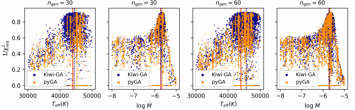
Fig. B.4. Comparison of the fitness distributions of T_{\text{eff}} and \log \dot{M} of two genetic algorithm runs. The dark blue points show the models of a Kiwi-GA run, the yellow points the models of a pyGA run. Setup of the runs was identical: both runs had the same data (FASTWIND model with simulated S/N of 30), parameter space, number of individuals, and number of generations. The left two plots show the run states after 30 generations, the right two plots after 60 generations. The ‘true values’, that is, the value of the model used for simulating the data, is indicated with a red line. Dark blue and yellow dotted lines indicate the best fit models.
