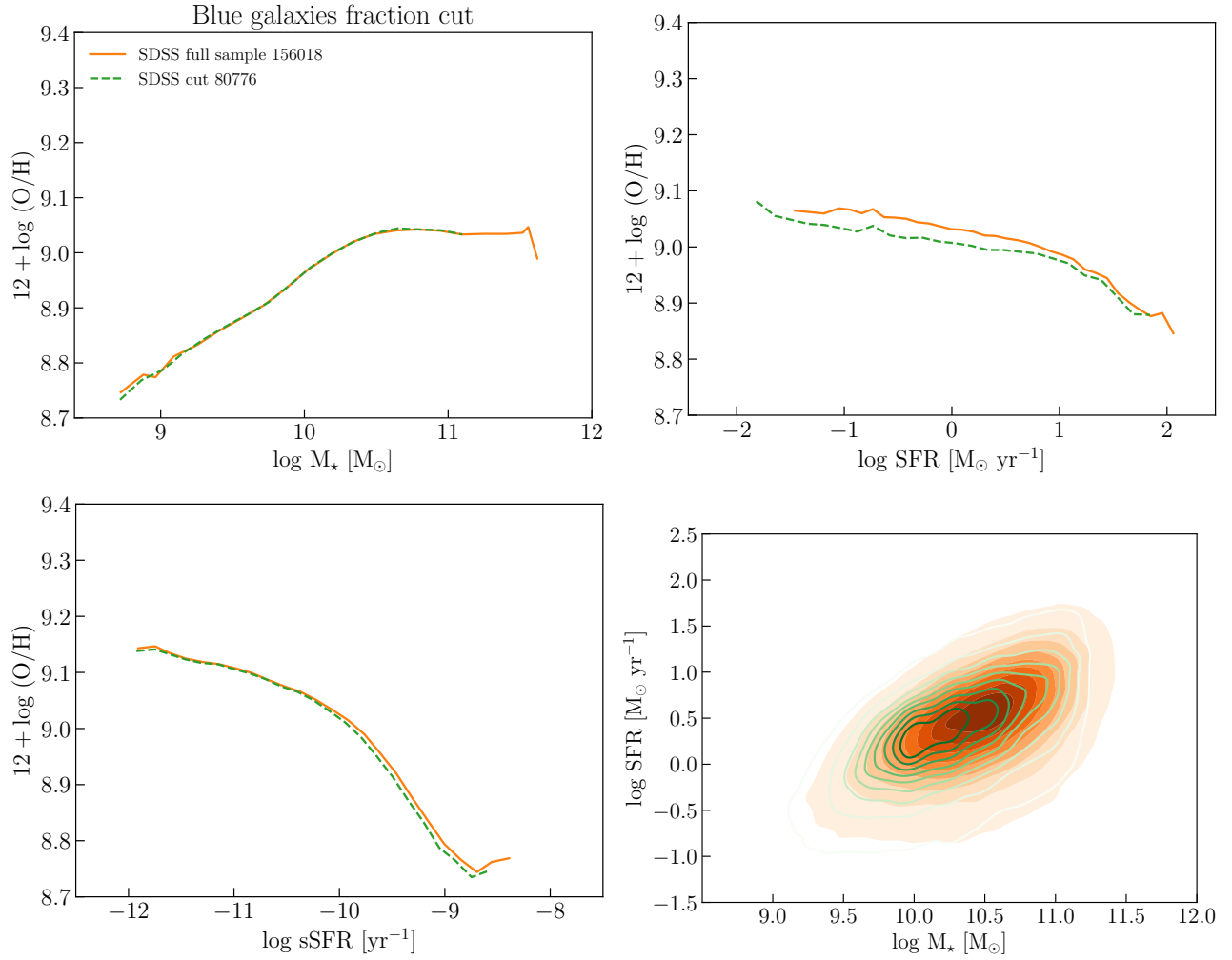
Fig. 12. Effects of the fraction of blue galaxies on the projections of the FMR (full sample: orange solid line; same fraction on M_* than VIPERS: green dashed line).
