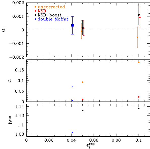
Fig. 8. Top panel: multiplicative bias of galaxies with 20 < m_r < 24.5 after METADETECTION for simulated ground-based observations with a PSF that follows a Moffat profile with \text{FWHM} = 0''.7 . Middle panel: residual additive bias c_i , if we do not correct the polarisations (orange) or use the standard KSB correction (red). Bottom panel: best estimate for b^{\text{sm}} as a function of \epsilon_i^{\text{PSF}} . The blue points shows the results for a double Moffat profile with a large ellipticity gradient (see Sect. 5 for details). Also for this more complex PSF do we find a multiplicative bias that is consistent with zero.
