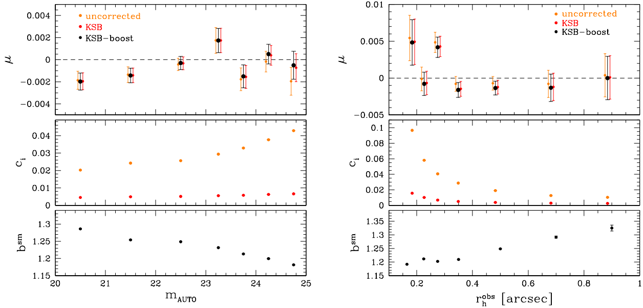
Fig. 4. Left panel: residual multiplicative bias ( top ), additive bias ( middle ) and estimate for b^{\text{sm}} ( bottom ) as a function of observed magnitude, m_{\text{AUTO}} , determined by SEXTRACTOR. Right panel: idem, but as a function of the observed half-light radius, r_h^{\text{obs}} . The orange points indicate the biases when the polarisations are not corrected for PSF anisotropy, whereas the red points are for the standard KSB correction. The black points use b^{\text{sm}} to correct for PSF anisotropy, resulting in vanishing additive bias by construction (and therefore not shown).
