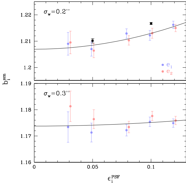
Fig. 3. Correction factor b_1^{\text{sm}} as a function of PSF ellipticity for a weight function \sigma_w = 0''.2 (top) and \sigma_w = 0''.3 (bottom). The red and blue points show the results for the individual shear components using the grid-based simulations. The lines are the best-fit model (see text) to both components jointly. The bias is smaller overall for the larger weight function, whilst the dependence with PSF ellipticity is also reduced. The black squares in the top panel correspond to our baseline setup, with galaxies placed randomly. This suggests that blending has a small impact on the correction.
