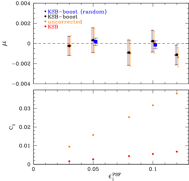
Fig. 2. Multiplicative bias, \mu (top) and additive bias, c_i (bottom) after METADTECTION, as a function of PSF ellipticity, \epsilon_i^{\text{PSF}} , for galaxies with 20 < m_{\text{VIS}} < 24.5 that were placed on a grid. The orange points correspond to the results without correction for PSF anisotropy, whereas the red points indicate the biases after the nominal KSB correction ( b^{\text{sm}} = 1 ). The black points show the results using the value for b^{\text{sm}} that nulls the additive bias for the grid-based simulations, whereas the blue squares correspond to our baseline setup, where galaxies were placed randomly (see Sect. 4.2; in this case the error bars are smaller, because we simulated more images for the baseline case). We do not show the corresponding additive biases, because those are consistent with zero by construction.
