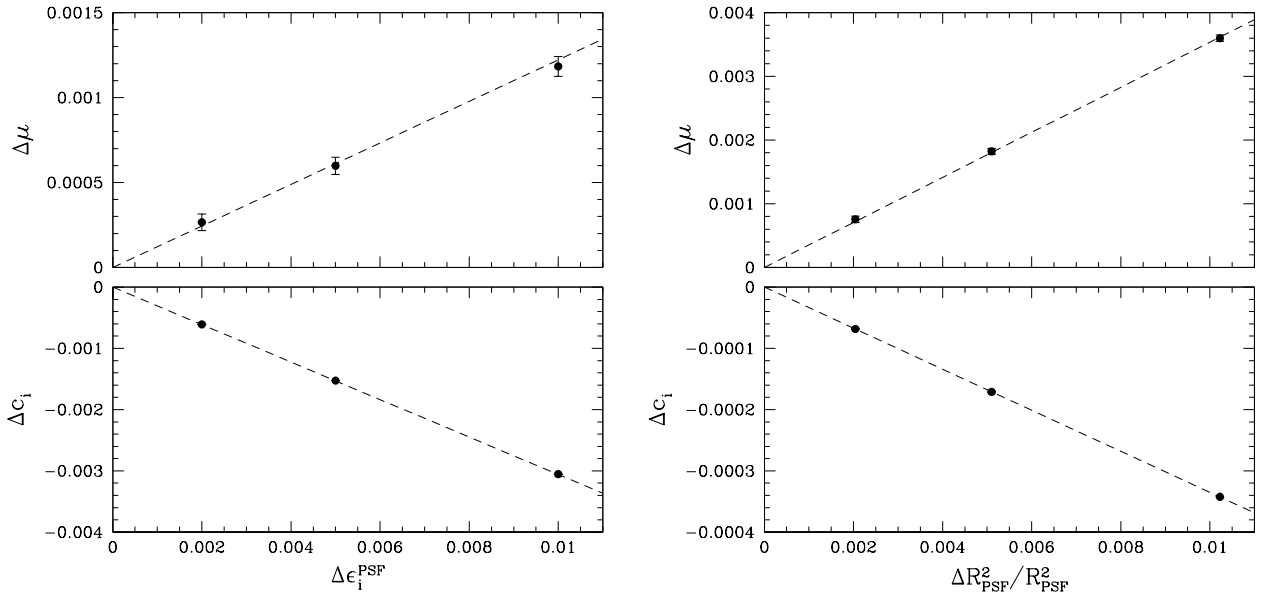
Fig. 7. Left: change in multiplicative bias ( top ) and additive bias ( bottom ) as a function of \Delta\epsilon_i^{\text{PSF}} , the error in PSF ellipticity. Right: idem, but when the size of the PSF is changed isotropically. The relative change in size is quantified by \Delta R_{\text{PSF}}^2 / R_{\text{PSF}}^2 , computed using the PSF quadrupole moments. In both cases, the multiplicative and additive biases increase linearly with the PSF error, but we note the different scales: The multiplicative bias is more sensitive to size errors, whereas the additive bias is most sensitive to errors in the PSF ellipticity.
