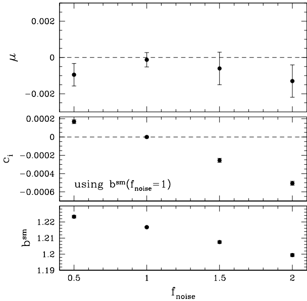
Fig. 5. Top panel: multiplicative bias after METADETECTION for galaxies with 20 < m_{\text{VIS}} < 24.5 when the noise is increased by a factor of f_{\text{noise}} with respect to the baseline case, with \epsilon_{\text{PSF}} = 0.1 . Middle panel: residual multiplicative bias c_i ; if we use b^{\text{sm}} = 1.217 , the estimate for the baseline case. Bottom panel: best estimate for b^{\text{sm}} as a function of f_{\text{noise}} , which shows a clear dependence on the noise level. If ignored, the residual multiplicative biases exceeds Euclid requirements for this level of PSF anisotropy.
