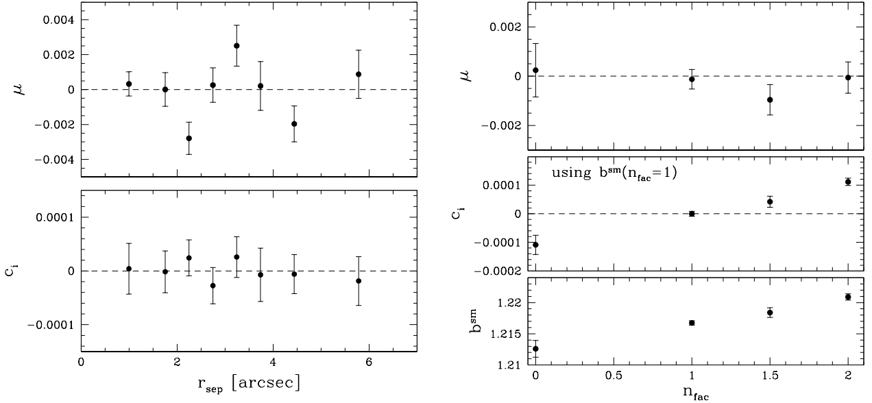
Fig. 6. Left panel: residual multiplicative bias ( top ) and additive bias ( bottom ) as a function of r_{\text{sep}} , the distance to the nearest galaxy in the input catalogue brighter than m = 26 . Right panel: residual biases as a function of n_{\text{fac}} , the relative increase in galaxy density, where n_{\text{fac}} corresponds to the grid-based case. In both cases, results were obtained using b^{\text{sm}} = 1.217 , the best estimate for the fiducial setup. The results indicate that the performance is not affected significantly by blending, although the additive biases exceed Euclid requirements for extreme over- and under-densities.
