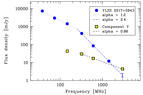
Fig. 7. Spectrum of VLSS J2217.5+5943, i.e., components II–IV (blue) and component V (dark yellow). Data are from the 8C catalog (38 MHz), VLSS (74 MHz), TGSS ADR (150 MHz), GMRT 325 MHz and 610 MHz, WSRT (1.4 GHz), and VLASS (3 GHz). The upper limit from VLASS corresponds to the 68 % confidence limit.
