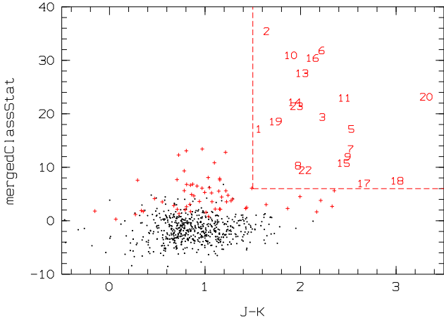
Fig. 2. Morphology-color diagram for 658 UKIDSSDR11PLUS sources with J < 19.5 and K < 19.5 in the 24 square arcmin field around VLSS J2217.5+5943. The color index J-K is computed from the Petrosian magnitudes. Black and red symbols indicate sources classified as star-like or as galaxies, respectively. The dashed lines mark the selection area for the galaxies in the present study.
