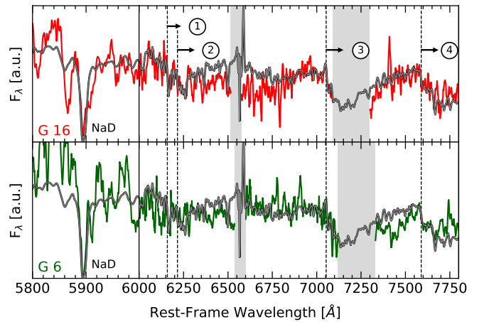
Fig. 5. Red to far-red spectra of galaxies G16 (red) and G6 (green) and of an elliptical template spectrum (gray) from 5800 to 7800 Å (rest frame). The NaD absorption and the band heads of TiO at \lambda 6158 (1), \lambda 6216 (2), \lambda 7053 (3), and \lambda 7589 (4) are marked. The region around the [N II] and H\alpha emission complex of the template galaxy is shaded in gray because it coincides with the strong telluric A-band (7590–7660 Å) in the observed frame. A region around 7200 Å corresponding to roughly 8370 Å in the observed frame, which is close to the wavelength of the dichroic filter transition between the two channels and is also contaminated by night-sky emission lines, is also shaded in gray.
