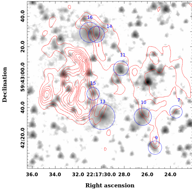
Fig. 9. 610 MHz contours (as in Fig. 8) plotted over the IRAC I1+I2 stacked image.
