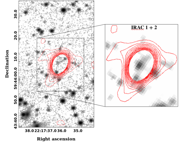
Fig. 11. Infrared counterpart of the compact radio source J221736.2+594407 (red contour lines) on the UGPS JHK image (left) and the IRAC 1+2 stack (right). Only the outer radio contours are plotted in order to show the NIR sources at the 610 MHz peak position (lowest contour at 3\sigma local background, followed by steps of 5\sigma ).
