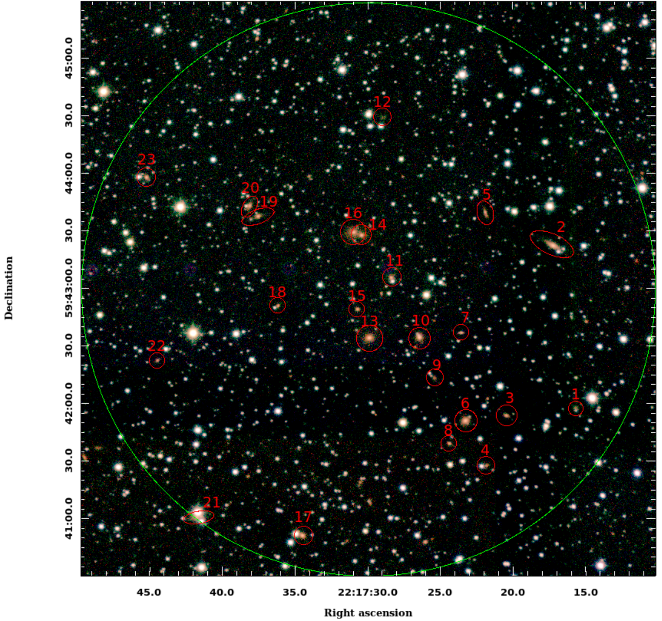
Fig. 1. RGB composite of the central 5' \times 5' field around the position of the radio source 24P73 ( 22^{\text{h}}17^{\text{m}}5 + 59^{\circ}43' , J2000) from the UGPS J , H , and K images. The green circle marks the selection area. Selected galaxies are indicated by their red color and numbered in order of increasing RA.
