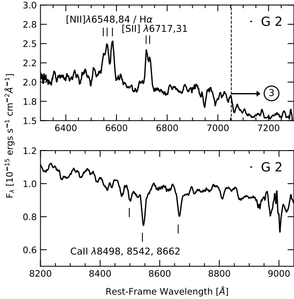
Fig. 6. Sections around the H \alpha region and the TiO \lambda 7053 band head (3), as well as around the Ca II infrared triplet of G2.
