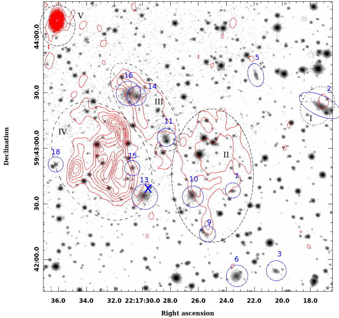
Fig. 8. 2'6 \times 2'6 field containing both the radio source 24P73 and the central part of the galaxy concentration with the brightest galaxies, G2, G6, G13, and G16. Galaxies are indicated by their blue color. The inverted grayscale background image is the stack of the J -, H -, and K -band images from UGPS. The red curves are the contour lines of the GMRT 610 MHz radio map (lowest level at 3\sigma , all others in steps of 5\sigma with \sigma = 55 \mu\text{Jy} ). Dashed black ellipses mark the five radio components, labeled with Roman numerals. The luminosity-weighted center of the projected galaxy distribution, excluding G2, is indicated by the blue x symbol.
