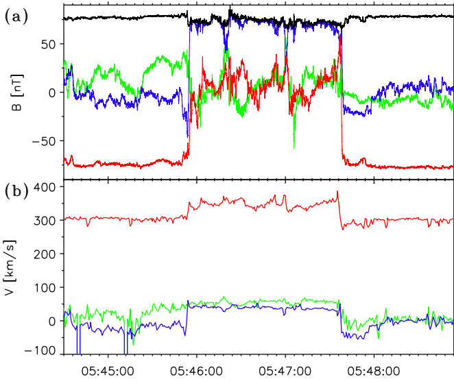
Fig. 1. Switchback observations from the Parker Solar Probe. From the PSP/FIELDS and PSP/SWEAP instruments on Nov. 5, 2018, measurements of the three components of the magnetic field and velocity in heliospheric R (red), T (green), N (blue) coordinates at a time close to the first perihelion of the mission around 35.7 R_{\odot} .
