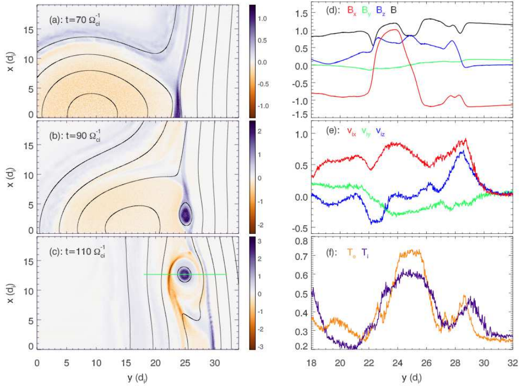
Fig. 3. Flux rope formation at three times during interchange reconnection near the solar surface. (a)–(c) Out-of-plane electron current J_{ez} with overlying magnetic field lines. Along the horizontal line in (c), in (d) the magnetic field components, B_x , B_y , B_z and B in red, green, blue and black, respectively, in (e) the corresponding ion velocities and in (f) the electron and ion temperatures.
