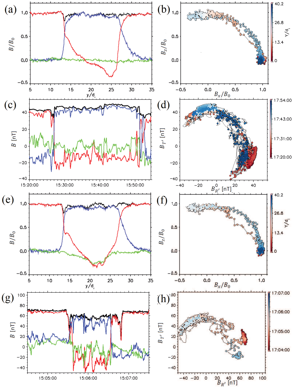
Fig. 5. (a) and (e): cuts of the magnetic fields ( B_x in red, B_y in green, B_z in blue and B in black) and associated hodograms in (b) and (f) across the large flux rope in Fig. 4. The cuts are along the white lines in (c). The cut in (a) corresponds to the midplane of the island where B_y \sim 0 while that in (e) is offset from the centerline where B_y < 0 . In (c) and (g) time profiles of magnetic fields ( B_{R'} in red, B_{N'} in green, B_{T'} in blue and B in black) and in (d) and (h) associated hodograms from switchbacks from PSP/FIELDS. The two events correspond to cases with the minimum variance magnetic field B_{N'} small (Nov. 1, 2018) (as in (a)) and negative (Nov. 4, 2018) (as in (e)). See the text for a discussion of the coordinate system used to present the spacecraft data. It differs from the traditional R, T, N system.
