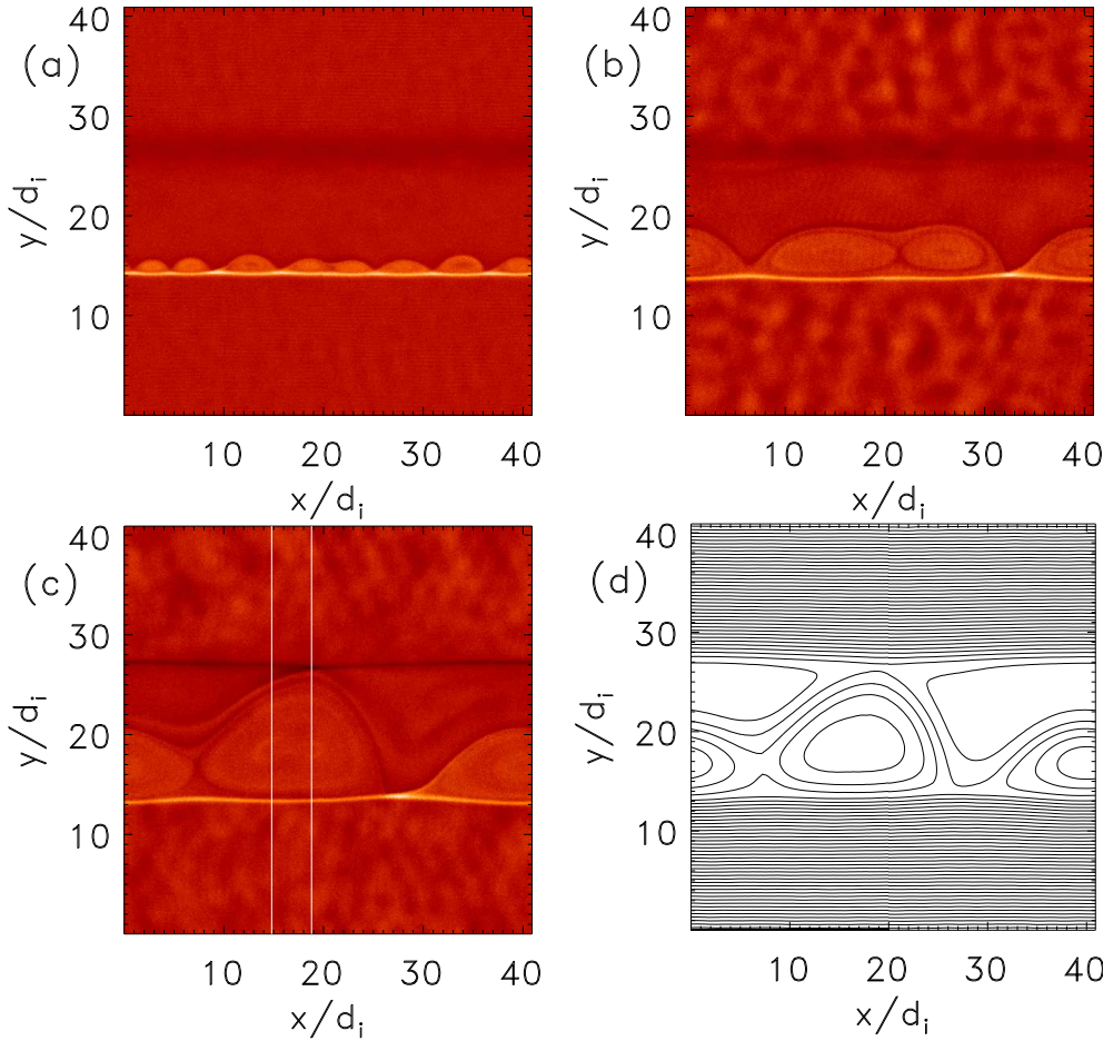
Fig. 4. Formation of the fluxrope within the ambient solar-wind magnetic field at \Omega_i t = 36 in (a), 180 in (b) and 292 in (c). Shown is the out-of-plane current J_{ey} . (d) Magnetic field lines for the time in (c). The large flux rope in (d) has reconnected all of the initial reversed magnetic field B_x and has the topology of the schematic in Fig. 2.
