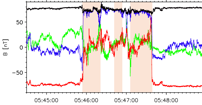
Fig. 6. Same magnetic field data as in Fig. 1. The shaded regions mark the possible locations of three flux ropes embedded within a large switchback.
