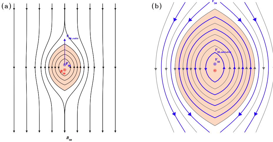
Fig. 2. (a) Schematic of a flux rope with a magnetic field that wraps a core axial field. The flux rope is propagating outward within a solar wind magnetic field pointing back towards the sun. As indicated, the flux rope generally has axial flow. (b) Schematic of the relaxed state of the flux rope in which the flow within the flux rope is field aligned.
