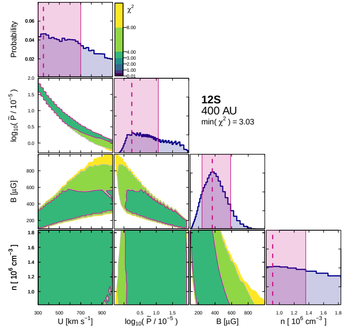
Fig. 4. Corner plot of the \chi^2 surface as a function of the model parameters for the VLA source 12S. The figure is organised as in Fig. 2.
