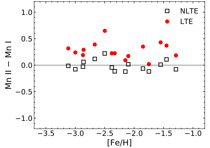
Fig. 1. Differences between abundances derived from Mn I and Mn II line for the metal-poor Galactic stars, for which UV spectra are available and robust Mn II measurements could be derived.
