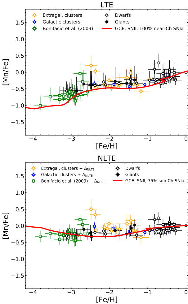
Fig. 2. Manganese abundance ratios as a function of metallicity. Top panel: LTE data presented with different symbols; the line shows the results of the GCE model with yield for SNe II taken from Woosley & Weaver (1995) , including only near- M_{\text{ch}} SNe Ia with by Iwamoto et al. (1999) . Bottom panel: NLTE data. The GCE model presented here adopts the yields by Kobayashi et al. (2011) for SNe II and includes 25% of near- M_{\text{ch}} and 75% of sub- M_{\text{ch}} SNe Ia.
