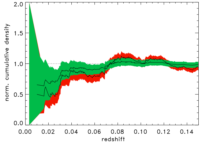
Fig. 10. Cumulative density distribution of NORAS II clusters as a function of redshift normalised to the mean for a lower X-ray luminosity limit of L_{X_0} = 5 \cdot 10^{42} \text{ erg s}^{-1} (lower curve with red uncertainty limits). The upper curve with green uncertainty limits shows the inferred dark matter distribution after correcting for the cluster bias.
