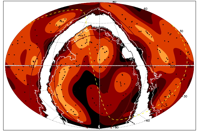
Fig. 7. Sky distribution of the clusters and their surface density in the CLASSIX survey with the extension into the zone of avoidance in equatorial coordinates. The survey is bounded by an interstellar hydrogen column density limit of n_{\text{H I}} < 2.5 \times 10^{21} cm ^{-2} . The white contours show the hydrogen column density boundary of n_{\text{H I}} = 1.5 \times 10^{21} cm ^{-2} . The red lines indicate the Galactic latitudes of l_{\text{H I}} = 20^\circ . The yellow dashed line marks the Supergalactic plane and the colour coding is the same as in Fig. 4.
