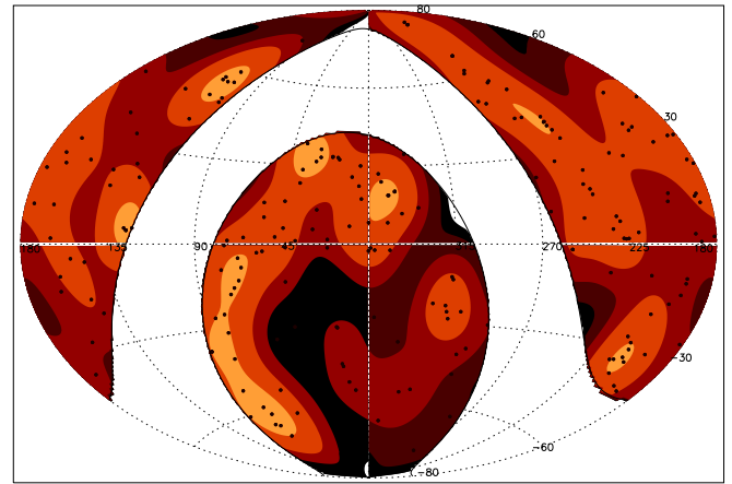
Fig. 4. Sky distribution of the clusters (black dots) and their surface density in the CLASSIX survey \Omega_{\text{M}} = 0.3 smoothed with a Gaussian filter with \sigma = 10 in the redshift slice z = 0 \pm 0.04 in equatorial coordinates. The colour coding for the density normalised to the mean is orange: >2 , red: 1.2 , brown: 0.5 , and dark brown/black: <0.5 .
