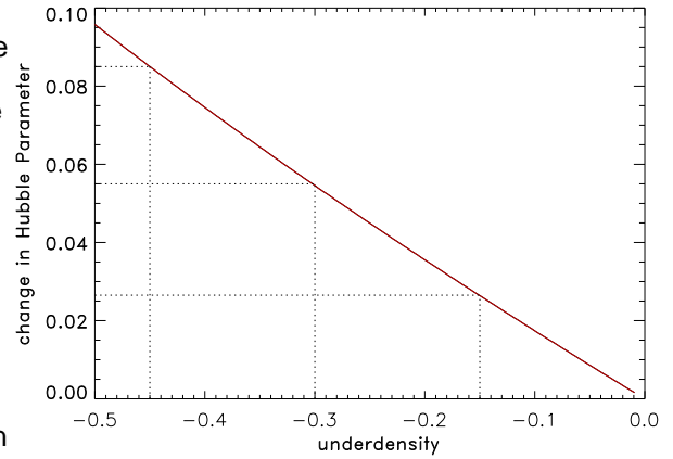
Fig. C.1. Change of the Hubble parameter as a function of the underdensity of the region studied. The dotted lines mark the underdensity values of 30% and 15%.
