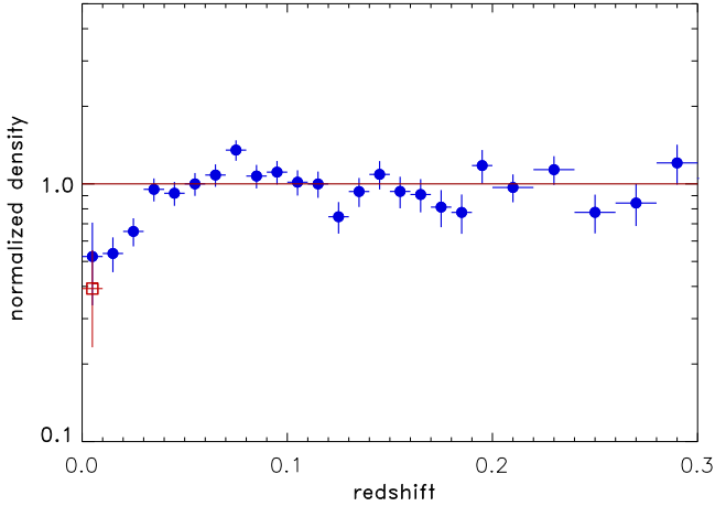
Fig. 1. Cluster density distribution as a function of redshift for the CLASSIX galaxy clusters covering the sky by \Omega_{\text{M}} = 0.3 for a minimum luminosity of 10^{42} \text{ erg s}^{-1} (0.1–2.4 keV). The density distribution plot has been normalised by the expected cluster density based on the same local density deficit. The open square shows the result if the region of the Virgo cluster is excluded from the analysis.
