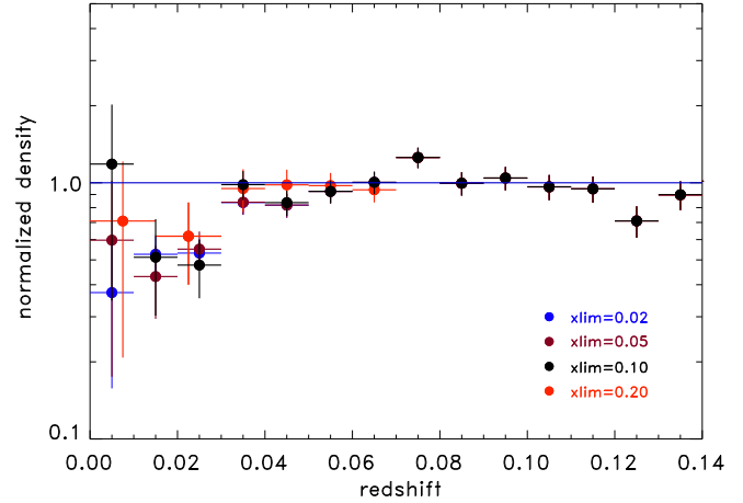
Fig. 3. CLASSIX galaxy cluster density distribution as a function of redshift for four different lower X-ray luminosity limits, given in the parameter x_{\text{lim}} in units of 10^{44} \text{ erg s}^{-1} . All samples trace the same local density deficit.
