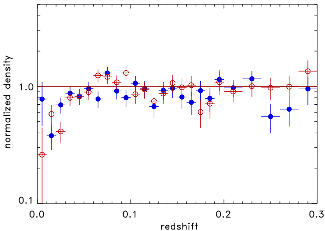
Fig. 6. Cluster density distribution as a function of redshift in the northern Galactic cap (filled blue circles) and southern Galactic cap (open red circles) at |b_{\text{H I}}| < 20^\circ , for a minimum luminosity of 10^{42} erg s ^{-1} (0.1–2.4 keV). The density distribution has been normalised by the expected cluster density based on the average luminosity function as explained in Sect. 3.
