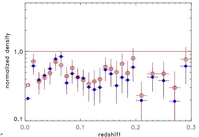
Fig. 8. Cluster density distribution as a function of redshift in the zone of avoidance at |b_{\text{H I}}| < 20^\circ . Filled symbols are for the region with a Galactic hydrogen column density of n_{\text{H I}} < 2.5 \times 10^{21} cm ^{-2} and open symbols for n_{\text{H I}} < 1.5 \times 10^{21} cm ^{-2} . The cluster sample in this region is not complete and therefore the data provide a lower limit. The density distribution has been normalised by the expected cluster density based on the average luminosity function as explained in Sect. 3.
