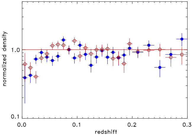
Fig. 5. Cluster density distribution as a function of redshift for the REFLEX II survey in the southern sky (open red circles) and the NORAS II survey in the north (filled blue circles) at l_{\text{H I}} < 20^\circ , for a minimum luminosity of 10^{42} erg s ^{-1} (0.1–2.4 keV). The density distribution has been normalised by the expected cluster density based on the average luminosity function as explained in Sect. 3.
