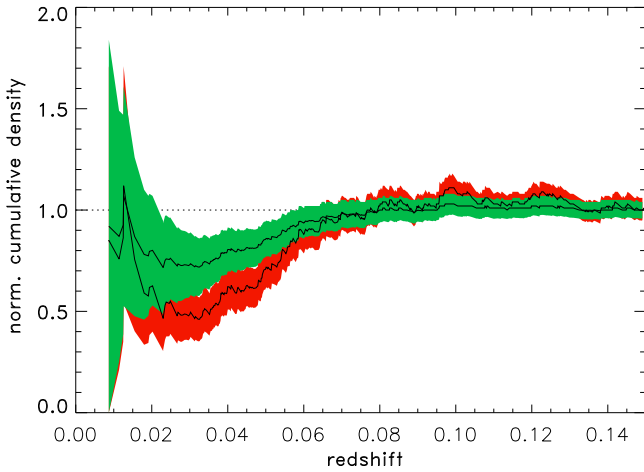
Fig. 9. Cumulative density distribution of REFLEX II clusters as a function of redshift normalised to the mean for a lower X-ray luminosity limit of L_{X_0} = 5 \cdot 10^{42} \text{ erg s}^{-1} (lower curve with red uncertainty limits). The upper curve with green uncertainty limits shows the inferred dark matter distribution after correcting for the cluster bias.
