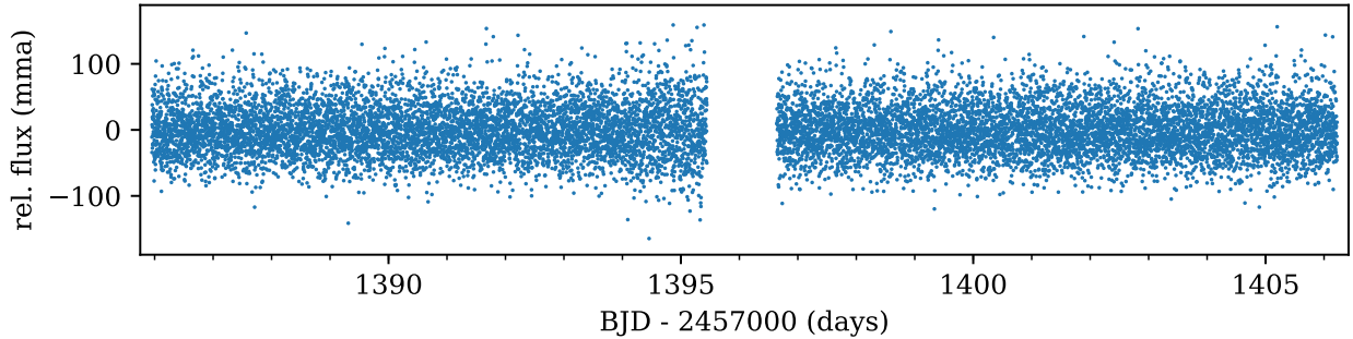
Fig. 1. Final reduced TESS Sector 3 light curve of TIC 257459955. A gap occurs at spacecraft perigee.
