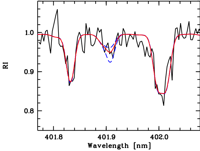
Fig. 3. Observed spectrum (solid black) in the range of the 401.9 nm Th II line, compared with the best fit (solid red) providing A(\text{Th}) = 0.12 , and two synthetic spectra at A(\text{Th}) of -0.3 and 0.5 (dashed blue). The Th II line is blended with a ^{13}\text{C} H line, which is taken into account.
