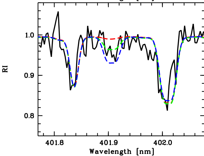
Fig. 4. Top panel: observed spectrum (solid black) in the range of the G-band, compared with synthetic spectra with different ^{12}\text{C}/^{13}\text{C} ratios (dashed red 90; dashed green 7.5, the best fit; and dashed blue 3). Bottom panel: Th II line with the synthetic spectra of the top panel and with a solar scaled Th abundance.
