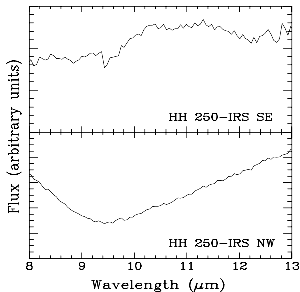
Fig. 1. Spectra of both components of HH 250-IRS binary in 8–13 \mu\text{m} region. The spectra are smoothed to the resolution \lambda/\Delta\lambda \approx 170 of the flux-calibrated spectrum of the telluric correction star (Cohen et al. 1999).
