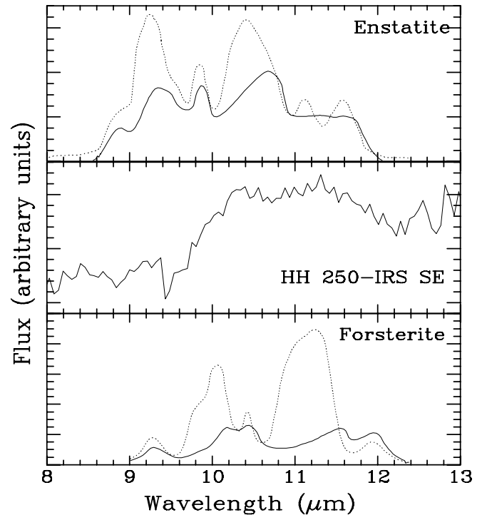
Fig. 2. Silicate feature of HH 250-IRS SE ( middle panel ) compared to spectra of enstatite ( top panel ) and forsterite ( bottom panel ). The spectra of crystalline silicates are adapted from van Boekel et al. (2005). To facilitate the comparison a constant level has been subtracted from the spectrum of HH 250-IRS SE. The solid and dotted curves in the spectra of both silicates correspond to grains of 1 and 0.1 \mu\text{m} , in size, respectively.
