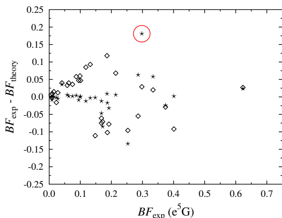
Fig. 5. Experimental branching fractions from 3d^3(^4F)4d\ e^5G compared with Kurucz (1995) ( \star ) and Kurucz (2013) ( \diamond ). The circled data is not calculated, but experimental values from Martin et al. (1988). See discussion in text.
