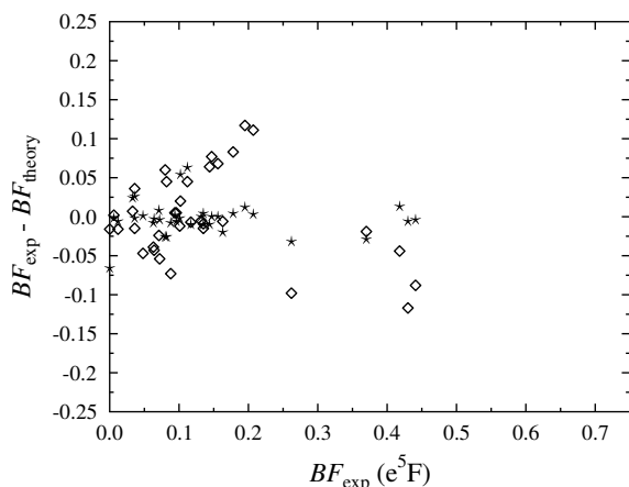
Fig. 4. Experimental branching fractions from 3d^3(^4F)4d\ ^5F compared with Kurucz (1995) ( \star ) and Kurucz (2013) ( \diamond ).
