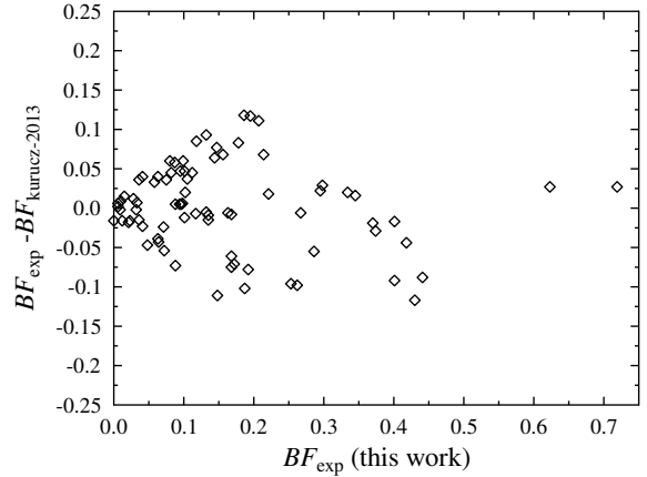
Fig. 3. All measured branching fractions for the 4p-4d transitions in V II compared with Kurucz (2013).
