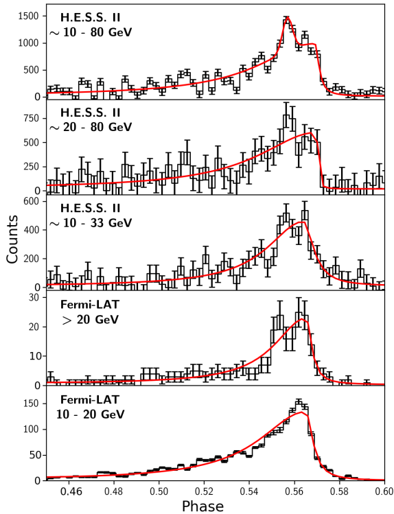
Fig. 3. \gamma -Ray phasogram of the Vela pulsar around P2 in the phase range [0.45, 0.6], in different energy bands from 10 to 80 GeV, as obtained from the Fermi -LAT and H.E.S.S. II data. The red curve represents the asymmetric Lorentzian form fitted to data, except for the top-most panel where an additional Gaussian component is included in the fit to the H.E.S.S. II full energy range light curve (see Table 2). The background has been subtracted for the H.E.S.S. II light curves. The bin width for all histograms is 0.25 ms.
