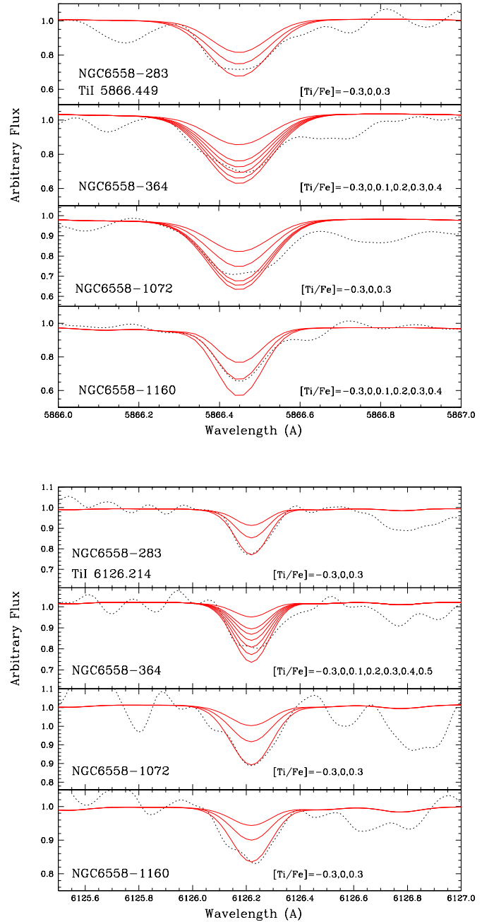
Fig. 4. Ti I 5866.449 and 6126.214 Å lines in the four sample stars. Calculations for different [\text{Ti}/\text{Fe}] are shown, with values as indicated in each panel.
