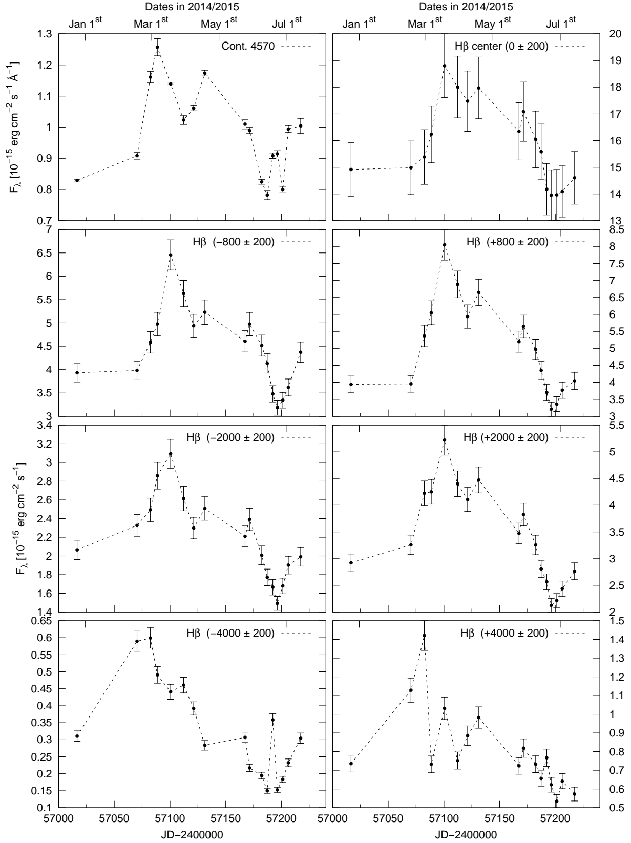
Fig. A.2. Light curves of the continuum flux at 4570 Å and of selected H \beta line segments (in units of 10^{-15} erg \text{s}^{-1} \text{cm}^{-2} ): H \beta center and segments at v = \pm 800, \pm 2000, \pm 4000 km \text{s}^{-1} .
