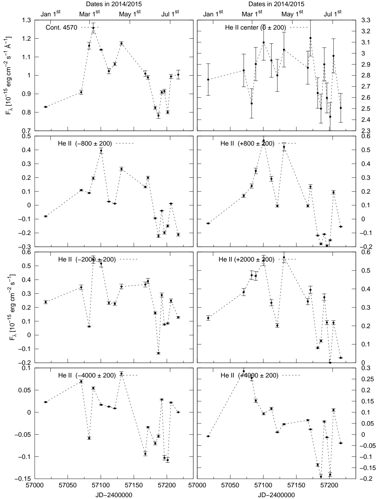
Fig. A.4. Light curves of the continuum flux at 4570 \text{ \AA} and of selected He II \lambda 4686 line segments (in units of 10^{-15} \text{ erg s}^{-1} \text{ cm}^{-2} ): He II \lambda 4686_{\text{center}} and segments at v = \pm 800, \pm 2000, \pm 4000 \text{ km s}^{-1} .
