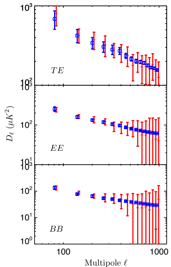
Fig. 8. High-resolution power spectra on the LR63 region; simulation vs. data. From top to bottom: TE, EE, and BB power spectra of the Planck 353 GHz, CMB-corrected maps (red crosses), and one high-resolution ( N_{\text{side}} = 2048 , FWHM = 10' ) realization of the model (blue squares).
