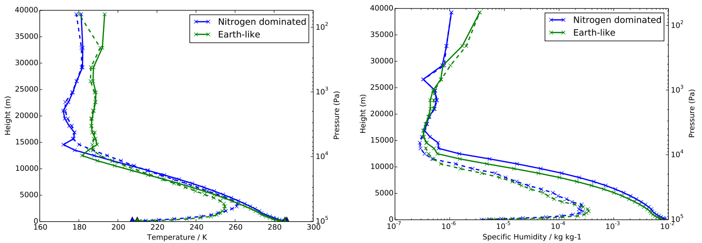
Fig. 5. Ten orbit mean profiles of temperature and water vapour ( left and right panels , respectively) from the sub-stellar point on the dayside of the tidally locked planet (solid) and its antipode (dashed). Filled triangles show the surface temperature, and crosses indicate the position of the model levels.
