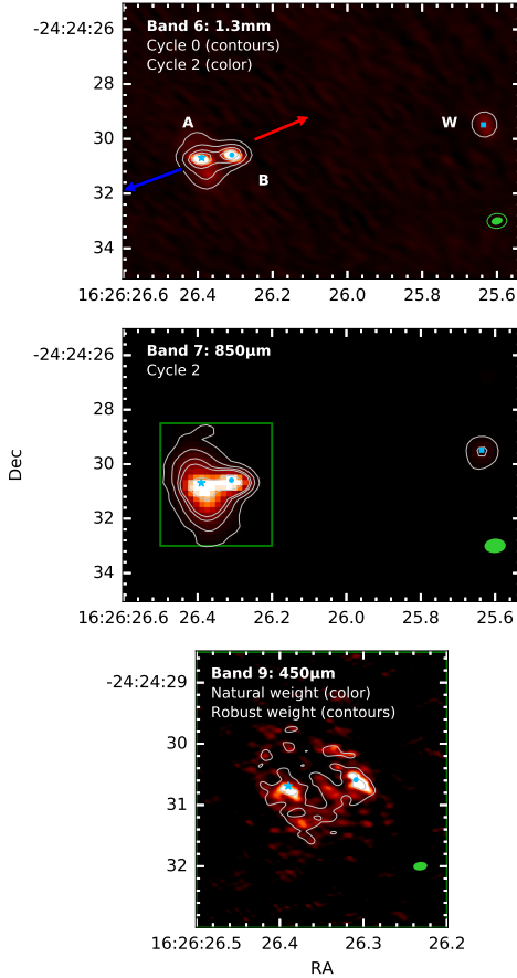
Fig. 1. VLA 1623 observed with ALMA. The phase center for all observations is similar and located around the position of VLA 1623 A. Contours are in steps of 3, 8, 15, 20, 50 \sigma ; \sigma is listed in Table 1. The green ellipses show the beam size of the observations. The green box in the middle panel outlines the area of the Band 9 observations presented in the bottom panel.
