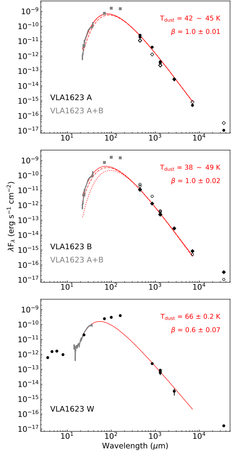
Fig. 2. Spectral energy distribution of VLA 1623 including the Spitzer IRS spectra. The red curves show the best fit graybody to each SED. The dust temperature T_{\text{dust}} and dust emissivity index \beta are indicated in each panel. For VLA 1623 A (top) and B (middle), the dashed curves show the best fit assuming that the emission at \lambda < 450\mu\text{m} is evenly distributed among the two sources. The dotted curve assumes VLA 1623 B only contributes one-tenth of the total emission for \lambda < 450\mu\text{m} . The open symbols in the top and middle panel are the fluxes for VLA 1623 B and VLA 1623 A, respectively, and are included for ease of comparison.
