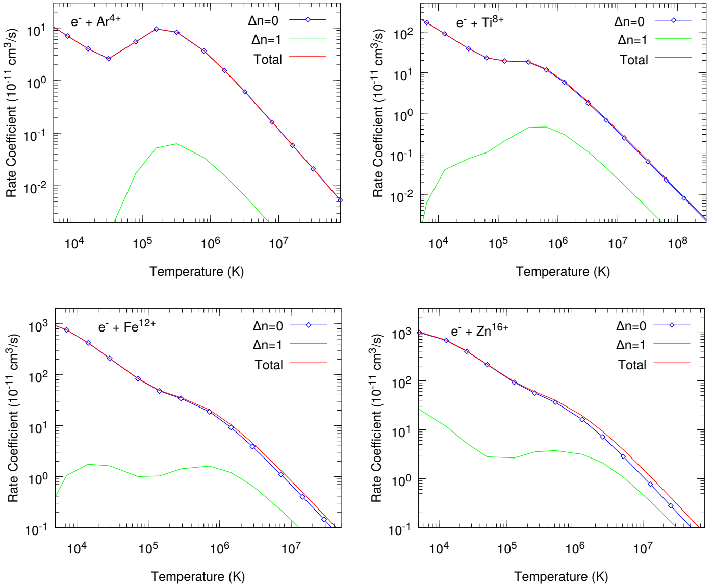
Fig. 6. Total Maxwellian-averaged ground-level DR rate coefficients and the separate contributions from \Delta n_c = 0 and \Delta n_c = 1 core excitations for Ar 4+ , Ti 8+ , Fe 12+ , and Zn 16+ ions.
