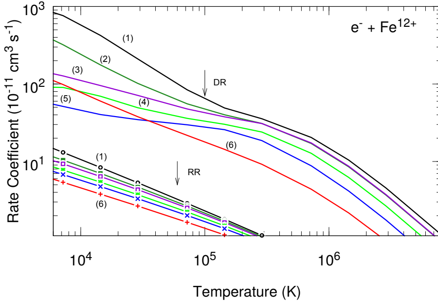
Fig. 5. Total Maxwellian-averaged DR and RR rate coefficients from the ground ( 3s^23p^2\ ^3P_0 ) ( i = 1 ) and metastable initial levels ( 3s^23p^2\ (^3P_{1,2}, ^1D_2, ^1S_0) ) ( i = 2-5 ) and 3s^23p3d\ (^5S_2) ( i = 6 ) of \text{Fe}^{12+} .
